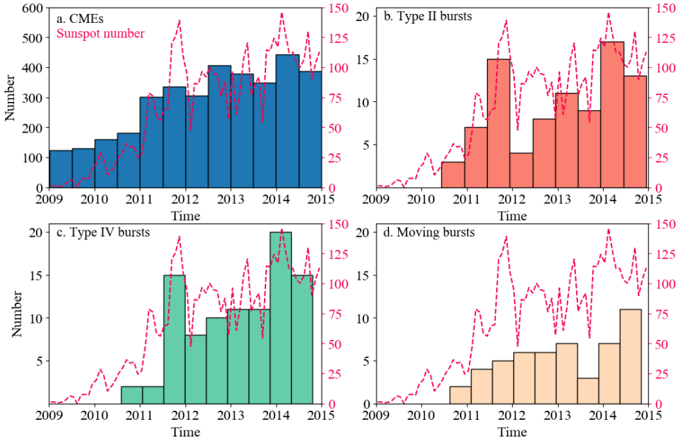
Fig. 2. Histograms showing the (a) occurrence of CMEs, (b) type II bursts, (c) type IV bursts, and (d) and moving radio bursts during the observational windows of the NRH in SC24. Overlaid on each panel in pink are the monthly average sunspot numbers during the time period shown.
