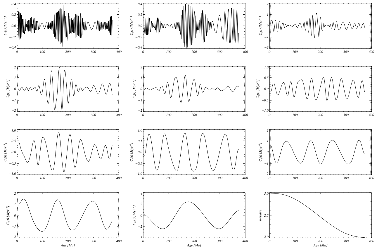
Figure 2. IMFs obtained through the EMD technique applied to the reversal rate time series. The residue of the decomposition is shown in the lowest right panel, while the IMFs C_j(t) , for j=0,1,\dots,10 , are reported in the other panels.
