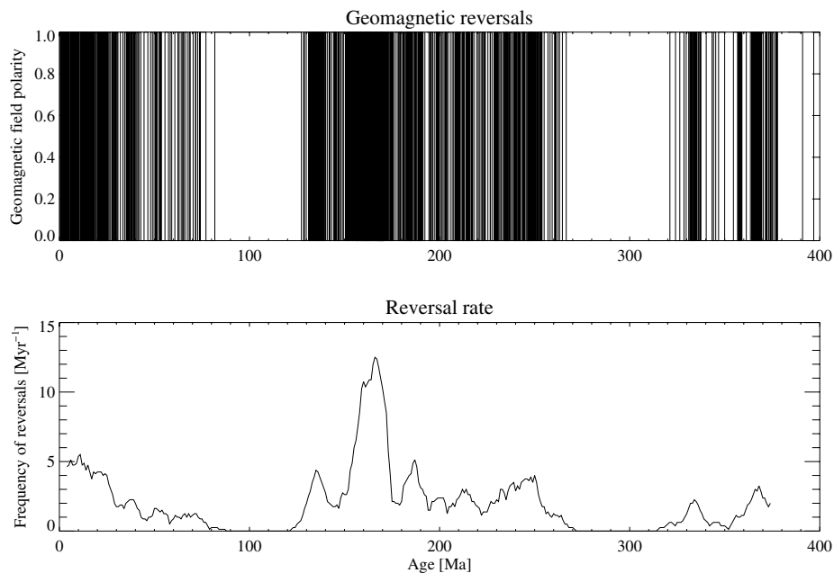
Figure 1. Upper panel: geomagnetic polarity back to 375.3 Ma. The polarity is denoted by 1 for the present polarity and 0 for reversed. A line connects the values, therefore black regions correspond to a high reversal rate and white regions to intervals of constant value. Lower panel: reversal rate time series obtained by averaging over sliding windows of length \Delta t = 8 Myr (see Supplementary Information).
