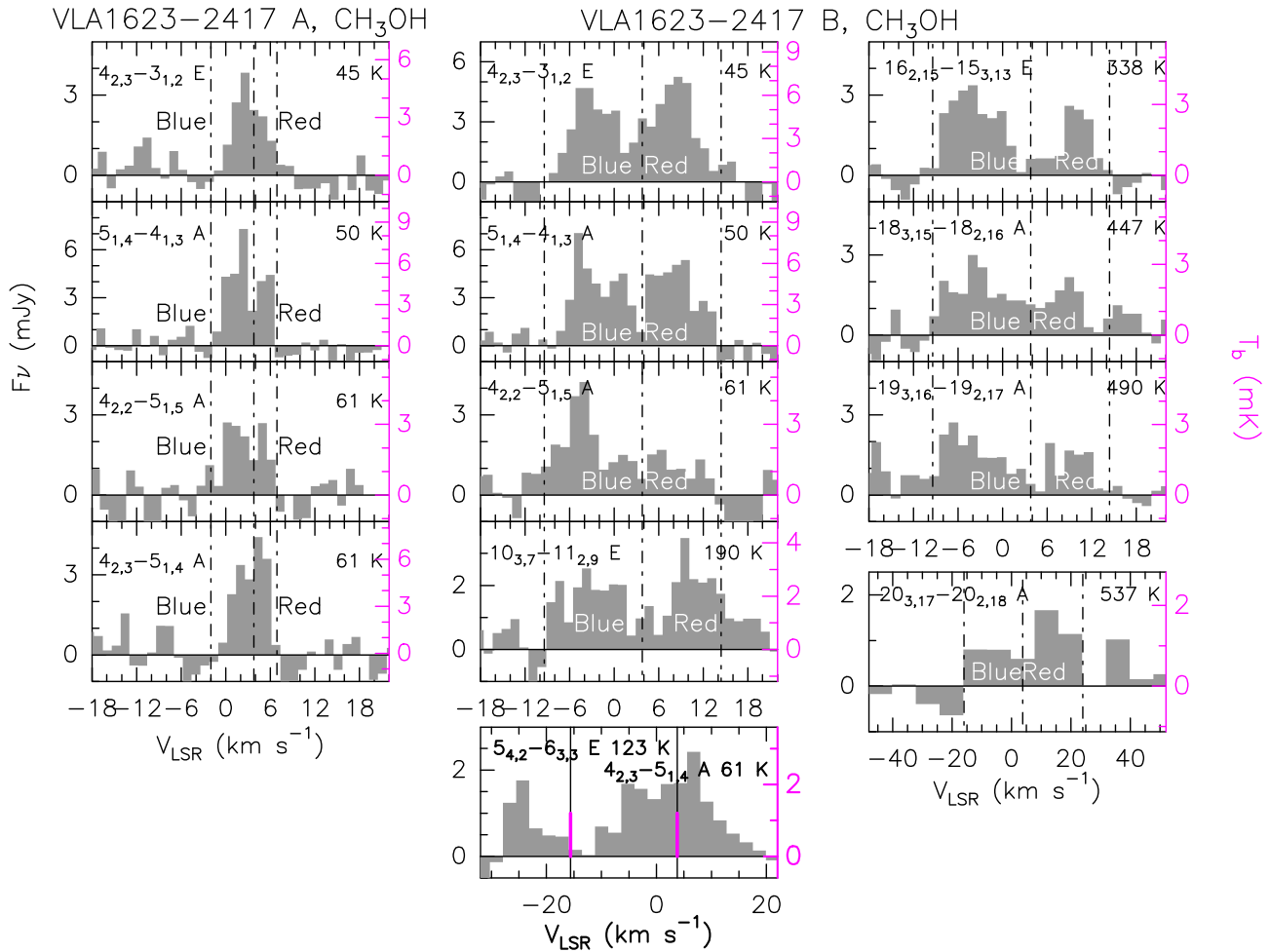
Figure 3. Observed \text{CH}_3\text{OH} line spectra (in both F_\nu and T_B scales) at the positions of the VLA1623 A binary protostar (left-hand panels) and B protostar (middle and right-hand panels). Transitions and upper level energies are reported. The vertical dashed lines mark: the systemic local standard of rest (LSR) velocity ( +3.8 \text{ km s}^{-1} ; Narayanan & Logan 2006), as well as the velocity ranges of the red- and blueshifted emission used to derive velocity integrated maps (see Table 1 and Fig. 2) and maps of the blue- and redshifted emissions (see Fig. 7). Note that the 4_{2,3}-5_{1,4} A and 5_{4,2}-6_{3,3} spectra towards B (smoothed to a spectral resolution of 2.4 \text{ km s}^{-1} to increase the S/N) are blended: The continuous black and magenta lines show the differences between their rest frequencies (in the velocity scale).
