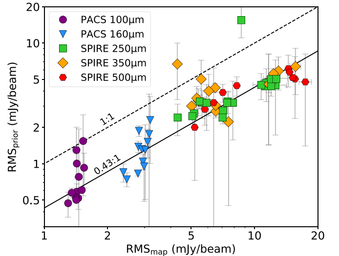
Figure 4. The rms noise of Herschel images measured from the prior-based catalogs ( \text{RMS}_{\text{prior}} ; see Section 3.3) vs. the 2D uncertainty maps ( \text{RMS}_{\text{map}} ). Measurements obtained on the maps from 100 to 500\,\mu\text{m} are shown as symbols with different colors as labeled in the upper left legend. The dashed line indicates the case in which the two rms noises are identical, and the solid line represents the median ratio of \text{RMS}_{\text{prior}} to \text{RMS}_{\text{map}} of 0.43 \pm 0.01 .
