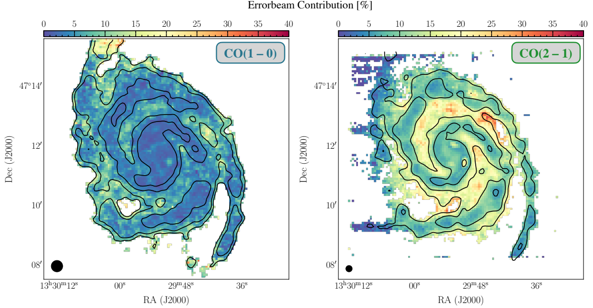
Fig. A.4. 2D distribution of the error beam contribution. ( Left ) ^{12}\text{CO}(1-0) map. Contours are drawn at S/N = 10, 20, 30 of \text{CO}(1-0) emission. ( Right ) ^{12}\text{CO}(2-1) map. We see that the error beam contribution is more pronounced for \text{CO}(2-1) , in particular in the interarm regions of the galaxy.
