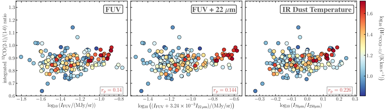
Fig. 15. ^{12}\text{CO}(2-1)/(1-0) line ratio compared to FUV intensity (left), FUV+22 \mu\text{m} (centre), and infrared colour (right). We only include sight lines with S/N > 5 for the line ratio to minimise scatter from faint ^{12}\text{CO} lines. We use a working resolution of 27 arcsec. FUV emission follows to some extent young ( \leq 100 Myr) stellar populations. Because FUV can be heavily obscured, we correct using 22 \mu\text{m} data from WISE band-4 observations. To combine FUV and 22 \mu\text{m} , we multiply the 22 \mu\text{m} by a factor 3\text{--}24 \times 10^{-3} . The resulting sum is proportional to the SFR surface density (Leroy et al. 2019). The infrared 70 \mu\text{m}/250 \mu\text{m} colour is a proxy for the dust temperature. We provide the Pearson’s linear correlation coefficient, r_p , in each panel. We do not find any evident correlation of the line ratio with either quantity.
