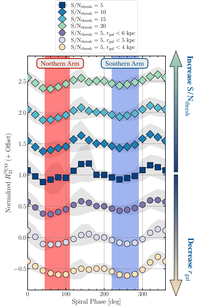
Fig. 14. Spiral arm–interarm CO line ratio variation consistency. For the arm–interarm variation in Fig. 12, we include all sight lines with S/N > 5 . Here, we increase the S/N threshold from 5 to 20 in steps of 5 to investigate whether the higher line ratios are still preserved in the interarm region. Furthermore, we add a radial constraint, only including sight lines within a given galactocentric radius of 4, 5, and 6 kpc. We normalise the line ratios by the global CO (2–1) brightness weighted median. We offset different line ratios in steps of 0.5 (in the positive direction for increasing S/N and in negative steps for decreasing radial constraint). We see that the trend of higher line ratios in the interarm region is persistent for all computations shown in this figure.
