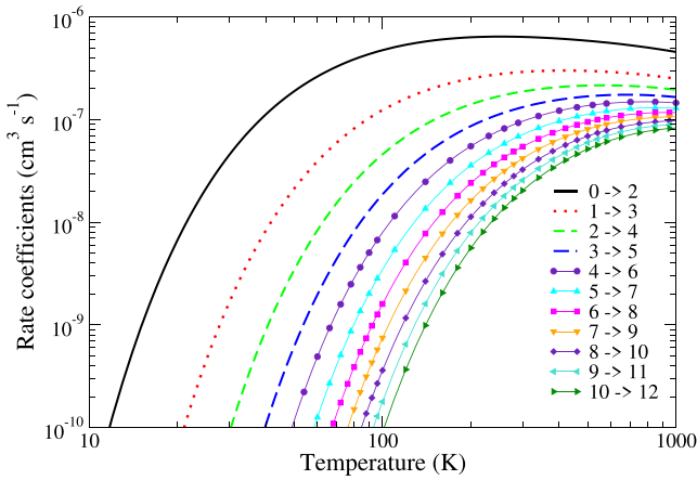
Figure 2. Maxwell rate coefficients for the RE N_i^+ \rightarrow N_f^+ = N_i^+ + 2 , with N_i^+ = 0 to 10 of the vibrationally relaxed ( v_i^+ = 0 ) D_2^+ ( X^2\Sigma_g^+ ).
