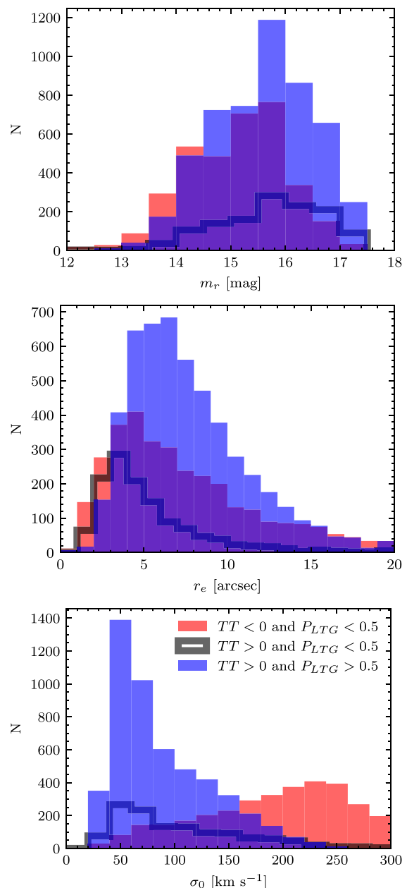
Figure 6. Galaxies having inconsistent T-Type and P_{\text{LTG}} classifications (open histograms) tend to be faint (top), have small angular sizes (middle), and small central velocity dispersions (bottom).
