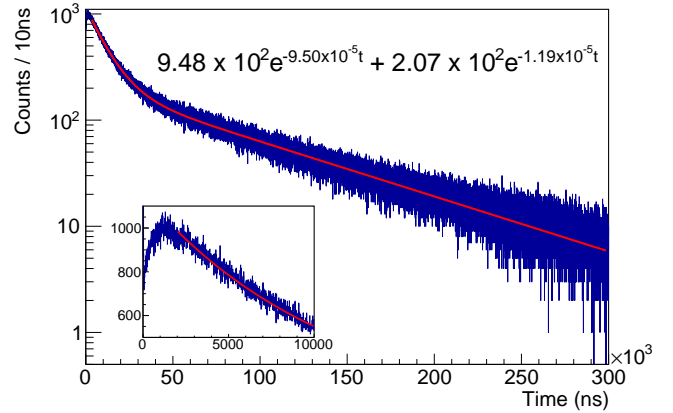
FIG. 7. Evolution of the neutron detection for the neutron spectrum displayed in Fig. 3, over the first 300 \mu\text{s} . Inset: Zoom-in over the first 10 \mu\text{s} , showing that the signal peaks around 1.2 \mu\text{s} . The axes of the inset represent the same values, in the same units, as the main graph.
