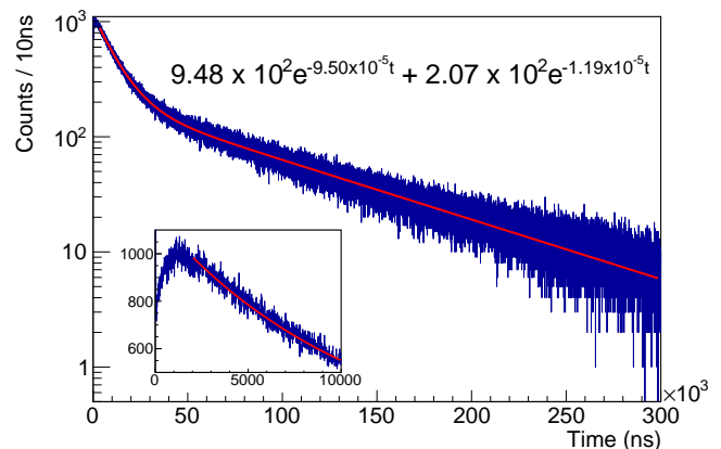
FIG. 7. Evolution of the neutron detection for the neutron spectrum displayed in Fig. 3, over the first 300 \mu\text{s} . Inset: Zoom-in over the first 10 \mu\text{s} , showing that the signal peaks around 1.2 \mu\text{s} . The axes of the inset represent the same values, in the same units, as the main graph.
