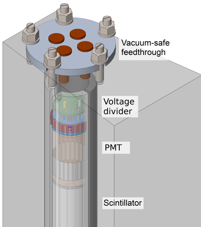
FIG. 12. Close up view of one of the final detector modules, showing the top part of the module with the end of the scintillator rod, the PMT and the voltage divider, and the arrangement for the vacuum sealing of the unit with the four LEMO feed-throughs connecting the signal and high-voltage cables to the top and bottom PMT.
