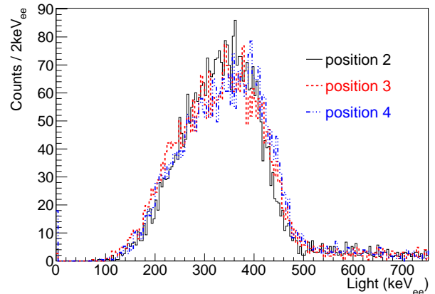
FIG. 16. Histogram of the light collected by the detector unit when summing the energy measured by both PMTs for 3 different positions of the directive gamma source described in Fig. 15, and recalibrating the photon energy against the know Compton edge (477.34 keV). As one could expect, those spectra are identical.
