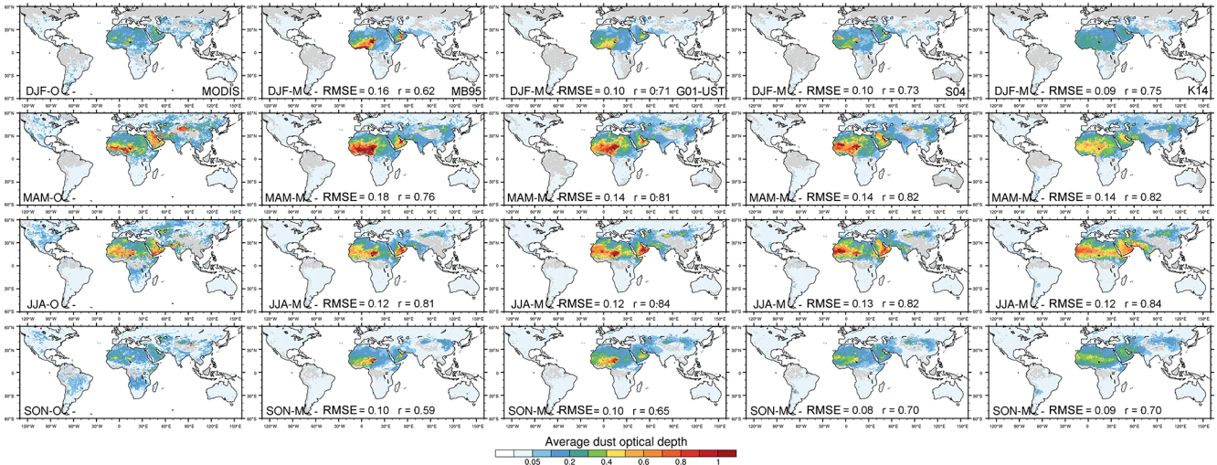
Figure B1. Seasonally averaged MODIS Deep Blue DOD (left) and MONARCH all-sky \text{DOD}_{\text{coarse}} at satellite overpass times co-located with MODIS DOD for the MB95, G01-UST, S04, and K14 runs. The seasonal averages were calculated with respect to the number of valid values per grid cell in the MODIS product. Area-weighted RMSE and uncentered Pearson product-moment coefficient of linear correlation ( r ) are indicated in the respective panels.
