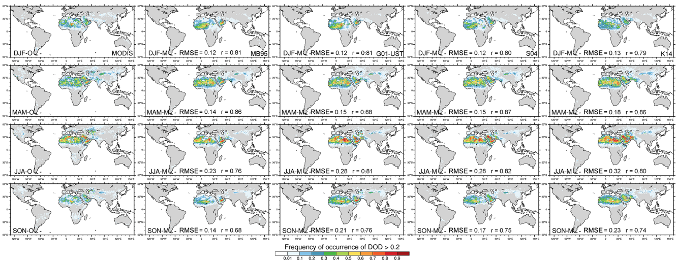
Figure B2. Seasonally averaged FoO of \text{DOD} > 0.2 , normalized by the number of days per season for MODIS Deep Blue (left) and MONARCH all-sky \text{DOD}_{\text{coarse}} at satellite overpass times co-located with MODIS DOD for the MB95, G01-UST, S04, and K14 runs. The FoO was calculated with respect to the number of days in the season. Area-weighted RMSE and uncentered Pearson product-moment coefficient of linear correlation ( r ) are indicated in the respective panels.
