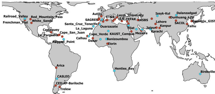
Figure C1. AERONET stations (direct-Sun V3 level 2.0) available in 2012. The station subset used for comparison with MONARCH are shown in turquoise, whereas all other stations are marked in red.
