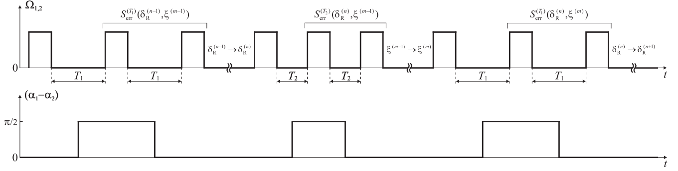
FIG. 3. Scheme of the GABRS-CPT sequence, where n and m are the step indices for the first and second servo loops, respectively.
