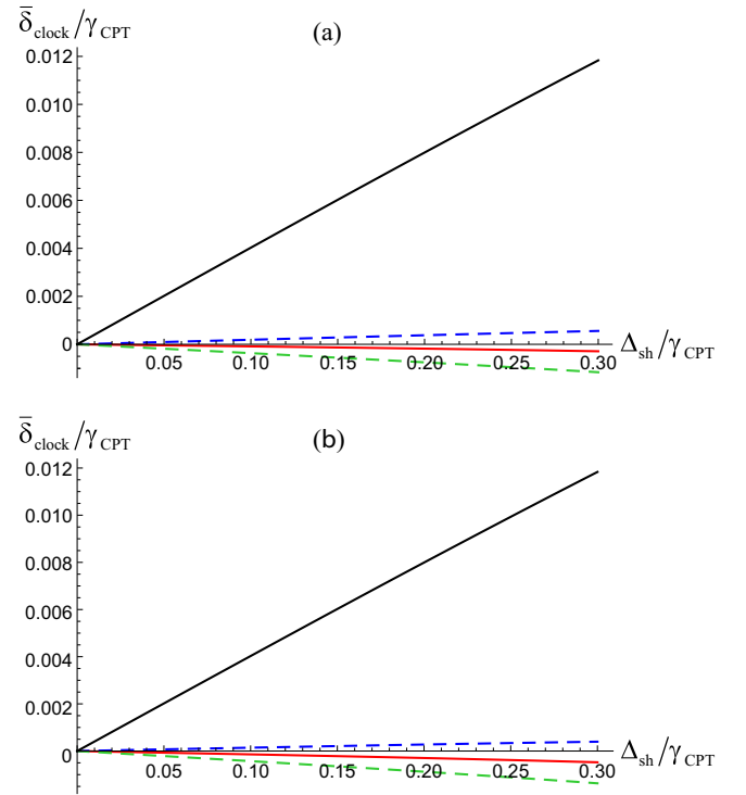
FIG. 10. Shift of the clock frequency \bar{\delta}_{\text{clock}} versus the light shift \Delta_{\text{sh}} for MCESRS: (a) detecting pulses of the equal durations; (b) detecting pulses of the different durations. The black solid line is calculated for the usual Ramsey scheme ( T = 0.5 \Gamma^{-1} ), the red solid line is calculated for the MCESRS ( T_L = 0.5 \Gamma^{-1} and T_S = 0.05 \Gamma^{-1} ) in the case of the ideal value (B2) of the calibration coefficient \beta_{\text{cal}} , the green dashed line is calculated for the MCESRS if \beta_{\text{cal}} deviates by +5% from the ideal value, and the blue dashed line is calculated for the MCESRS if \beta_{\text{cal}} deviates by -5% from the ideal value. Numerical parameters of the model are as follows: \Omega_1 = \Omega_2 = 0.25 \gamma_{\text{sp}} , \gamma_1 = \gamma_2 = \gamma_{\text{sp}}/2 , \gamma_{\text{opt}} = 50 \gamma_{\text{sp}} , \Gamma = 5 \times 10^{-5} \gamma_{\text{sp}} , \tau_p = \infty (steady state), \tau_d = \tau_s = 0.15 \gamma_{\text{CPT}}^{-1} , and \alpha_r^\pm = \pm \pi/2 .
