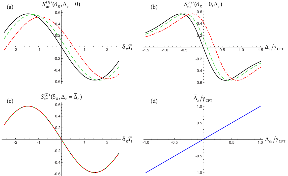
FIG. 6. (a) Error signal S_{\text{err}}^{(T_1)}(\delta_R, \Delta_c = 0) in the standard Ramsey scheme. (b) Error signal S_{\text{err}}^{(T_2)}(\delta_R = 0, \Delta_c) for stabilization of the additional frequency jump. (c) Error signal S_{\text{err}}^{(T_1)}(\delta_R, \Delta_c = \bar{\Delta}_c) for stabilization of the LO frequencies in the autobalanced Ramsey scheme with the additional frequency jump. (d) Dependence of the frequency jump \bar{\Delta}_c on the frequency shift of the clock transition \Delta_{\text{sh}} . The graphs (a)–(c) are calculated for the following values of the light shift of the Raman transition: \Delta_{\text{sh}}/\gamma_{\text{CPT}} = 0 (black solid line), \Delta_{\text{sh}}/\gamma_{\text{CPT}} = 0.1 (green dashed line), and \Delta_{\text{sh}}/\gamma_{\text{CPT}} = 0.3 (red dot-and-dash line). Numerical parameters of the model are as follows: \Omega_1 = \Omega_2 = 0.25 \gamma_{\text{sp}} , \gamma_1 = \gamma_2 = \gamma_{\text{sp}}/2 , \gamma_{\text{opt}} = 50 \gamma_{\text{sp}} , \Gamma = 5 \times 10^{-5} \gamma_{\text{sp}} , T_1 = 0.5 \Gamma^{-1} , T_2 = 0.1 \Gamma^{-1} , \tau_p = \infty (steady state), \tau_d = 5 \gamma_{\text{CPT}}^{-1} , and \alpha_r^\pm = \pm\pi/2 .
