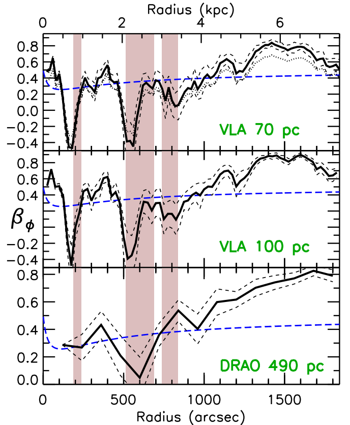
Fig. 6. Profiles of azimuthal velocity anisotropy \beta_\phi of the atomic gas in M 33 at different angular resolutions. Solid lines show the anisotropy profiles obtained assuming \sigma_z = \langle \sigma_{\text{los}} \rangle_\phi and a null thermal component. Short-dashed lines show the \pm 1 rms errors; a dotted line is an illustration of result choosing another vertical dispersion, \sigma_z = 4 \text{ km s}^{-1} (70 pc resolution only); and a blue long-dashed line is the velocity anisotropy profile expected from the epicycle theory (Sect. 5). Shaded areas are as in Fig. 4.
