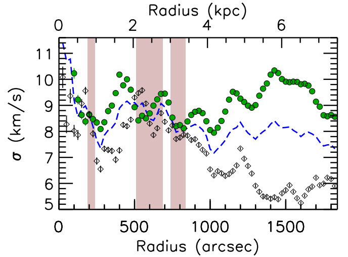
Fig. 4. Results of the anisotropic and axisymmetric velocity model for the atomic gas in Messier 33 (100 pc resolution data). Results are those of the one-parameter model and show the profile of \sigma_R ( \sigma_\phi , respectively) as filled green circles (open diamonds), obtained assuming \sigma_\phi = \sigma_z = \langle \sigma_{\text{los}} \rangle_\phi ( \sigma_R = \sigma_z = \langle \sigma_{\text{los}} \rangle_\phi ). A dashed blue line is for \langle \sigma_{\text{los}} \rangle_\phi (corrected from instrumental dispersion). Results obtained assuming a null thermal component. The shaded areas highlight the regions where the k = 2 mode was found to be weaker than other dispersion asymmetries (see Sect. 3).
