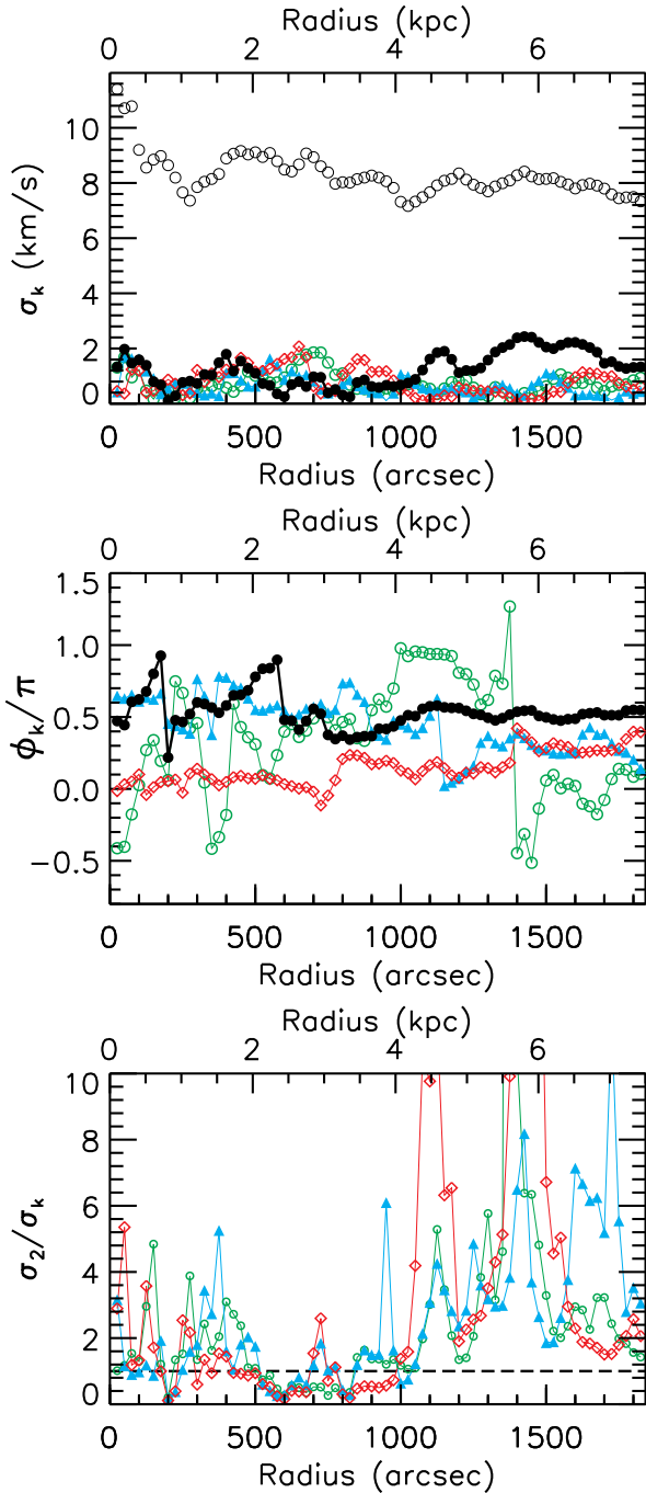
Fig. 3. Results of the discrete FFT of the HI velocity dispersion map of M33 (100 pc resolution, in the CNM case). The amplitudes ( upper panel ) and phases ( middle panel ) of the Fourier modes are shown as black open circles ( k = 0 ), green open circles ( k = 1 ), filled circles ( k = 2 ), blue upward filled triangles ( k = 3 ), and red open diamonds ( k = 4 ). The reference \phi = 0 is chosen along the semi-major axis of the NE approaching half of M33. Bottom panel : \sigma_2/\sigma_k , using the same colors and symbols as above for the k = 1, 3, 4 modes. The range of ratios is chosen up to 10 for clarity, but the total range is 78 for \sigma_2/\sigma_1 and \sigma_2/\sigma_4 , and 12 for \sigma_2/\sigma_3 .
