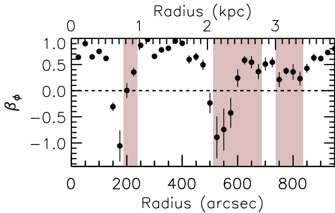
Fig. 8. Profile of azimuthal anisotropy \beta_\phi of the velocity dispersion of the atomic gas in M33 obtained using the 100 pc resolution VLA data by assuming \sigma_z = \langle \sigma_{\text{los}} \rangle_\phi and HI as a warm neutral medium (thermal component of 6 \text{ km s}^{-1} ). Shaded areas are as in Fig. 4.
