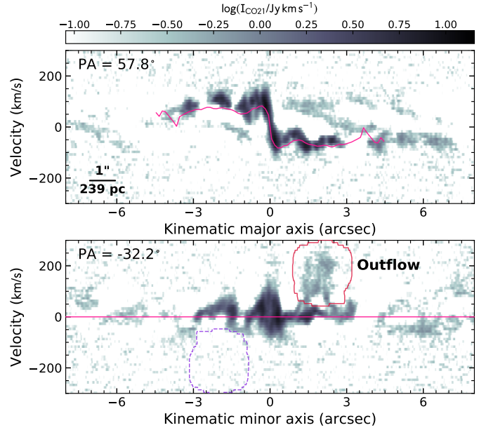
Fig. 4. Top: position-velocity diagram along the kinematic major axis (PA = 57^\circ.8 ). The magenta line indicates the best-fit circular rotation curve obtained with DISKFIT. Bottom: position-velocity diagram along the kinematic minor axis (PA = -32^\circ.2 ). The magenta horizontal line indicates the best-fit systemic velocity of the galaxy ( 3568 \pm 7 \text{ km s}^{-1} ). The solid red and dashed purple contours delineate the section of the 3D mask we used to integrate the outflow region and its symmetric region across the kinematic minor axis, respectively.
