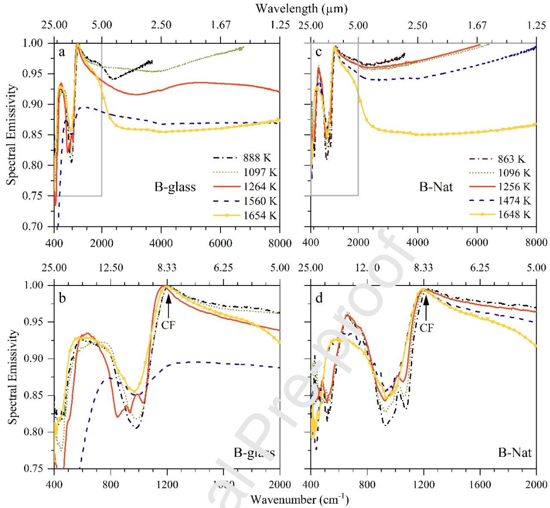
Figure 3: Spectral emissivity evolution with temperature and wavenumber for a,b) Bárðarbunga glass, and c,d) Bárðarbunga Natural (thickness: 1.5 mm, and 3.0 mm at ~1650 K). b), d) Zoom on TIR range (8–12 μm). Note the limited spectral range for the spectra recorded at lower temperature because of the insufficient radiation achieving detector. CF: Christiansen Feature.
