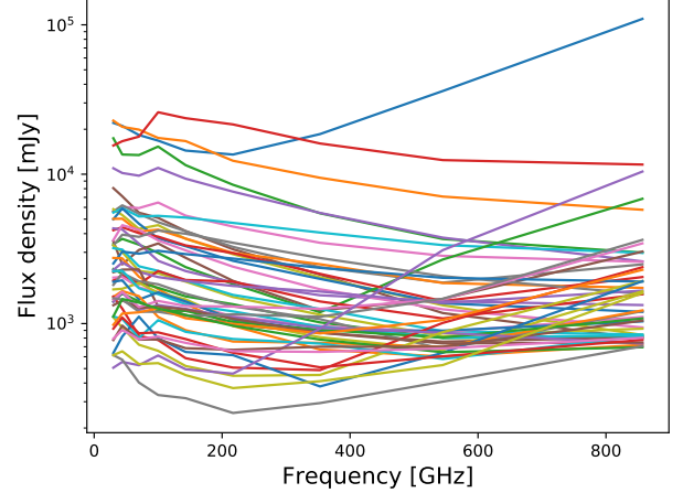
Fig. 7. Spectral energy distributions of the 49 PCNTb sources outside the Planck GAL070 mask that are identified as blazars in the BZCAT5 catalogue (Massaro et al. 2015).
