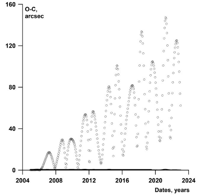
Figure 7. Comparison of our results with the JPL ephemerides for satellite S36 (Aegir). Observations made in 2019 are included. Empty circles are the differences between observations and positions obtained from the JPL ephemerides. The plot of precision estimates (line) merges with the x-axis. See also the notes relating to Fig. 1. The mean orbital period of this satellite is 1109 days (3.04 years).
