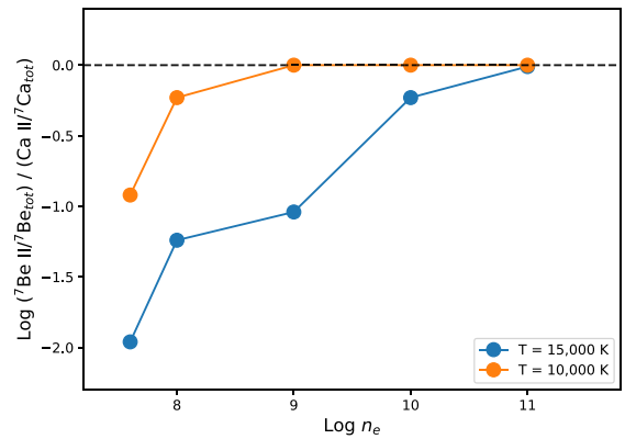
Figure 8. Relative mean ionization of {}^7\text{Be II} and Ca II, \log(\text{Be II}/\text{Be})/(\text{Ca II}/\text{Ca}) , for different values of gas densities and for two temperatures of the pseudo-photosphere.
