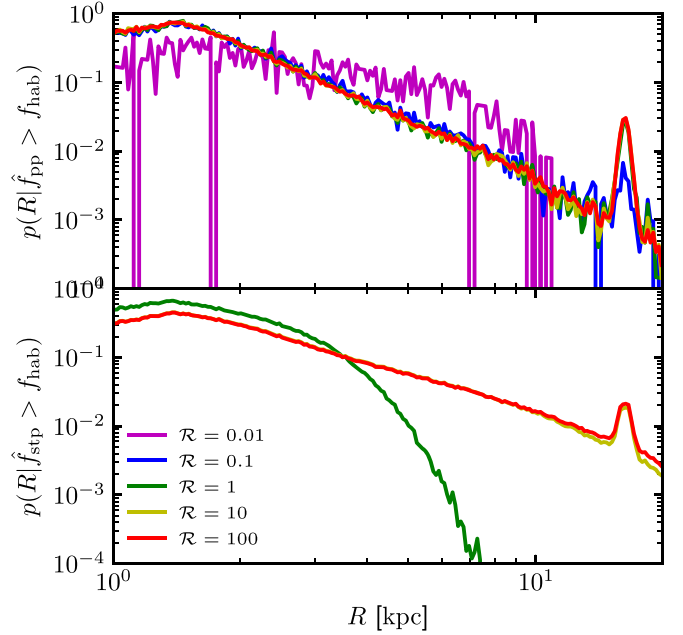
Figure 13. Radial distribution of star particles with unnormalized panspermia probabilities greater than the natural habitability ( p(R|\hat{f}_{\text{pp/stp}} > f_{\text{hab}}) ) in \text{gal}15784 at z = 0 , for different values of \mathcal{R} . p(R|\hat{f}_{\text{pp/stp}} > f_{\text{hab}}) is normalized such that its integral over R is 1.
