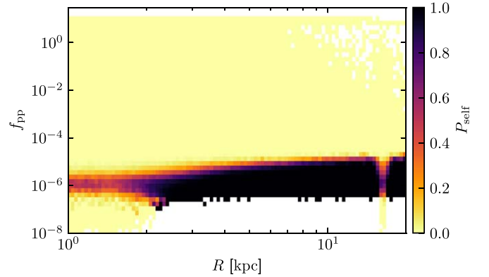
Figure 11. The probability of self-panspermia ( P_{self} ), where \mathcal{F}(x, x) > f_{pp/stp}(x)/2 , as a function of R and f_{pp}
