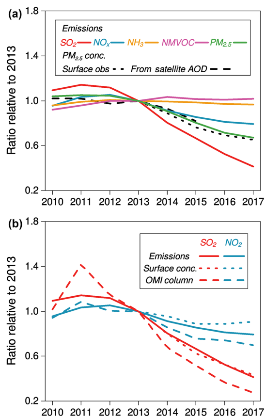
Figure 8. Emission trends compared with satellite- and ground-based observations. The satellite-retrieved \text{PM}_{2.5} concentrations (black, the dashed curve in a) (Lin et al., 2018) are compared with emission trends of \text{PM}_{2.5} precursors in (a). The 2010–2017 trends in \text{SO}_2 (red, the solid curve in b) and \text{NO}_x (blue, the solid curve in b) emissions are compared with OMI \text{SO}_2 (red, the dashed curve in b) and \text{NO}_2 (blue, the dashed curve in b) tropospheric columns for eastern China, respectively. Eastern China here includes the provinces of Beijing, Tianjin, Hebei, Shanxi, Shaanxi, Shandong, Henan, Hubei, Anhui, Jiangsu, Shanghai, and Zhejiang. The 2013–2017 trends in ground-based observations of \text{SO}_2 (red, the dotted curve in b), \text{NO}_2 (blue, the dotted curve in b), and \text{PM}_{2.5} (black, the dotted curve in a) are also presented. Data are normalized by dividing the value of each year by their corresponding value in 2013.
