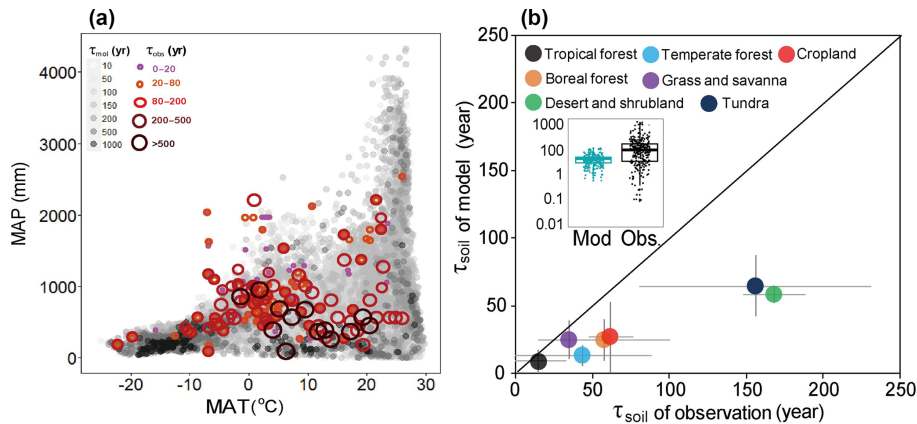
Figure 2. Global spatial variation of SOC transit time ( \tau_{soil} ) with climate and the difference of \tau_{soil} estimation between observations and models. (a) Spatial variation of \tau_{soil} with mean annual temperature (MAT) and mean annual precipitation (MAP). (b) Comparisons of modeled against observed \tau_{soil} . Details for the classification of biomes are provided in the method section.
