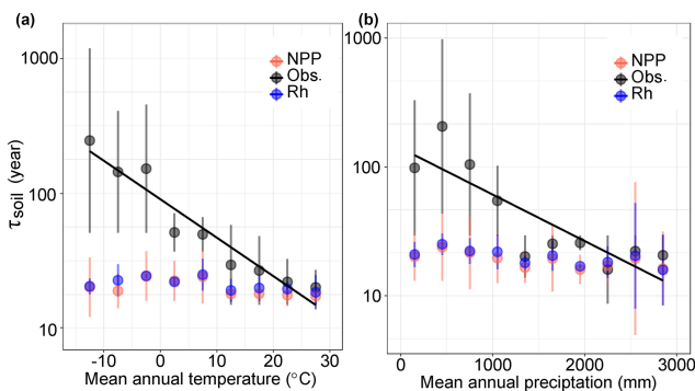
Figure 3. Relationships between SOC transit time ( \tau_{soil} ) and climate factors in both observations and CIMP5 models. The black solid lines show the negative correlation between \tau_{soil} and (a) mean annual temperature and (b) mean annual precipitation. The black dots indicate the aggregated \tau_{soil} over each category of MAT ( y = -5.47x + 1971.5 , r^2 = 0.49 , P < 0.01 ) or MAP ( y = -68.19x + 1222.6 , r^2 = 0.60 , P < 0.01 ). The red and blue dots present the mean value of multiple models based on the ratios of carbon stock over NPP and R_h , respectively.
