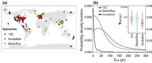
Figure 1. Spatial distributions of observational sites for estimates of SOC transit time ( \tau_{\text{soil}} , year). (a) The site locations of measurements with different approaches. (b) Probability density functions of \tau_{\text{soil}} measured with different approaches. Note that the left axis is for the ^{13}\text{C} and stock-over-flux approaches, and the right axis is for laboratory incubation studies.
