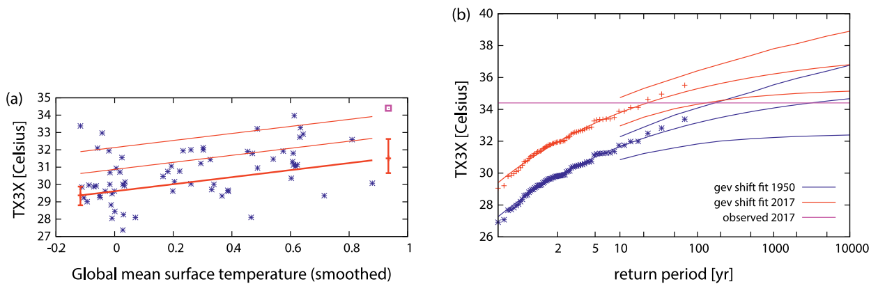
FIG. 2. An example of the results for the observed TX3X for the SE-box. (a) The fit applied to observations, where asterisks mark the observations, the thick line denotes the time-varying mean (fitted position parameter), the thin lines mark 1\sigma and 2\sigma (with \sigma the fitted scale parameter) above the mean, and the two vertical red whiskers show the 95% confidence interval of the fitted position parameter for the climates of 1950 (leftmost) and 2017 (rightmost). (b) Return period distributions shifted to the climates of 2017 (red lines and crosses) and the past (1950; blue lines and asterisks), including error margins (red and blue bounding curves). The purple square in (a) and horizontal line in (b) indicate the 2017 value (not included in the fits).
