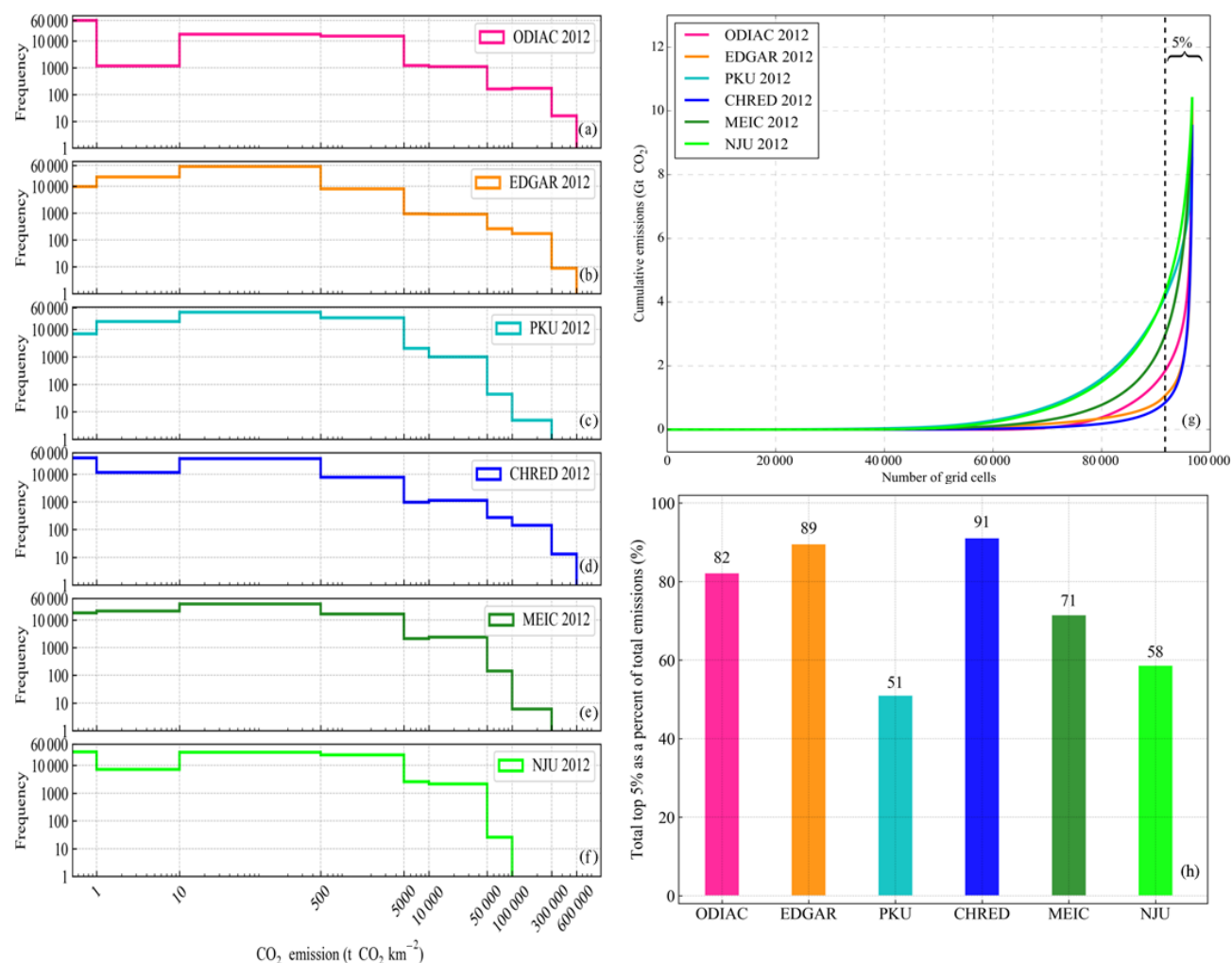
Figure 6. Frequency counts (a–f), cumulative emissions (g) (grids are sorted from low to high), and the top 5 % emitting grid plots (h) for ODIAC, EDGAR, PKU, CHRED, MEIC, and NJU in 2012 at a 10 km resolution.
