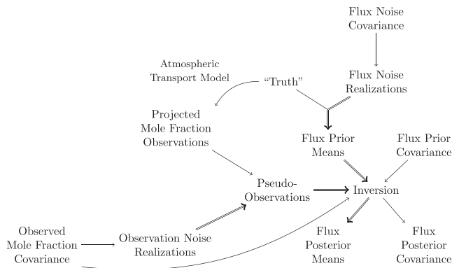
Figure 2. Flow chart describing the use of various variables for the experiments described in this section. Doubled lines denote parts with multiple realizations forming an ensemble. The noise realizations are the products of a pseudo-random number generator. The posterior means are generated from each pair of noisy observation and prior mean in turn. The “truth,” noise, and noise covariance are unknown for real-data applications. The flux noise and prior covariances are identical for this experiment.
