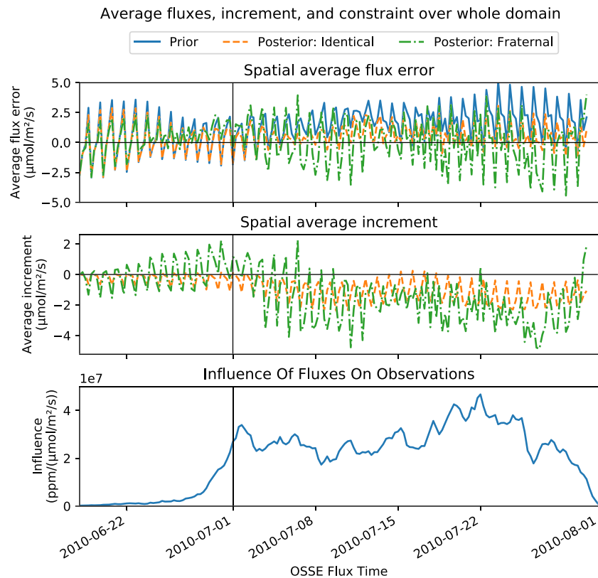
Figure 6. The top graph shows the magnitude of the difference between the prior and posterior estimates of the mean flux and the “true” flux the inversion was attempting to recover averaged over the spatial domain, both for the first ensemble member. The middle graph shows the change from the prior to the posterior mean flux estimates, again for the first ensemble member and averaged over the spatial domain. The bottom graph shows the influence of the fluxes at a given time on the average observation, also averaged over the spatial domain. The vertical line in each graph marks 1 July, the day of the first observation used in the inversion.
