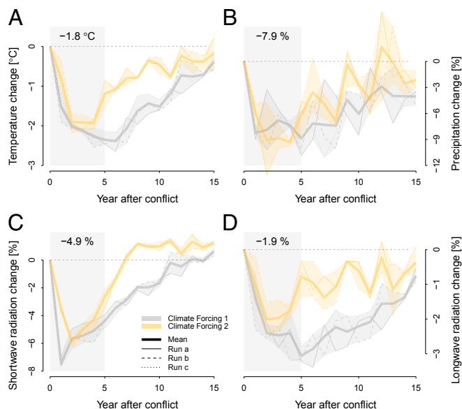
Fig. 1. Nuclear conflict-induced global climate perturbations. Changes in (A) 2-m air temperature (°C), (B) precipitation (%), and (C) surface incoming shortwave and (D) longwave solar radiation (%) are shown across 15 post-conflict years for two climate simulation sets (climate forcing 1 and 2), with three ensemble members each (runs a–c). Changes are shown as absolute (temperature) and relative (all other variables) differences between control and perturbed global mean values, calculated over the global land area. The average year 1 to 5 change is highlighted on top of the shaded boxes.
