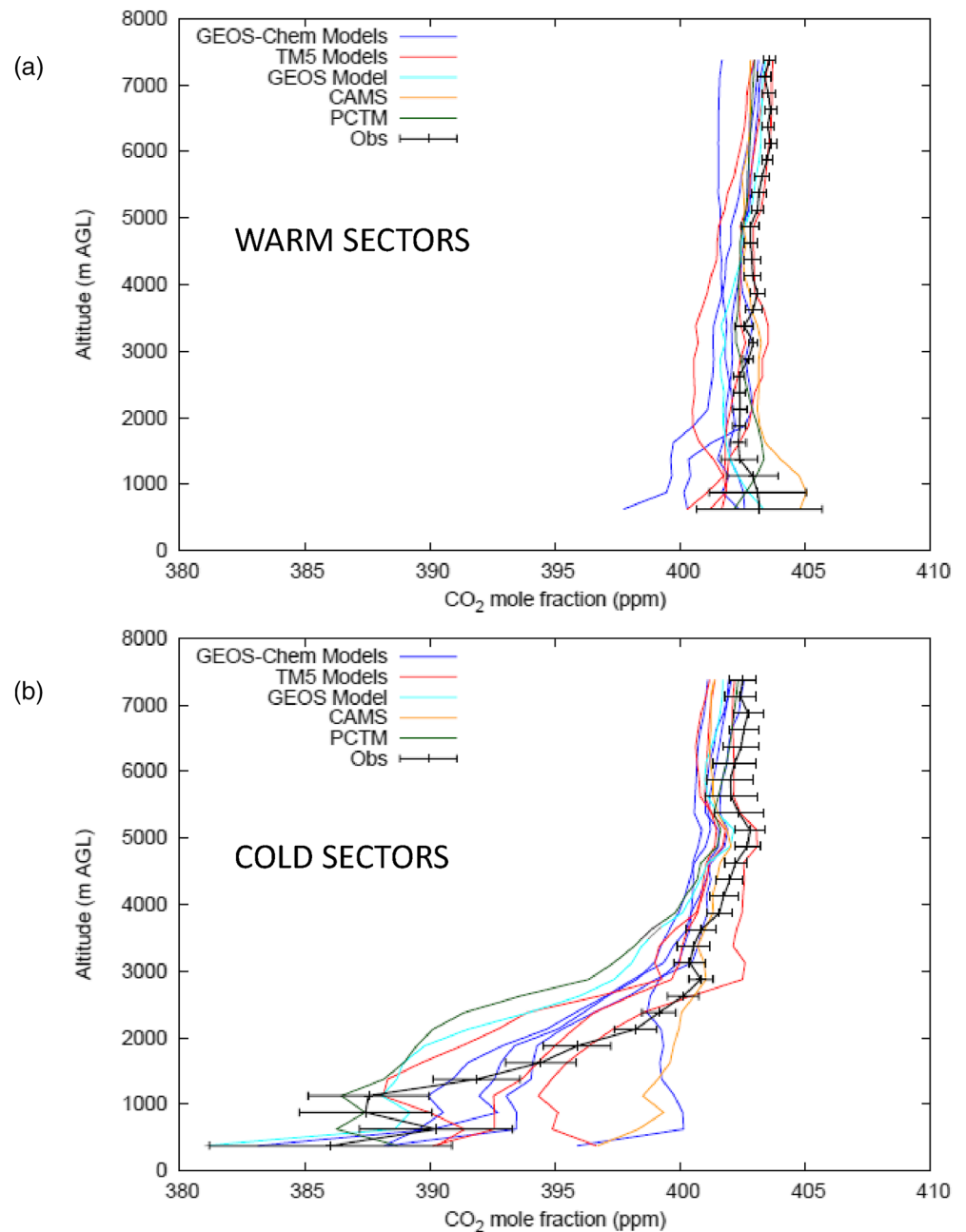
Figure 3. Same as Figure 1, but for the Midwest region (1–15 August, 2016). Statistics generated from 29 total warm sector profiles and 29 total cold sector profiles.
