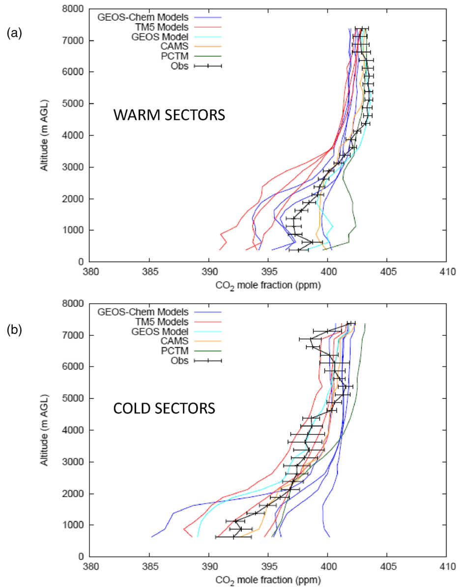
Figure 1. Vertical profiles of mean observed (black) and modeled (colored) mole fraction as a function of altitude AGL for (a) Mid-Atlantic warm sectors and (b) cold sectors, from 16 to 31 July, 2016. Blue indicates OCO-2 MIP models using GEOS-Chem offline transport; red indicate models using TM5 offline transport; light blue indicates the GEOS-5 inline transport member; orange indicates the CAMS member; green indicates the PCTM transport member. Bars on the observations indicate \pm\sigma / \sqrt{N} , as described in the text. Statistics generated from 36 total warm sector profiles and 12 total cold sector profiles.
