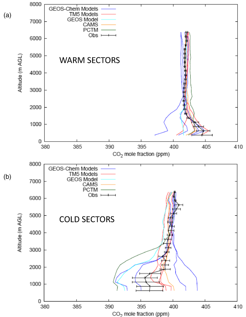
Figure 5. Same as Figure 1, but for the South region (16–31 August, 2016). Statistics generated from 31 total warm sector profiles and 11 total cold sector profiles.
