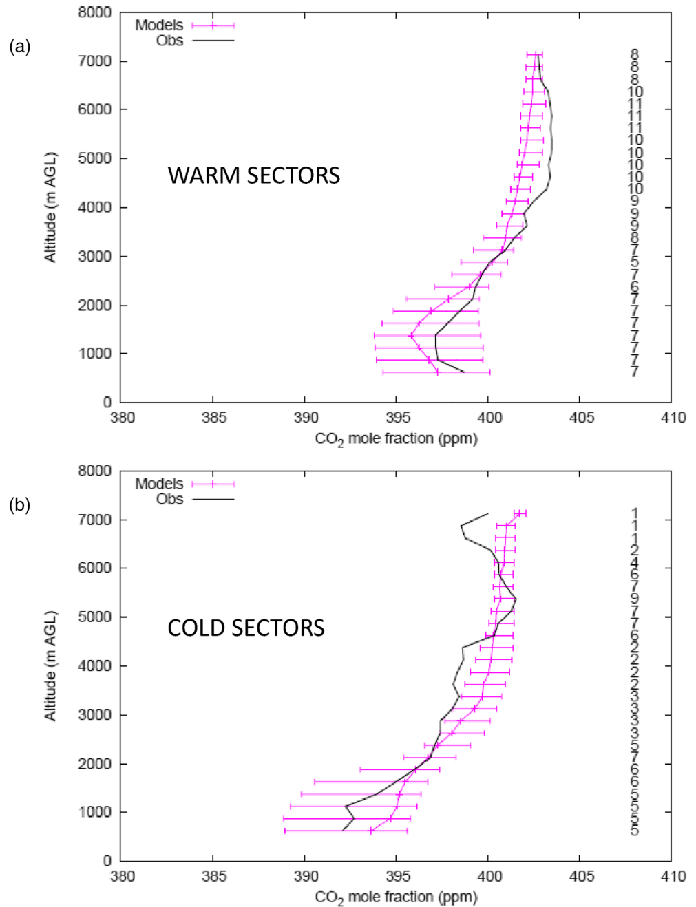
Figure 2. Vertical profiles of mean observed mole fraction (black) and model spread of mole fraction (colored) as a function of altitude AGL for (a) Mid-Atlantic warm sectors and (b) cold sectors, from 16 to 31 July, 2016. Vertical colored curve indicates median (50th quantile) value of model mole fraction; bars indicate location of 25th and 75th quantile of model mole fraction. Numbers to right indicate ordered rank of observations relative to models, with 1 indicating observed value is less than all 10 model values, and 11 indicating observed value is greater than all 10 model values.
