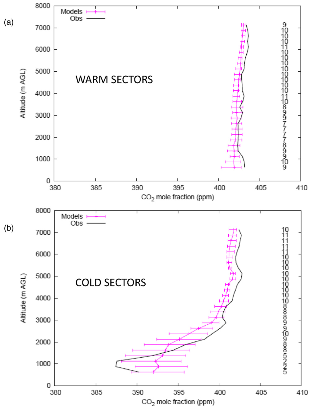
Figure 4. Same as Figure 2, but for the Midwest region (1–15 August, 2016).
