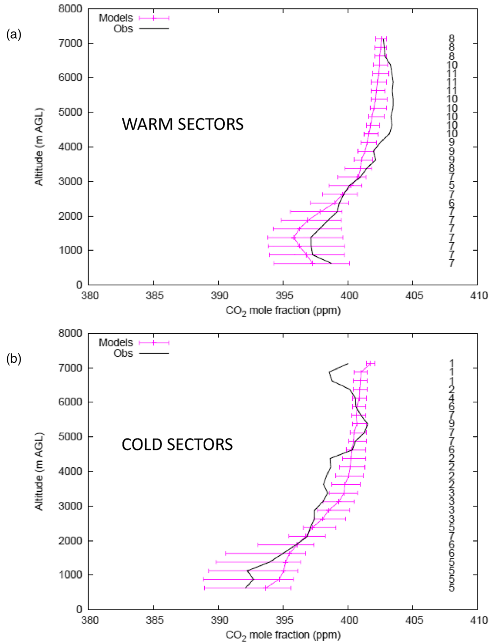
Figure 6. Same as Figure 2, but for the South region (15–31 August, 2016).
