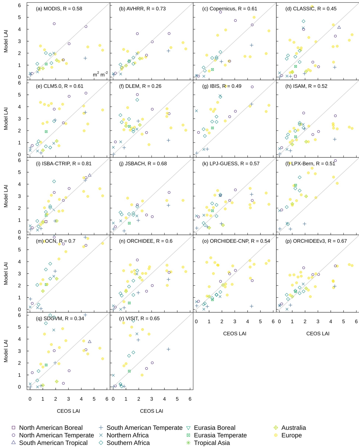
Figure 8. Evaluation of leaf area index against site-level measurements with units in m^2 m^{-2} .
