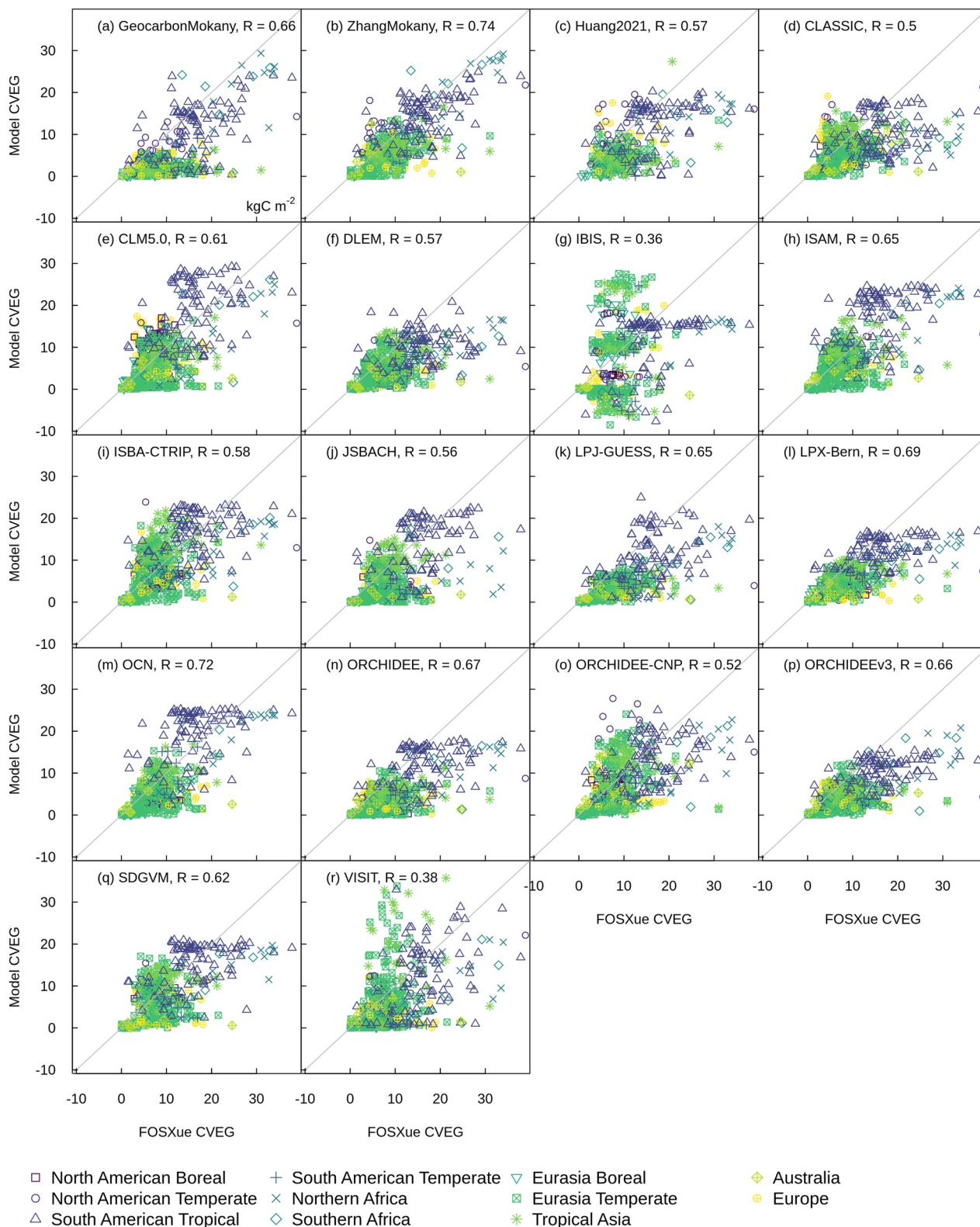
Figure B5. Evaluation of vegetation carbon against site-level measurements in units of \text{kgC m}^{-2} .
