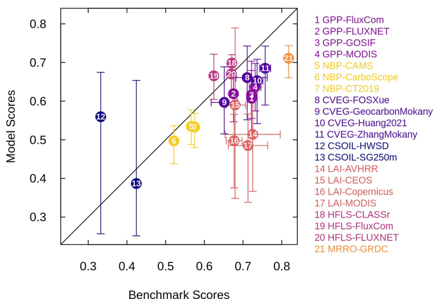
Figure 9. Model scores and benchmark scores, where dots present multi-model mean values and bars give the total range of scores.
