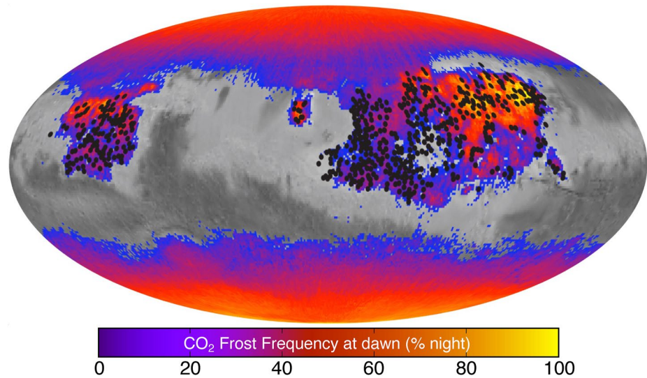
Figure 9. Distribution of slope streaks (black dots) extracted from Schorghofer et al. (2007) and diurnal CO 2 frost distribution and frequency (adapted from Piqueux et al. (2016)). No color is reported where no diurnal frost is modeled to be present at dawn. Here, 0 means no diurnal frost ever and 100 means diurnal frost is present every dawn of the year. Background is a TES albedo map, Mollweide projection, 200°E prime meridian.
