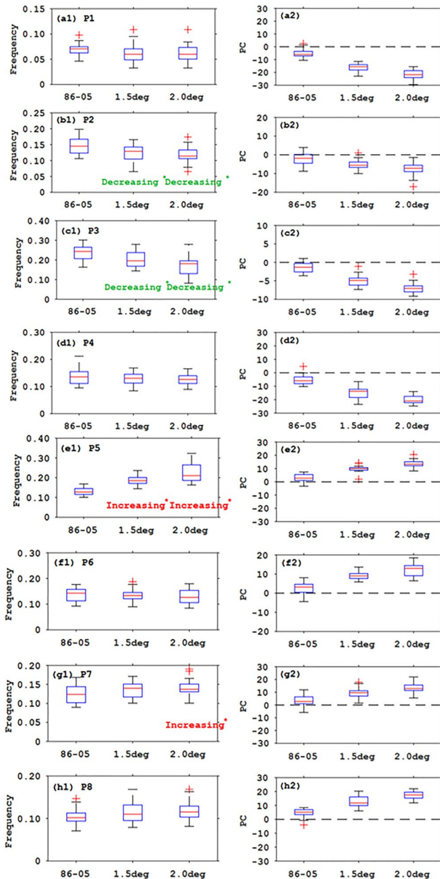
Figure 3. Boxplots showing occurrence frequency for eight rainfall patterns (a1–h1) and projection coefficients of corresponding circulation fields for eight rainfall patterns (a2–h2) during the three time periods (historical and 2 global warming targets). “Increasing*” and “Decreasing*” indicate the increasing and decreasing trend that passes the 95% significance test using Student’s t -test, respectively.
