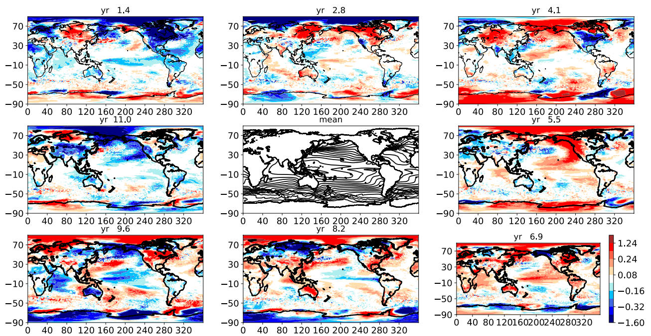
Fig. 2 Composites of the 11-years mode of global STs found in the CESM model simulation, in eight phase categories, displayed clockwise and labeled by the epoch at the middle of the category; color
