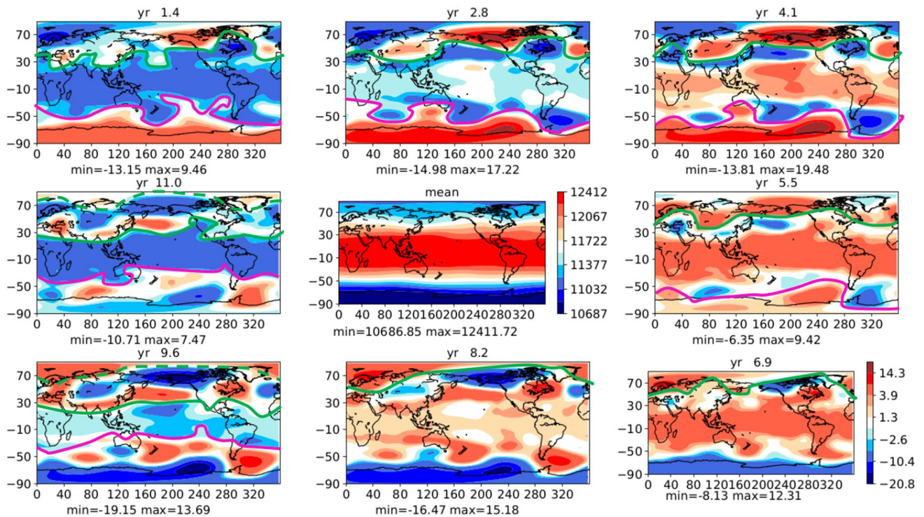
Fig. 5 As in Fig. 2 but for 200-hPa geopotential. The green solid line shows the approximate position of a specific hemispheric level curve in the northern hemisphere, in each phase of the oscillatory mode; its southern-hemisphere counterpart is shown as a solid magenta line.
