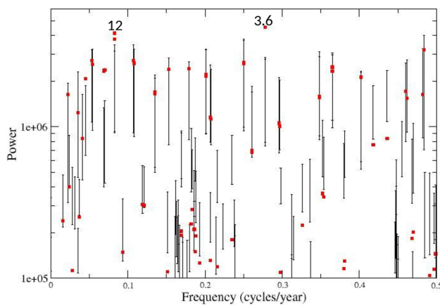
Fig. 10 Spectral analysis of the global geopotential 200-hPa field, as found in the NCEP-NCAR reanalysis, and by using MSSA with a window width of M = 20 years; please see text for detrending the time series, subtracting the seasonal cycle, and varimax rotation. The graphical conventions and significance methodology are as in Fig. 1
