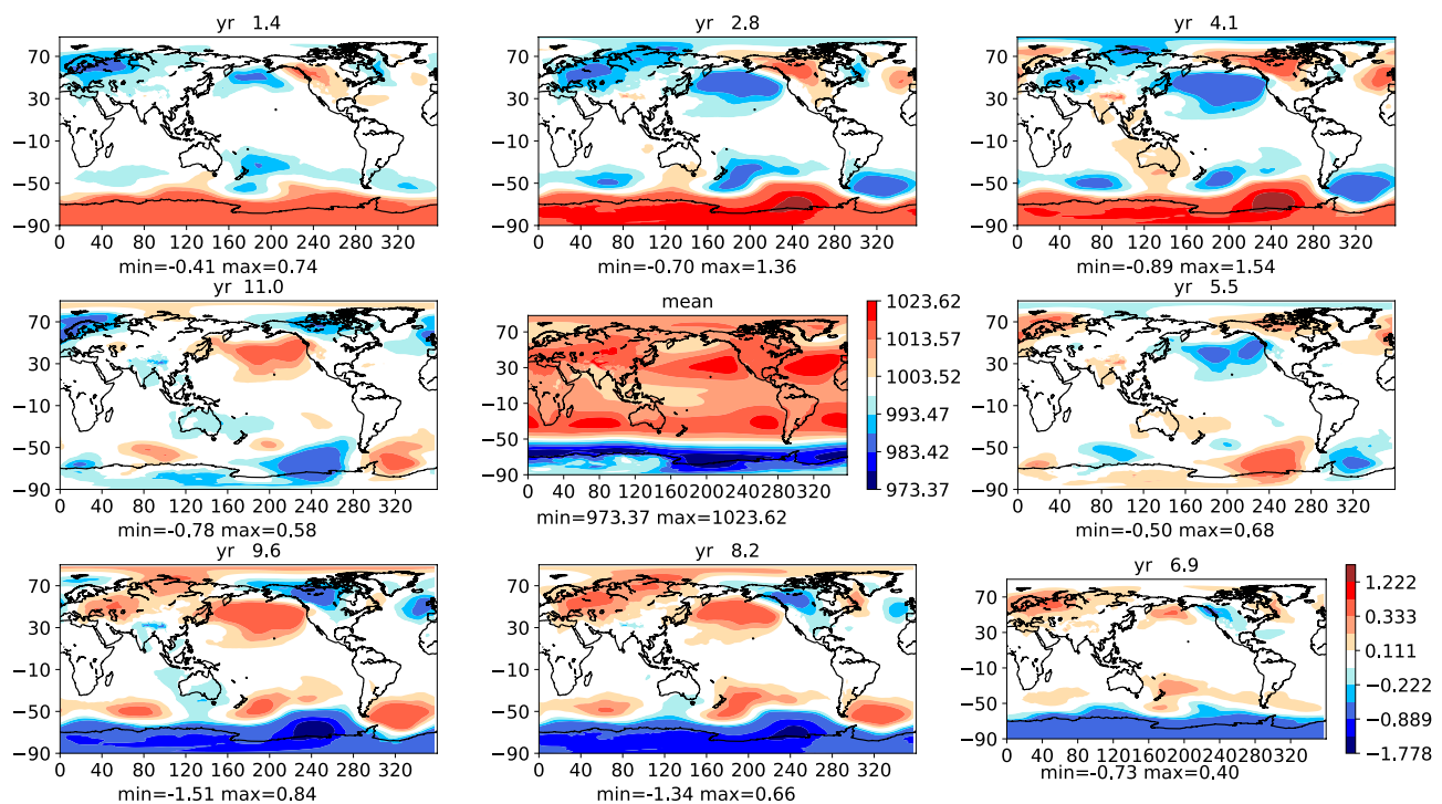
Fig. 6 As in Fig. 5 but for the SLP field. Color bar is in hPa for the phases of the oscillation, as well as for the mean field
