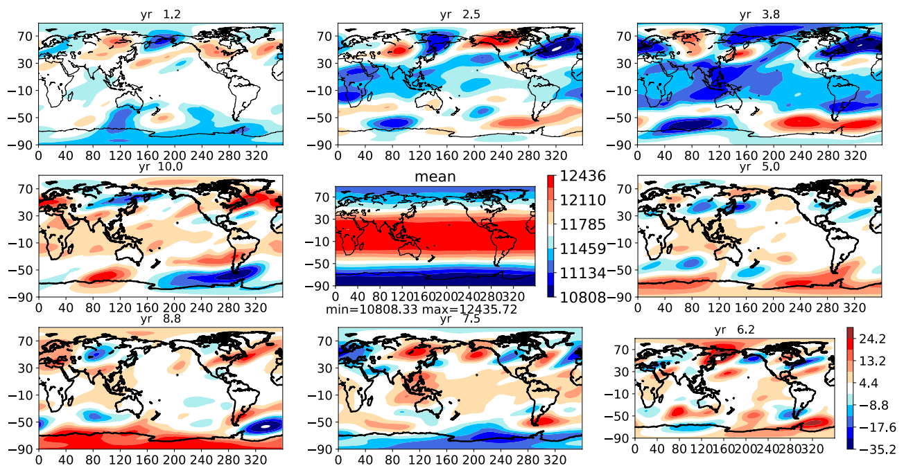
Fig. 20 Same as Fig. 17 but for the 10-years mode in the ERA5 reanalysis, with no ST-EOF-based filtering. See text for details
