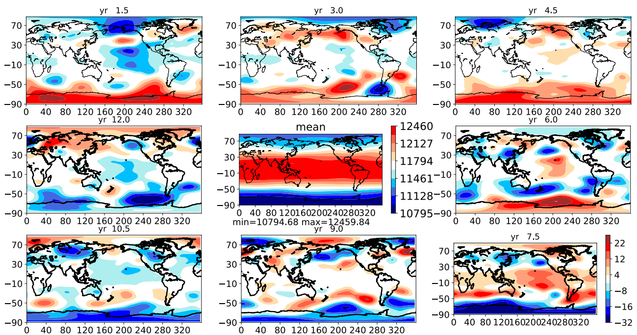
Fig. 19 Same as Fig. 17 but for the 12-years mode in the NCEP-NCAR reanalysis, with no ST-EOF-based filtering. See text for details
