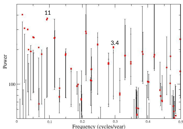
Fig. 1 Spectral analysis of the time series of the global ST, SLP and 200-hPa fields, as found in the CESM model simulation, after detrending and by using MSSA with a window width M = 20 years, after subtracting the seasonal cycle and applying varimax rotation for better frequency separation (Groth and Ghil 2015; Groth et al. 2017). The estimated variance of each mode in the dataset is shown as a filled red square, while lower and upper ticks on the error bars indicate the 5th and 95th percentiles of a red-noise process constructed from a surrogate data ensemble of 100 time series. Each of the surrogates has the same variance and lag-one auto-correlation as the original record. The surrogate time series were produced by projecting the first 40 principal components (PCs) of the MSSA analysis onto the basis vectors of a red-noise process
