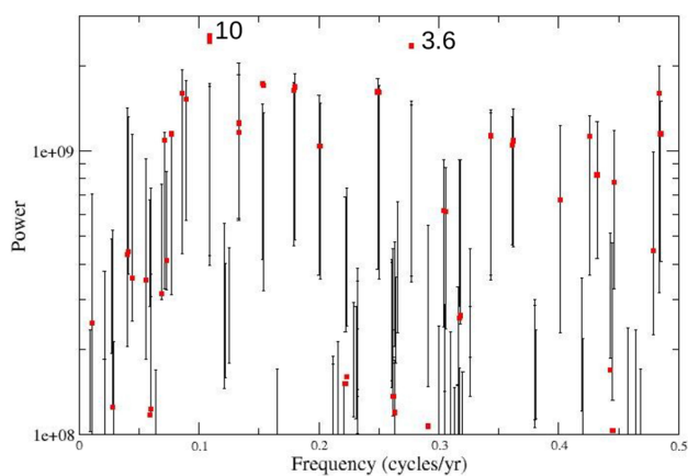
Fig. 13 Spectral analysis of the global geopotential 200-hPa field, as found in the ERA5 reanalysis, and by using MSSA with a window width of M = 20 years; please see text for detrending the time series, subtracting the seasonal cycle, and varimax rotation. The graphical conventions and significance methodology are as in Fig. 1
