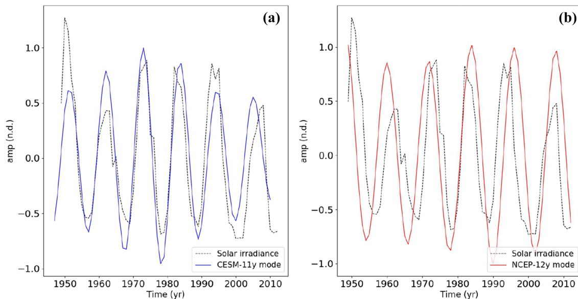
Fig. 21 Solar cycle and its relation to the decadal mode. a Total solar irradiance (TSI: Coddington et al. 2016) (black dashed curve) and the decadal mode (blue solid curve) in the CESM simulation; and b TSI
