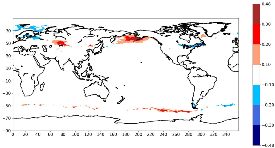
Fig. 18 Correlation map between S-PC1 of the CESM's 11-years oscillatory mode and its simulated ST evolution
