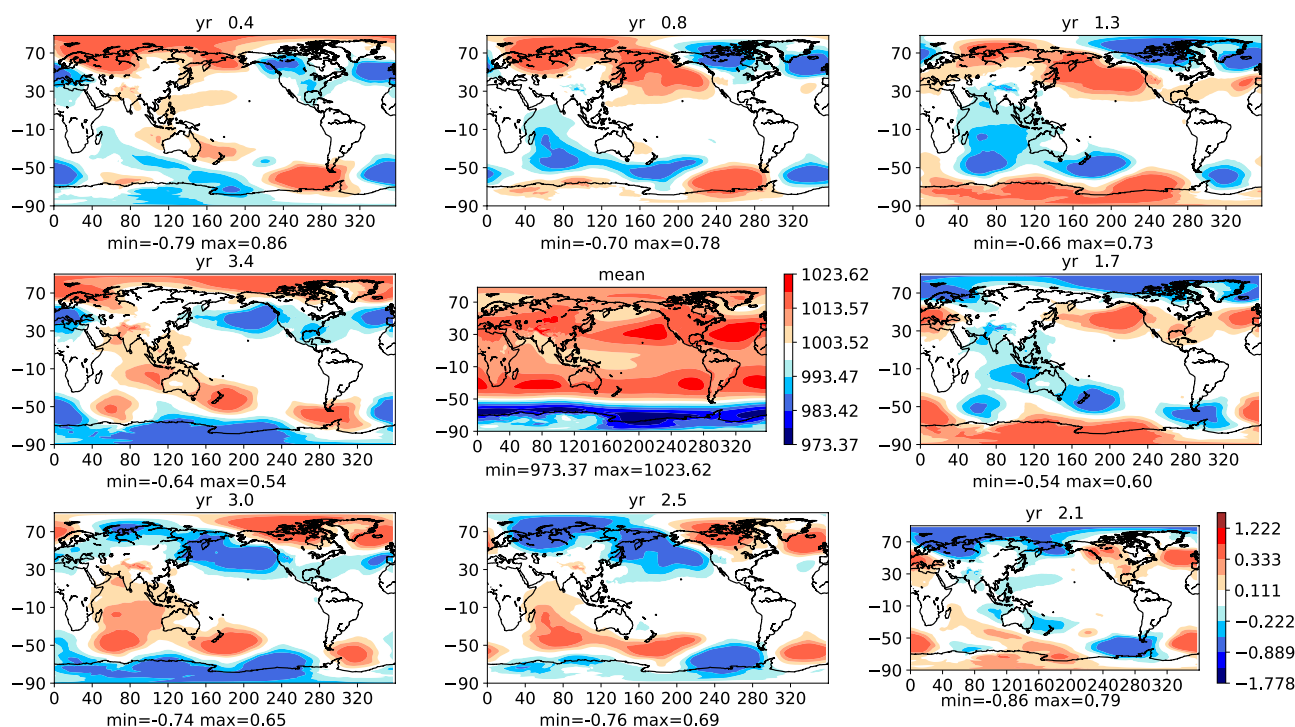
Fig. 9 As in Fig. 7 but for SLP. The mean SLP field is plotted in the middle panel and the color bars are as in Fig. 6
