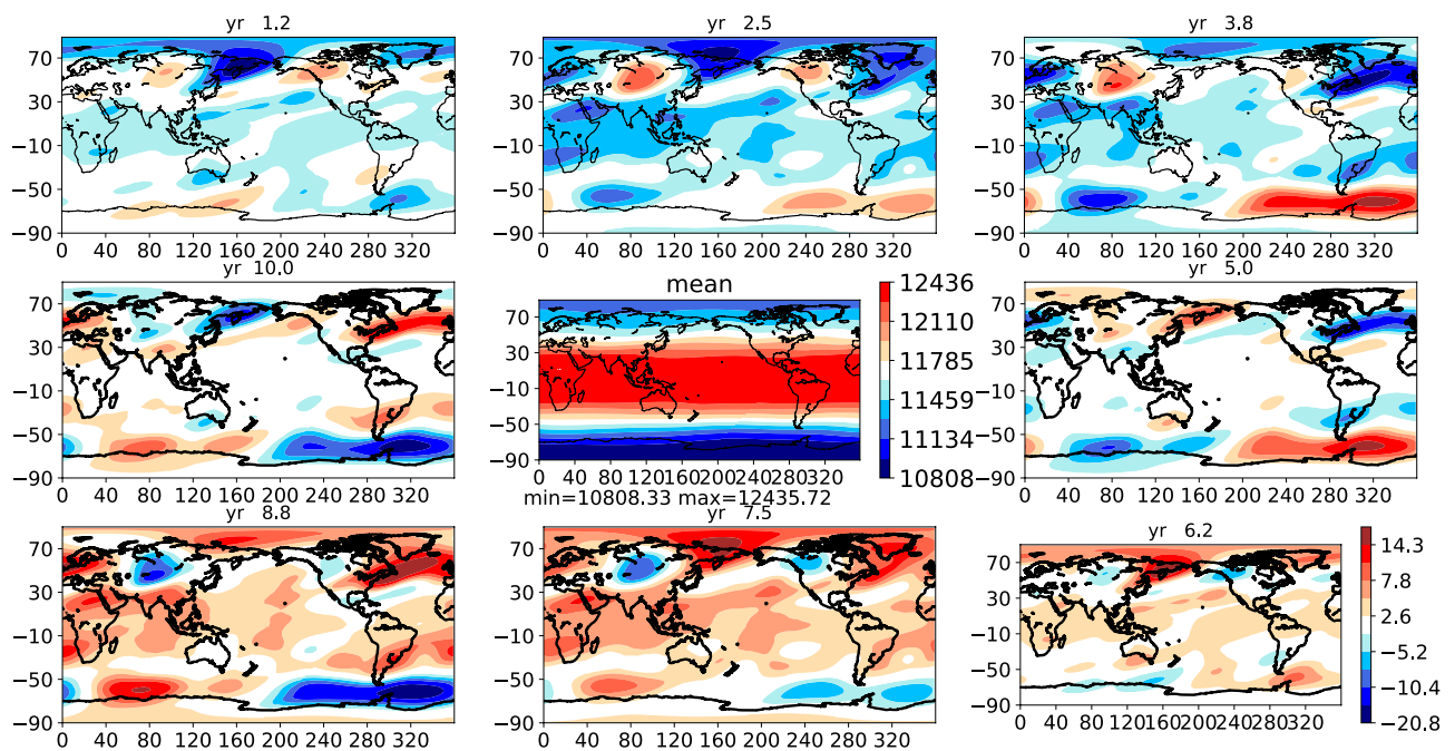
Fig. 14 Composites of the 10-years mode of global geopotential at 200 hPa, as found in the ERA5 reanalysis; panel ordering as in Fig. 2, color bars as in Fig. 5. These composites are based on MSSA pair (1,2), which captures 3.5 of the interannual variance
