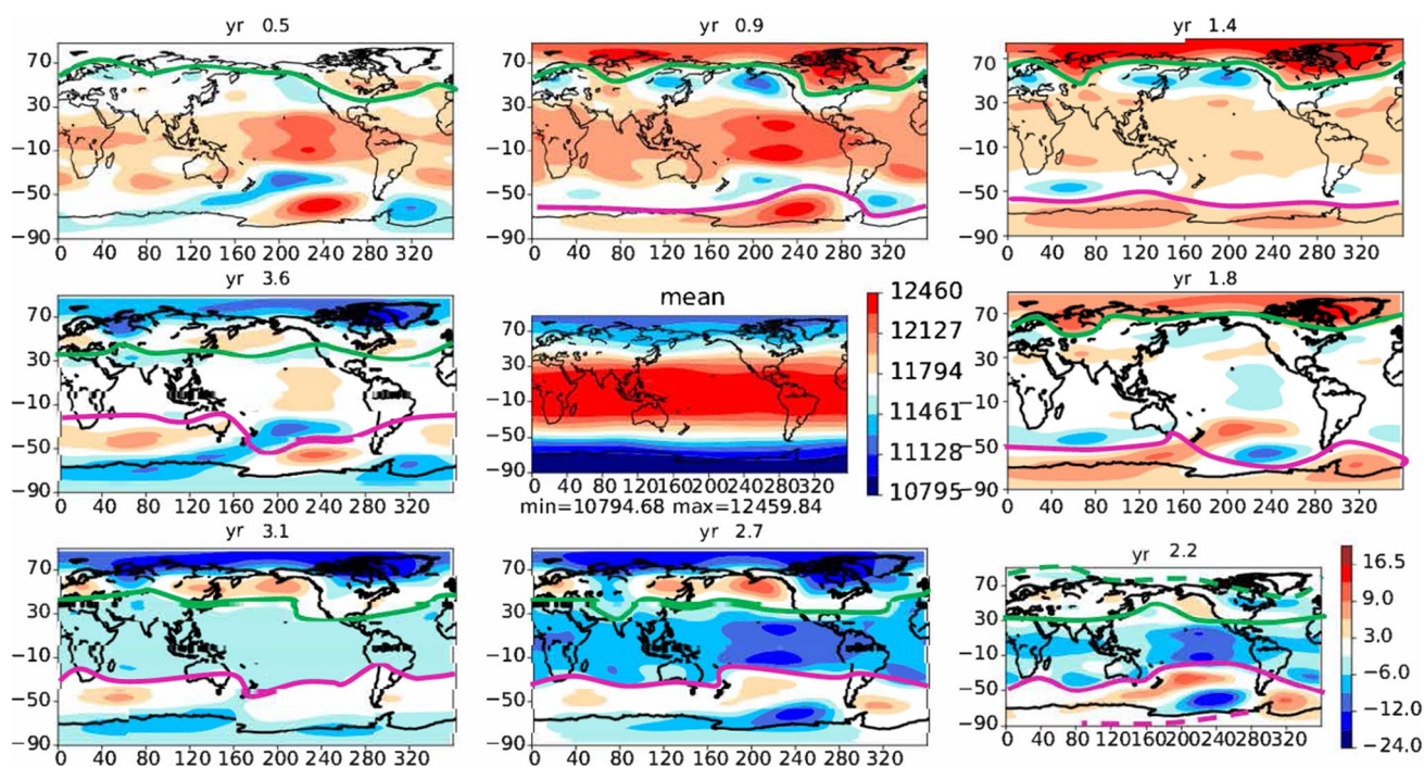
Fig. 12 Same as Fig. 11 but for the 3.6-years mode. The composites here are based on MSSA pair (1,2), which captures 6% of the interannual variance. The mean geopotential field in the middle panel is identical to that in Fig. 11
