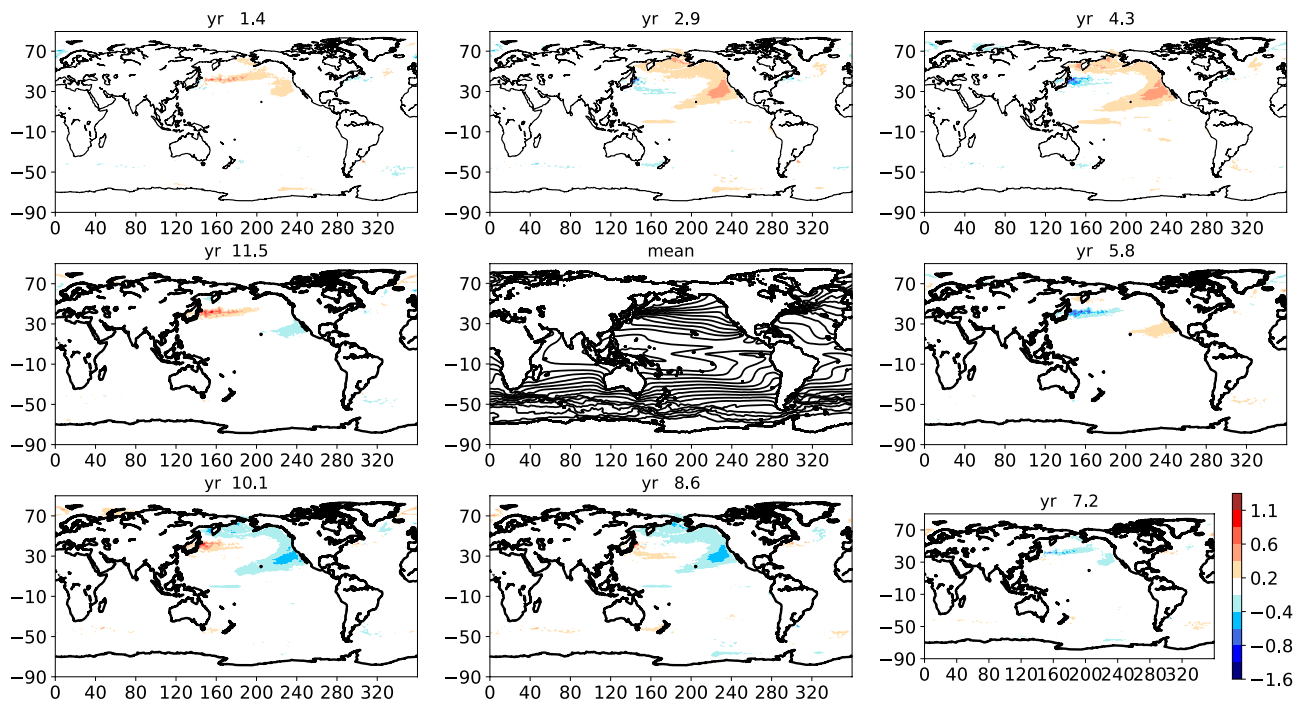
Fig. 4 Composites of the 11.5-years mode of global SSTs, given here by the temperature at a 5-m depth in the CESM model. Same panels and color bar units as in Fig. 2
