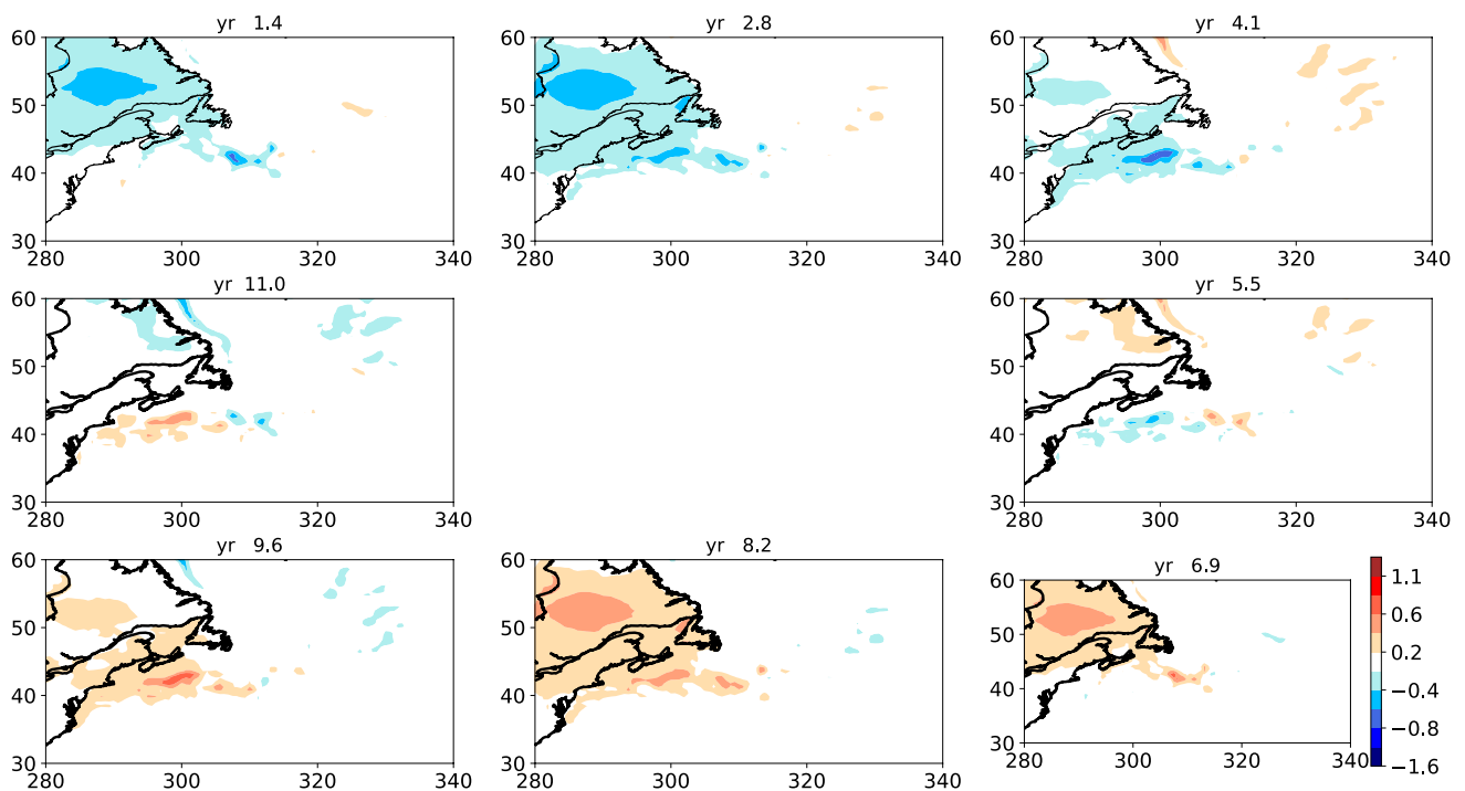
Fig. 3 Composites of the 11-years mode of global STs shown in Fig. 2, but zooming over the North Atlantic basin (NAB) in the Gulf Stream area (35 N–46 N, 287 E–310 E), in eight phase categories.
