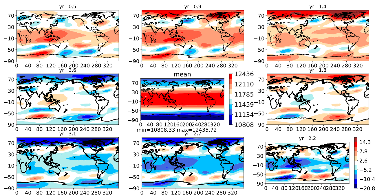
Fig. 15 Same as Fig. 11 but for the 3.6-years mode. The composites here are based on MSSA pair (3,4), which captures 3% of the interannual variance. The mean geopotential field in the middle panel is identical to that in Fig. 14
