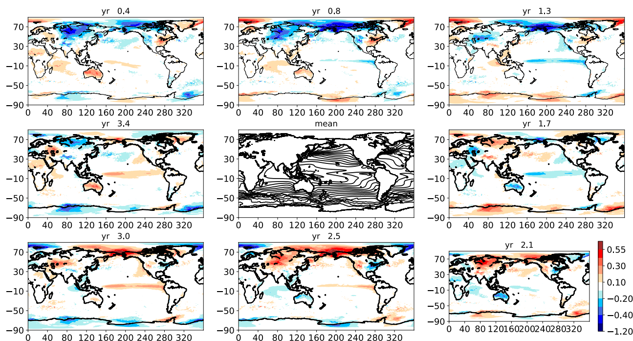
Fig. 7 Composites of the 3.4-years mode of global ST, in eight phase categories. These composites are based on MSSA pair (16,18), which captures 3% of the interannual variance. Same panels as in Fig. 2 and middle panel identically the same
