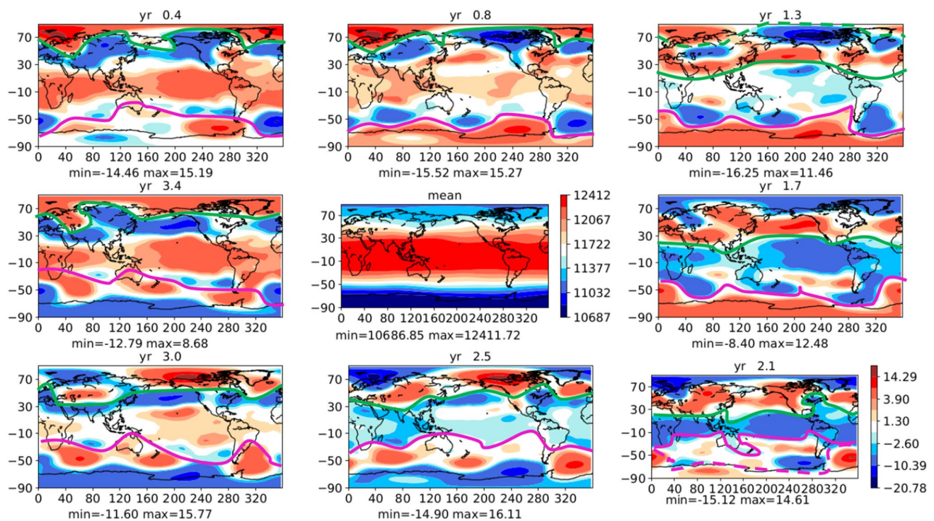
Fig. 8 As in Fig. 7 but for the geopotential at 200 hPa. Same panels and convention for the green and magenta solid and dashed lines as in Fig. 5
