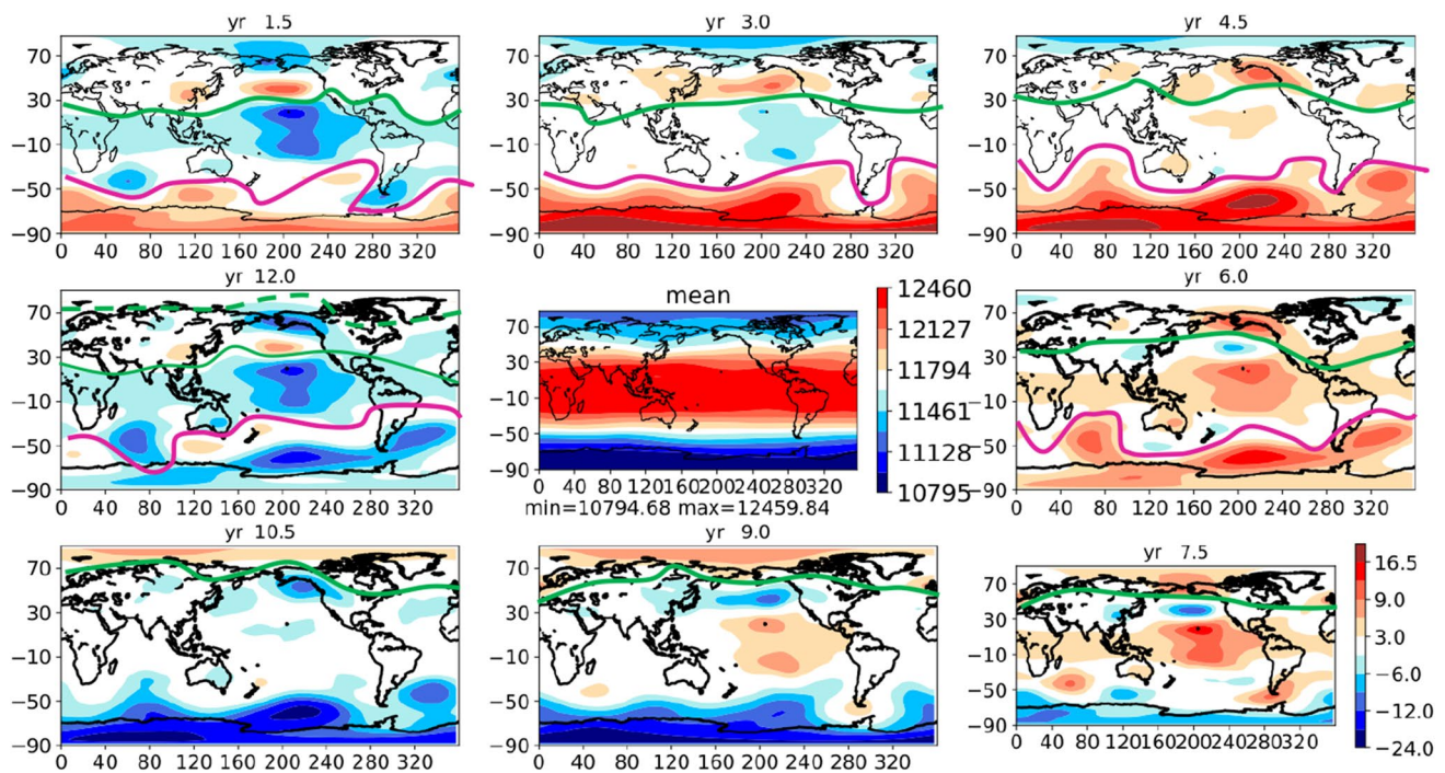
Fig. 11 Composites of the 12-years mode of global geopotential at 200 hPa, as found in the NCEP-NCAR reanalysis; panel ordering as in Fig. 2, color bars as in Fig. 5. These composites are based
