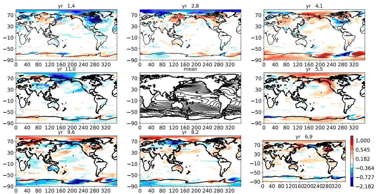
Fig. 16 Same as in Fig. 2 but for ST composites based on S-PC1 of the MSSA pair (3,4) and the CESM-simulated field evolution; see text for details. No filtering through the MSSA ST-EOFs has been used in this compositing. The mean ST field in the middle panel has contour interval (CI) = 2 K
