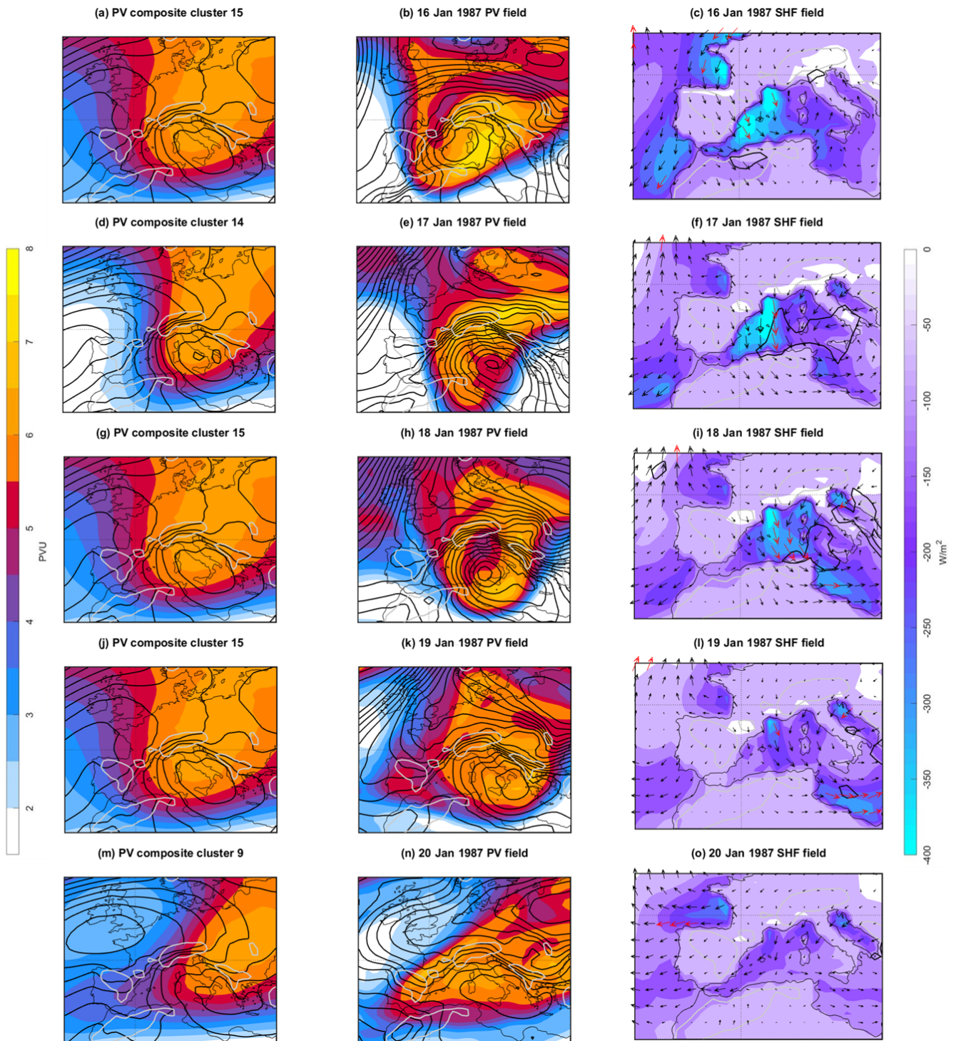
Figure 10. An illustrative AWB event identified by the transition 15 → 9. Shown are vertically averaged (320–340 K) daily PV distributions and SLP (black contours) throughout a mistral event (middle column), alongside their corresponding cluster composites (left column). Surface impact is shown on the right column in terms of the sum of sensible and latent heat fluxes ( W/m^2 , shaded), 10 m wind vectors (the red vectors represent magnitude in the upper quartile) and daily accumulated precipitation (black contours, 10 and 30 mm/d).
