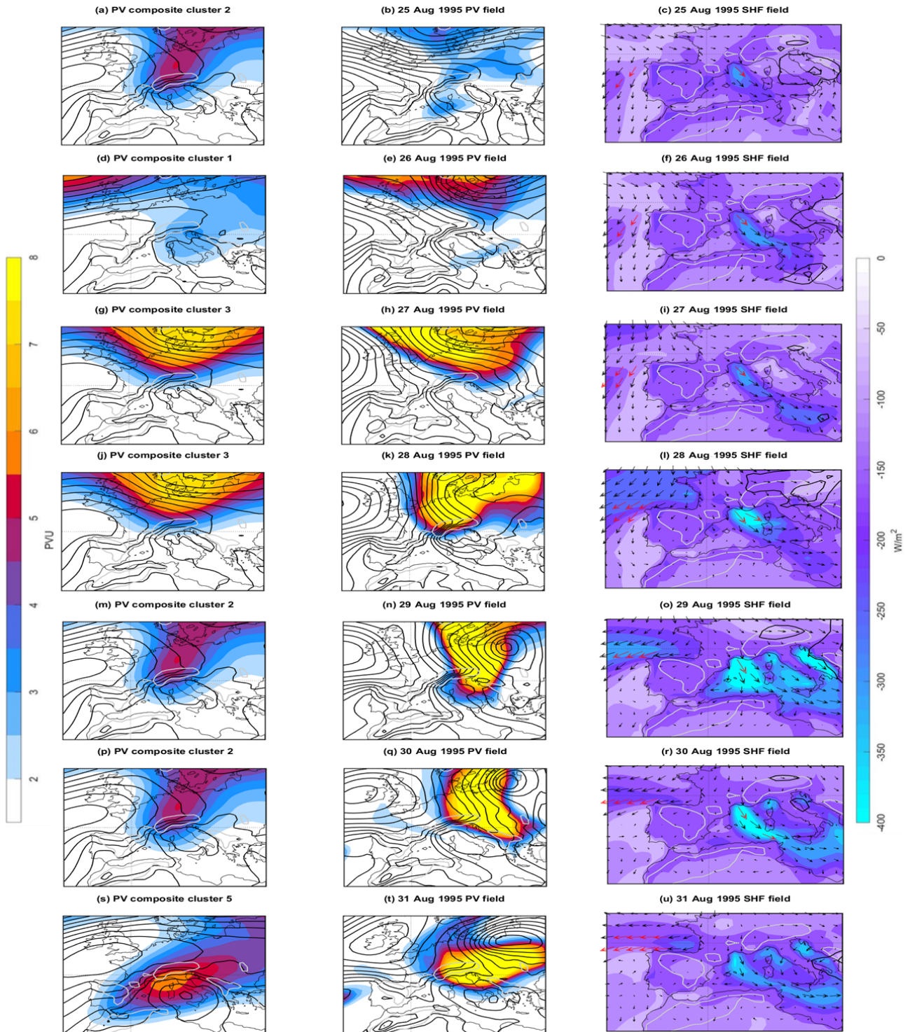
Figure 12. As in Fig. 10 but for a summer cutoff formation event identified by the transitions 2 → 1 and 2 → 5.
