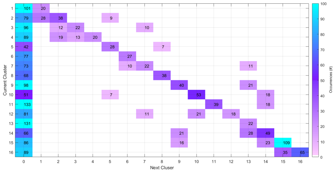
Figure 7. Transition probability matrix, based upon daily cluster transitions from the current cluster to the cluster on the next day (colored by number of days). The total days in each transition are given by the numbers in the corresponding rectangle. The 0 column represents the ending of mistral events, and the diagonal represents the probability to remain in the same cluster for the next day. Only statistically significant (90 % confidence level) transitions occurring within mistral events are shown.
