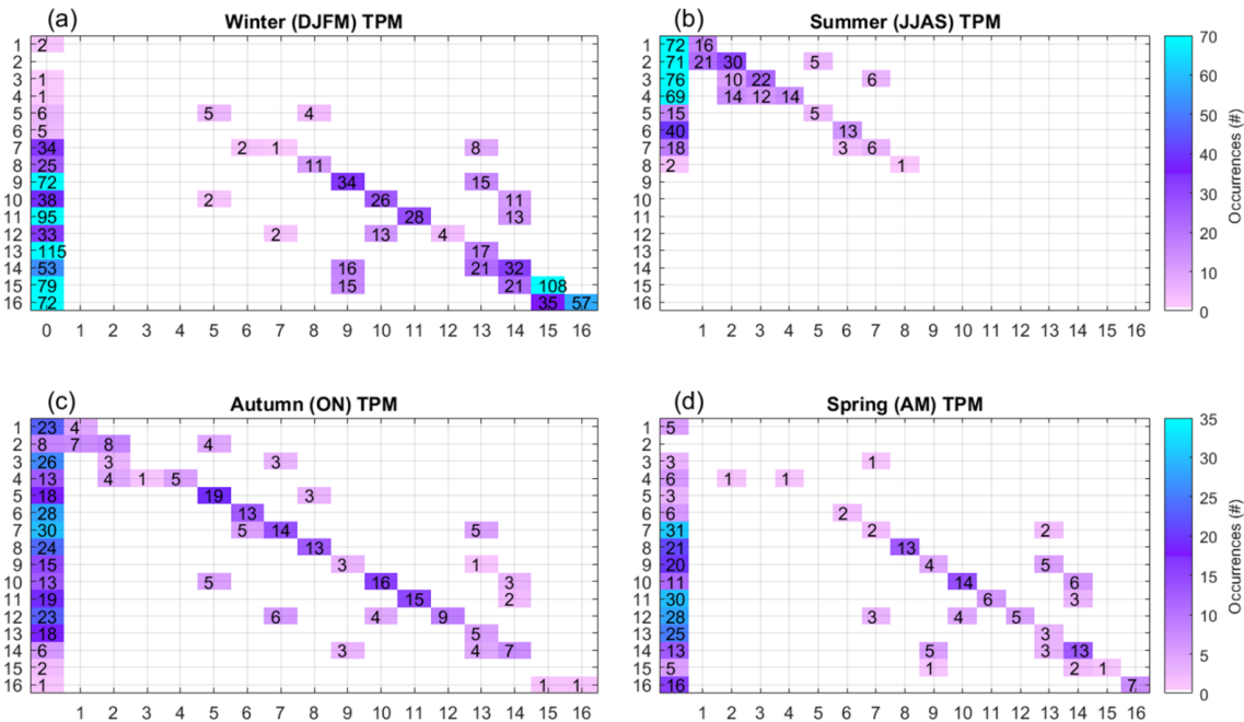
Figure 8. The same as Fig. 7 but separating by the different seasons. Note the 2-month periods in autumn (October–November) and spring (April–May), compared to 4 months in winter (December–March) and summer (June–September), and the different color scales, accordingly.
