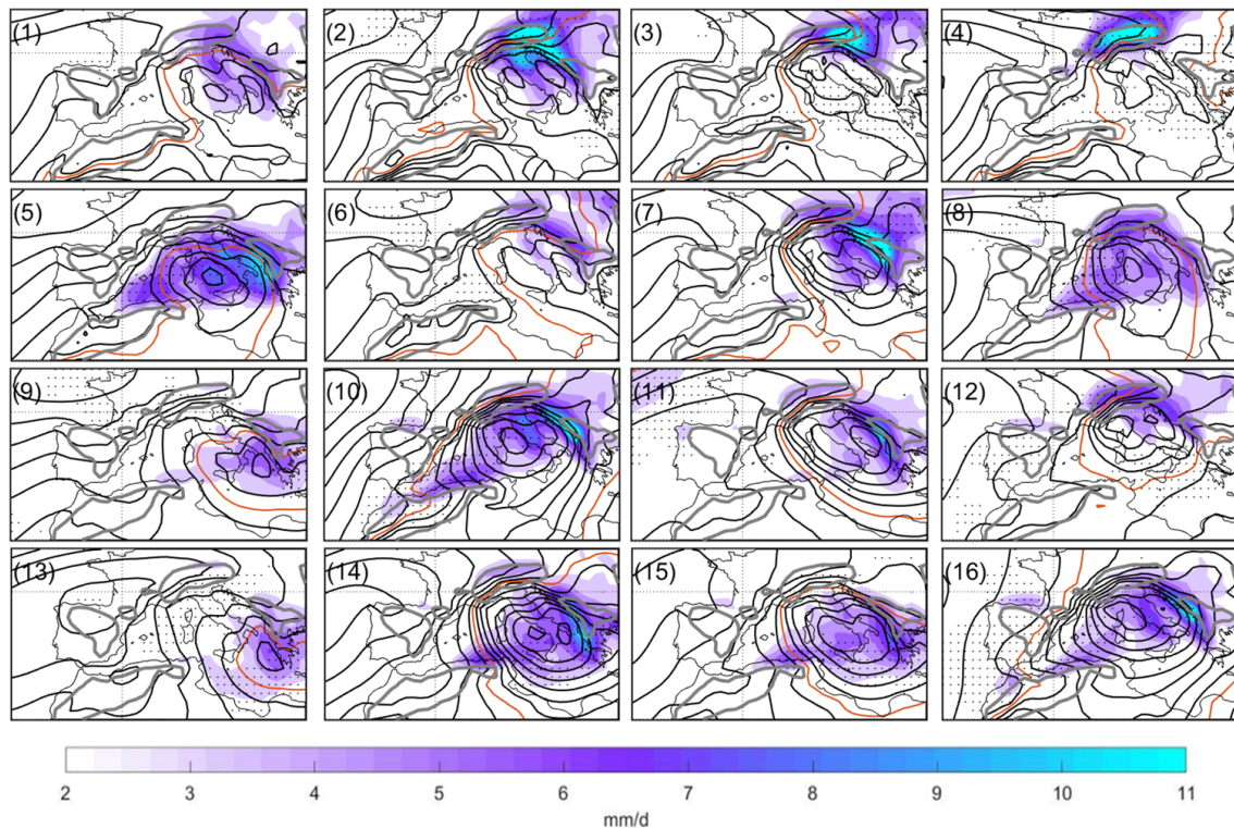
Figure 5. The same as Fig. 3 but for a smaller domain showing SLP (hPa, black contours) at 1 hPa intervals below 1015 hPa (colored line) and 2 hPa intervals above 1015 hPa. Daily accumulated precipitation (mm/d) is shaded. Dotted regions indicate statistical significance > 95 % for the precipitation composites compared to the average mistral flow.
