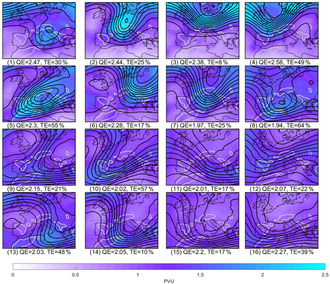
Figure B1. Standard deviation (SD) of isentropic PV within each cluster. The quantization and topographic errors (QE in PVU and TE in %, respectively) are noted at the bottom of each panel, following the cluster number. The average QE and TE for the network are 2.2 PVU and 30 %, respectively.
