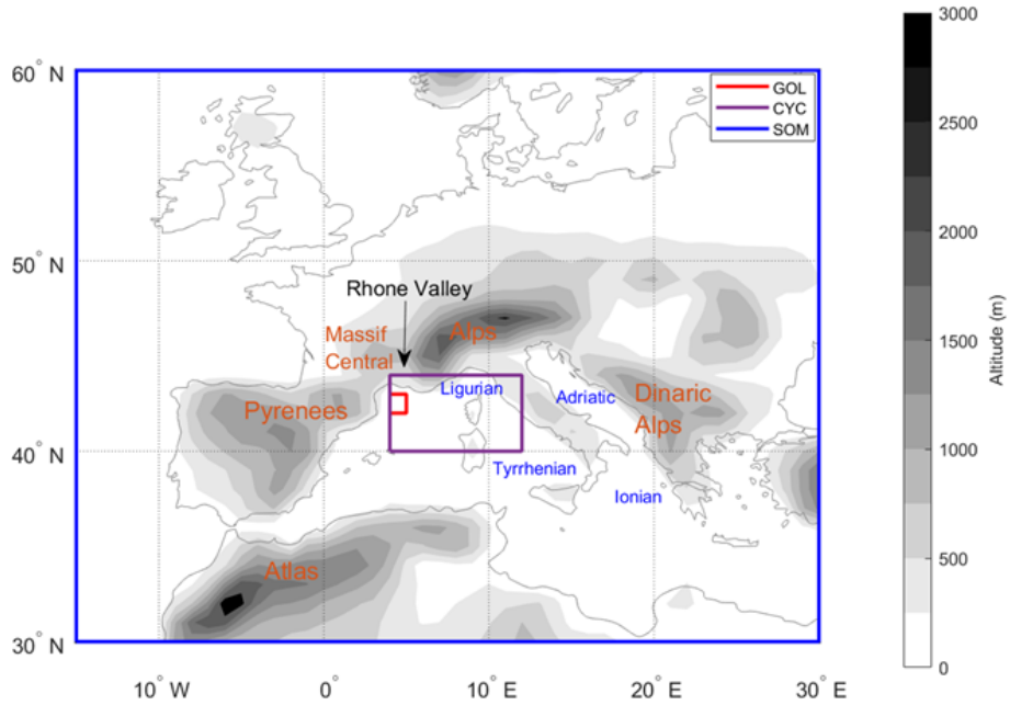
Figure 1. Geographical domains used in the analysis (see Methods section). The whole domain is used as SOM analysis input; the subregion where the Genoa cyclones are detected (CYC) and the subregion in which a northerly flow is required by the mistral definition (GOL) are marked in purple and red boxes, respectively. The topographic height from ERA-Interim is shown in shading (m).
