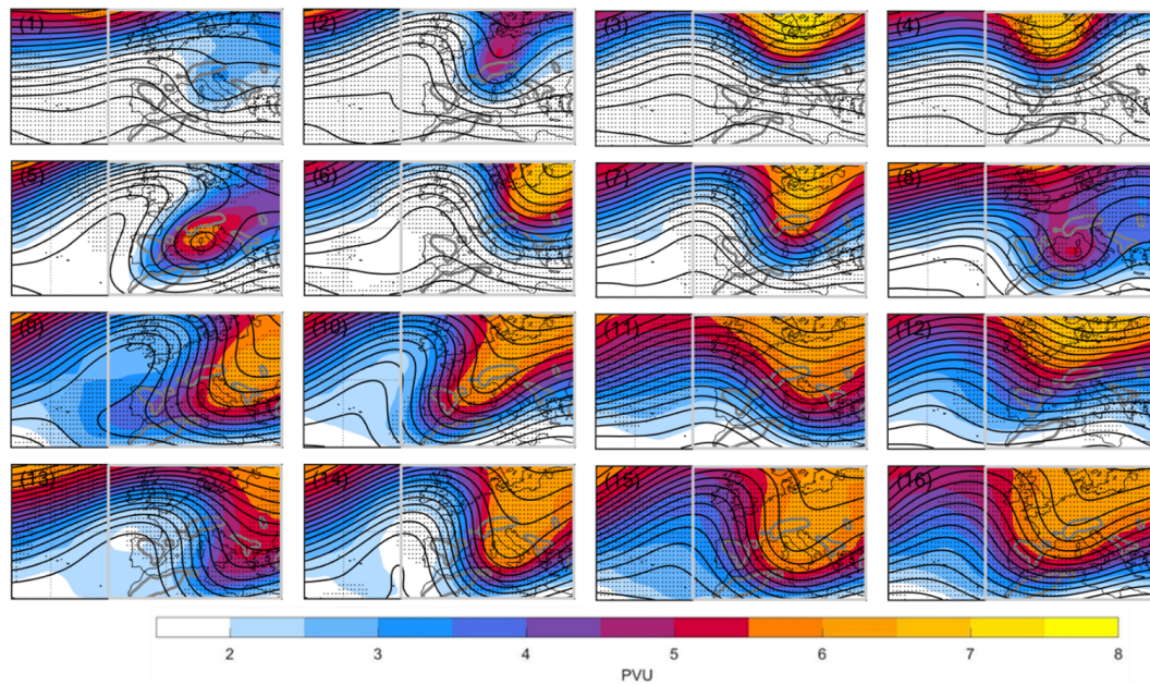
Figure 3. Daily mean vertically averaged isentropic (320–340 K) PV (PVU, color) and 500 hPa geopotential height (unlabeled black contours, 30 m intervals) of the SOM-identified clusters. The topographic height contour of 700 m is shown in dark grey. Dotted regions indicate statistical significance > 95 % for the PV composites compared to the average mistral flow. The bright grey frame indicates the domain in which the SOM classification was done.
