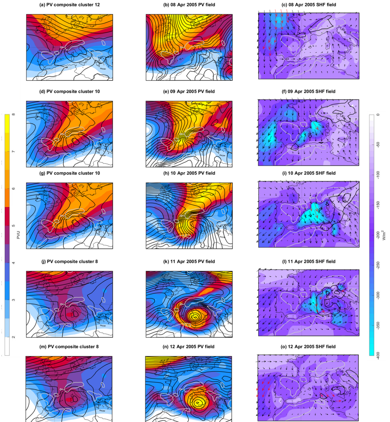
Figure 11. As in Fig. 10 but for a CWB event identified by the transition 10 → 8.
