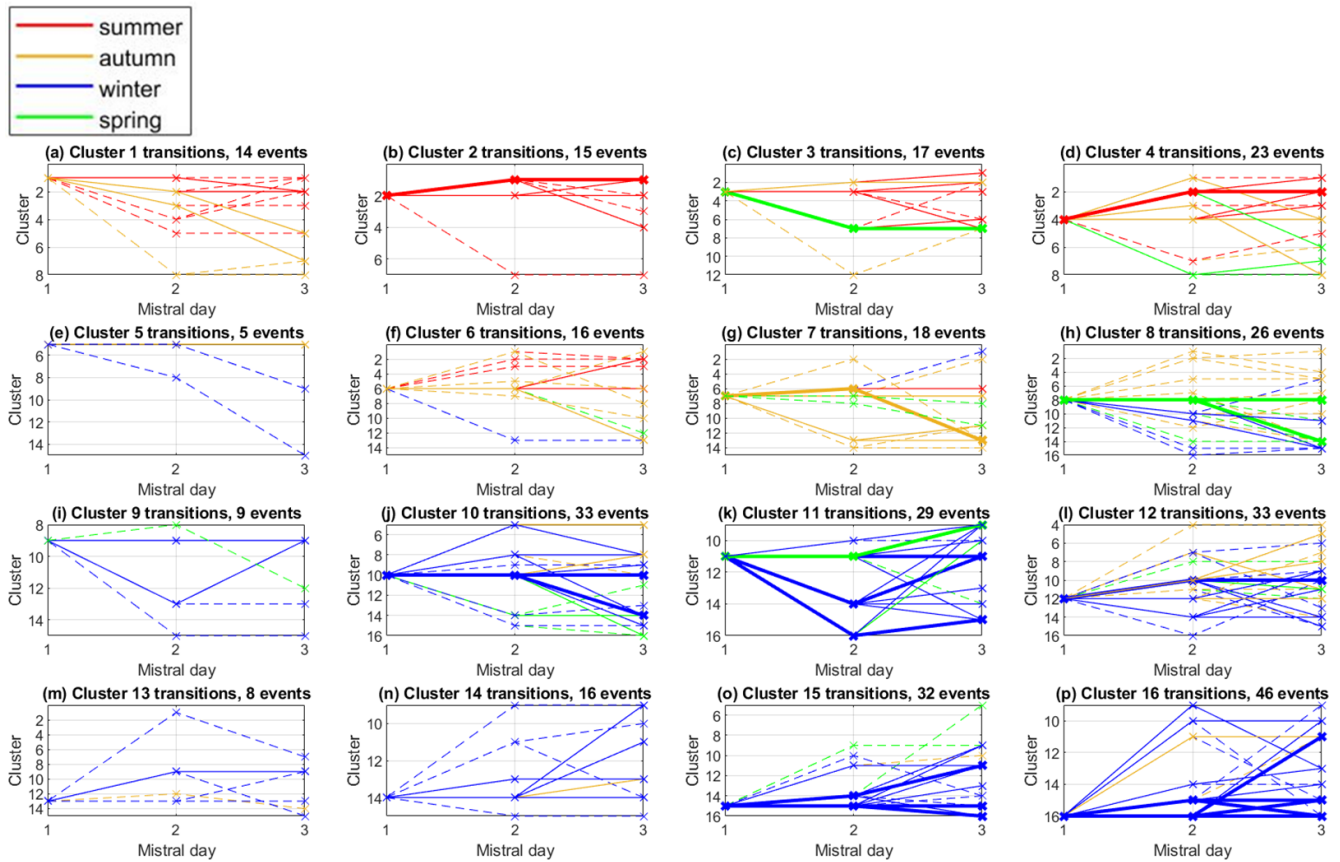
Figure 9. Transition sequences (days 1–3) for mistral events initiating with each cluster at mistral day 1 and lasting at least 3 d, at every season (using the same 2- and 4-month seasonal definitions as in Fig. 8). The x axis represents days passed from mistral initiation. Solid lines indicate transition sequences (days 1–3) that repeat 2–4 times throughout the time period. Thick lines emphasize sequences occurring 5–10 times, while dashed lines denote single-occurrence sequences.
