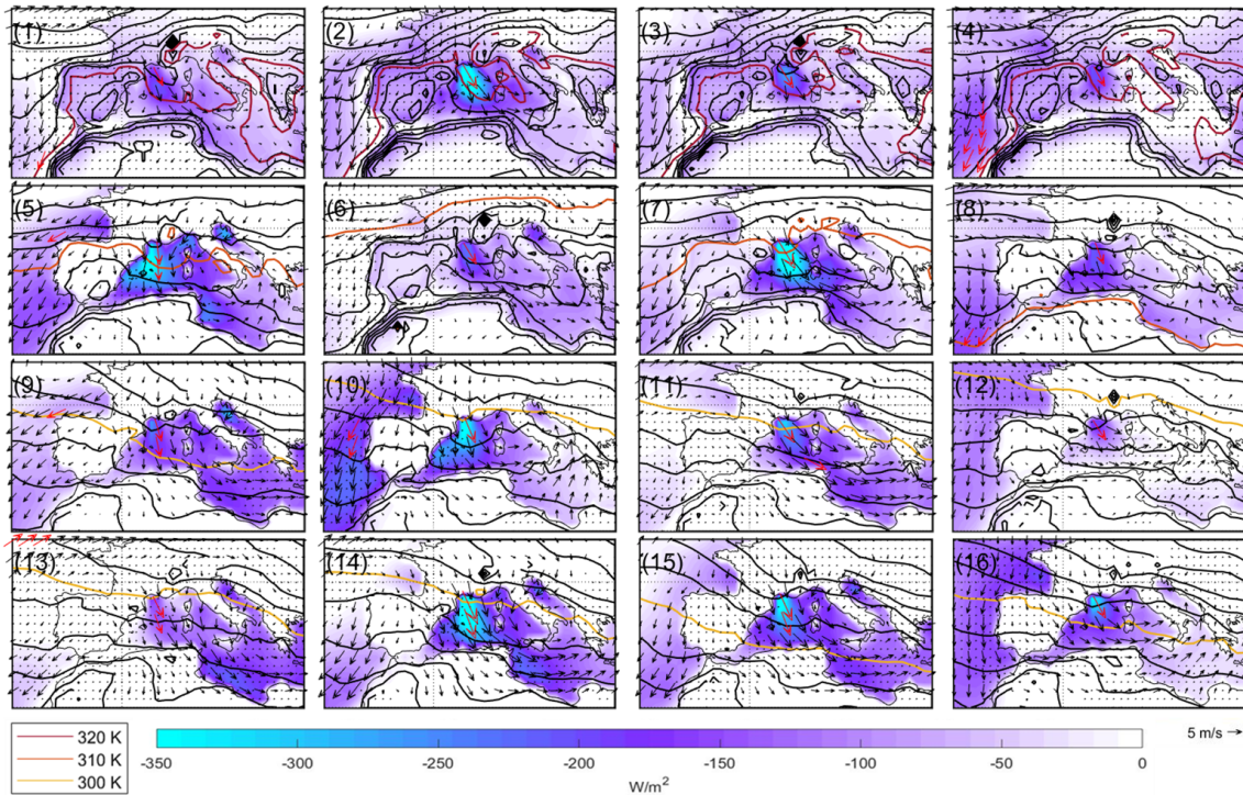
Figure 6. The same as Fig. 5 but for surface heat fluxes (sum of sensible and latent, W/m^2 ) in color; equivalent potential temperature at the 900 hPa level in black contours at 2 K intervals; and the 300, 310 and 320 K isotherms in color (see legend). Black arrows denote 10 m wind vectors, where red arrows mark winds above the local 75th percentile. Dotted regions indicate statistical significance > 95 % for the surface heat flux composites compared to the average mistral flow.
