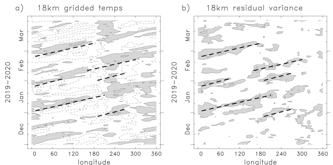
Figure 3. (a) Longitude-time diagram of gridded temperature anomalies over the equator ( 8^\circ\text{N} – \text{S} ) at 18 km (contours of \pm 1.5, 4.5 K) highlighting eastward traveling Kelvin waves. (b) Residual temperature variance over 8^\circ\text{N} – \text{S} at 18 km, with contour interval of 4 \text{ K}^2 . The thick dashed lines in (b) follow some of the residual variance maxima, and these are duplicated in (a) to show relation to the gridded temperatures. The small tick marks on the time axes denote 10-day intervals.
