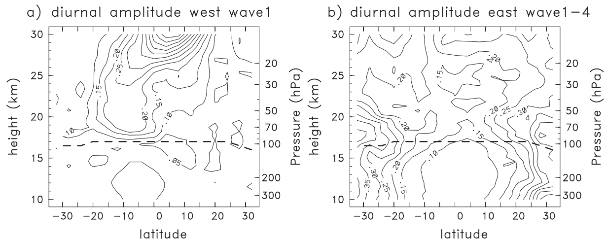
Figure 7. Meridional cross sections of rms amplitude for (a) migrating diurnal tide DW1, and (b) non-migrating diurnal tide DE1/4 (discussed in text). Contour interval is 0.05 (K). The dark dashed line is the thermal tropopause.
