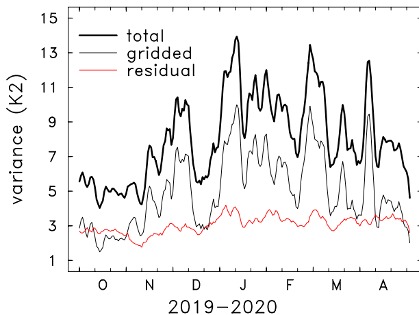
Figure 2. Time series of zonal temperature variance ( K^2 ) at 18 km over 8^\circ\text{N} – \text{S} , calculated from the full C2 measurements (total), from the gridded fields and the residual (difference between the total and gridded results).
