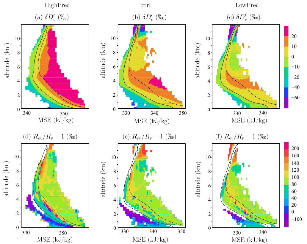
Figure 6. (b,e) As for Figure 5 but for (a) \delta D_v anomaly with respect to the domain-mean at each vertical level, (d) (\phi - 1) \cdot 1,000 , where \phi = R_{ev}/R_v ; it is expressed in ‰. (a,d) As for (b,e) but for HighPrec. (c,f) As for (b,e) but for LowPrec.
