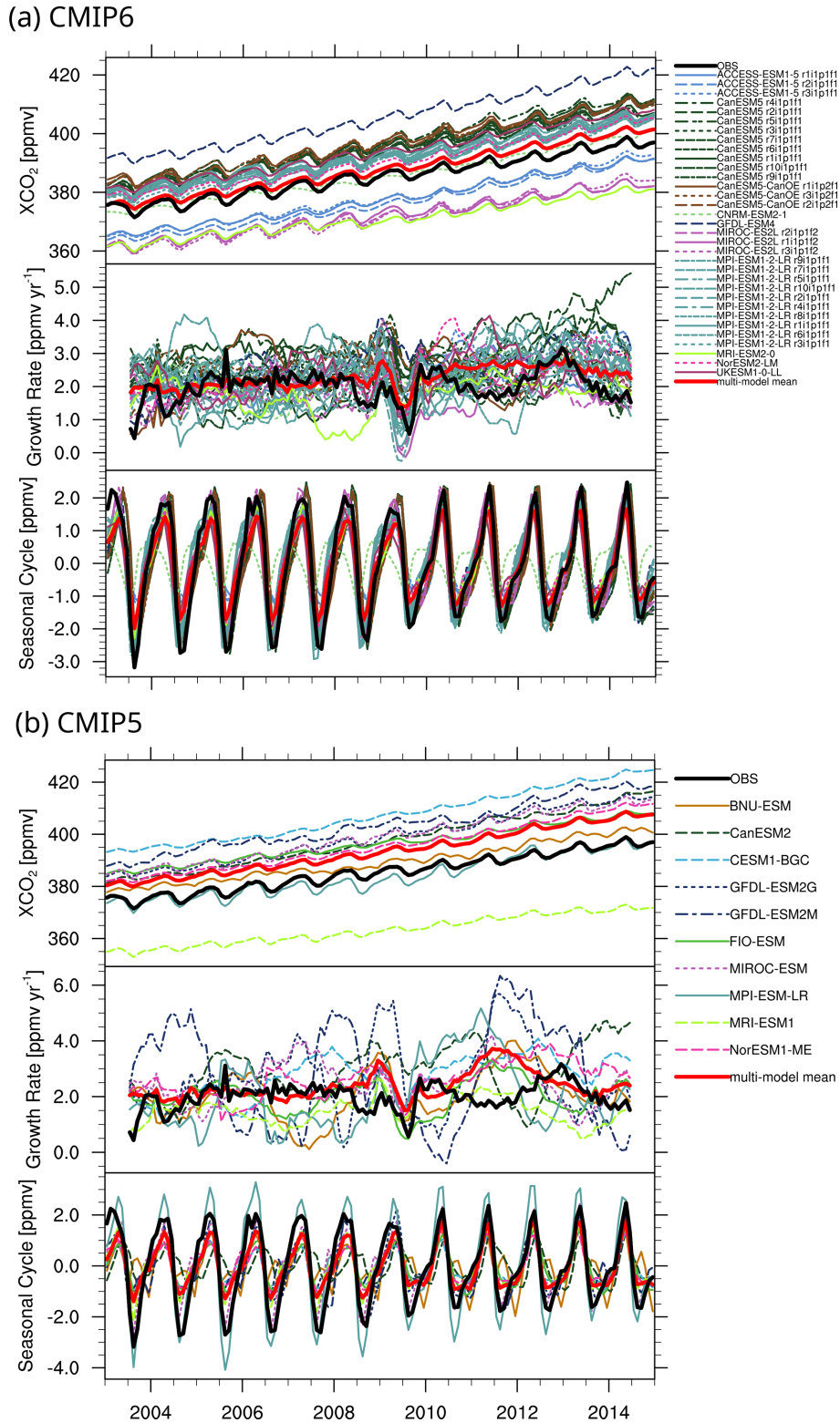
Figure 3. (a) Global time series of monthly mean column-averaged carbon dioxide ( XCO_2 ) from 2003 to 2014 for the emission-driven CMIP6 model simulations in comparison to satellite XCO_2 data (bold black line). The model output is sampled as the satellite data. The top panels show the time series, while the middle panels show the computed monthly growth rate, which has been used to detrend the data to obtain the seasonal cycle shown in the bottom panel. All available ensemble members for each model are shown to demonstrate the intrinsic variability of the models. (b) Same as Fig. 3a but for CMIP5. Only one ensemble member is shown.
