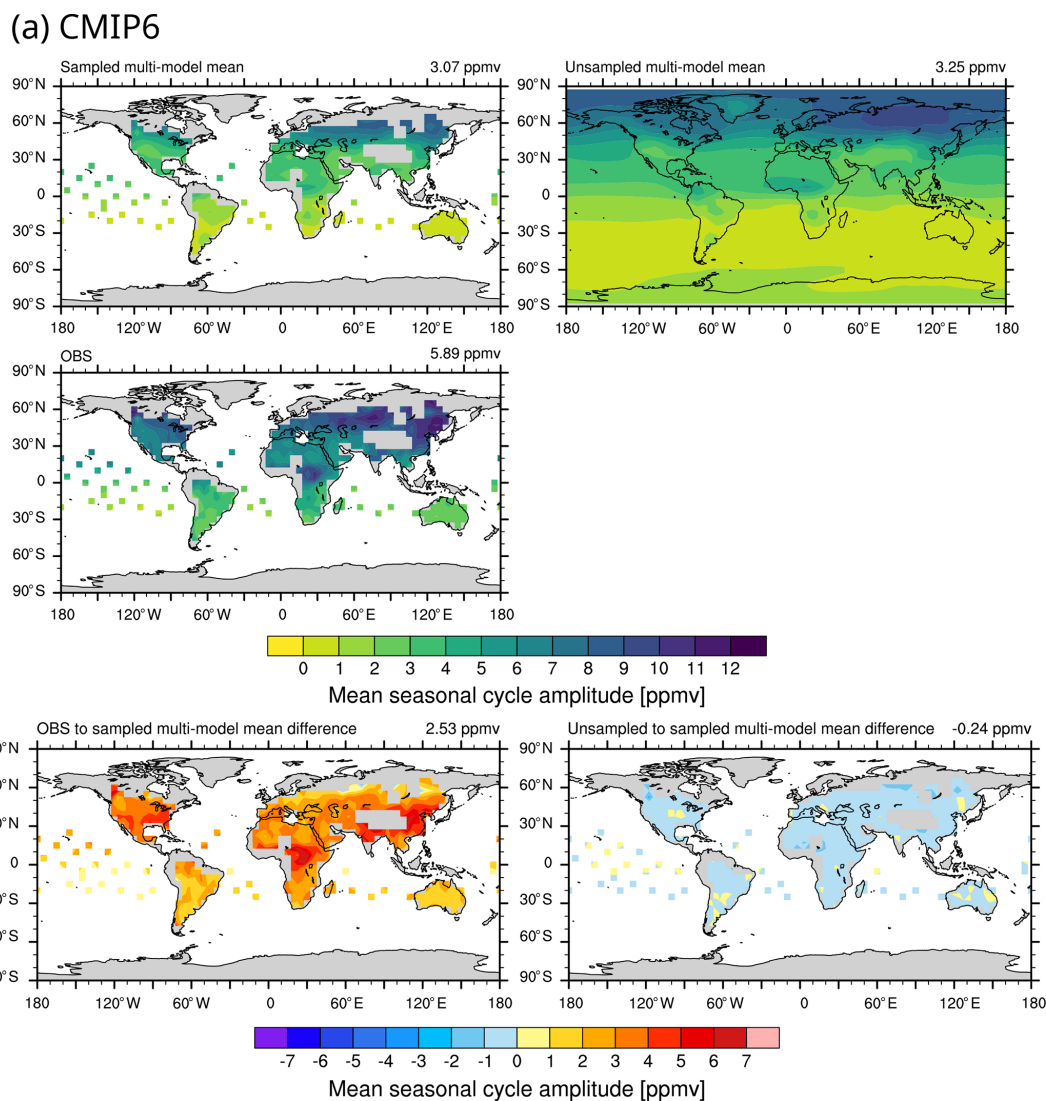
Figure 6. (a) Maps of mean SCA of the CMIP6 multi-model mean for 2003–2014. Top: SCA of multi-model mean with observational sampling (left) and without sampling (right). Middle: SCA of the satellite observations. Bottom: difference between observations and sampled model data (left) and sampled and unsampled model (right).
