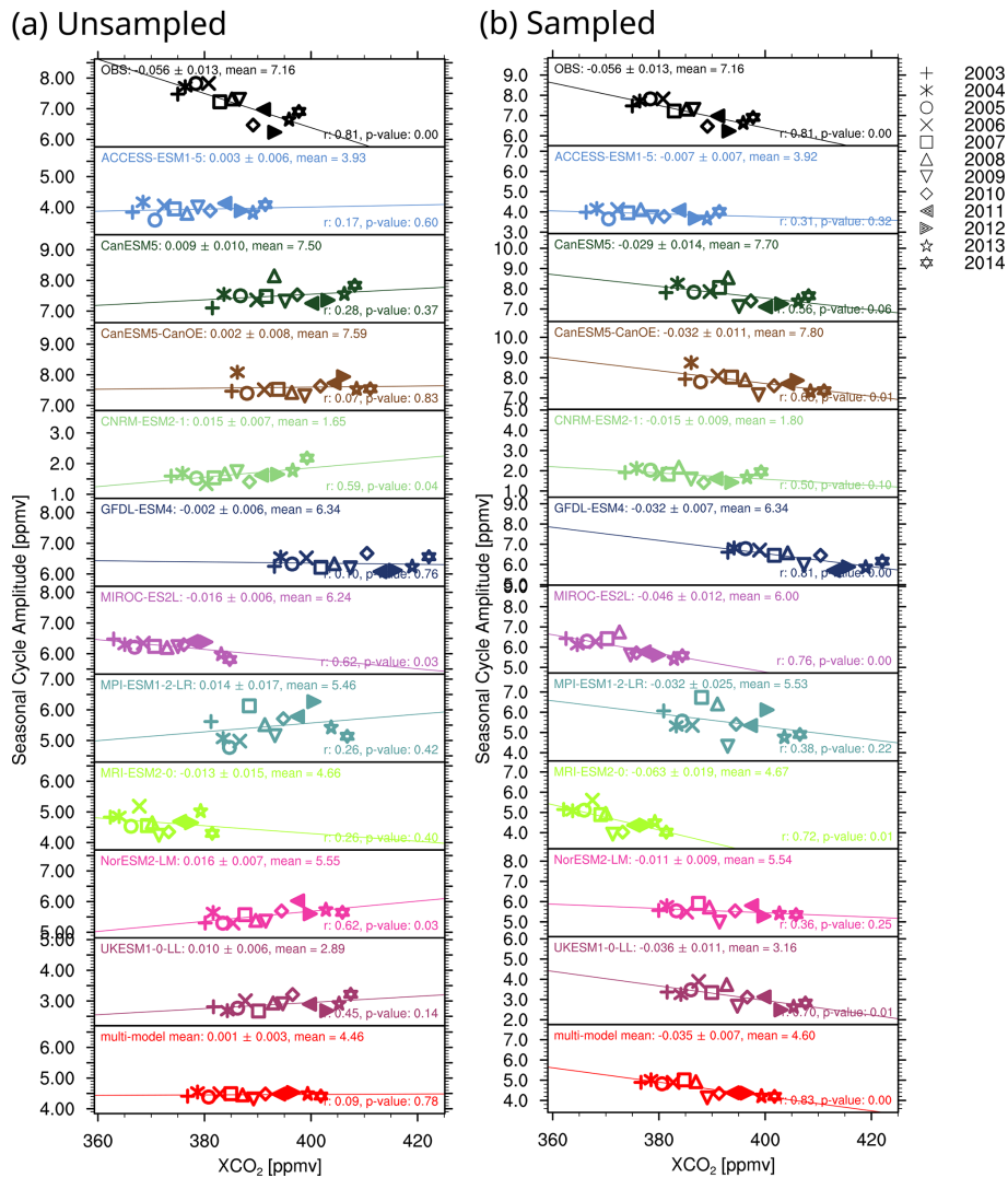
Figure 7. Trend of SCA with XCO 2 for 2003–2014 for the northern midlatitudes (30–60° N), including a linear regression with slope and mean SCA given in the top left of each panel and the Pearson correlation coefficient as well as the p value in the bottom right. Symbols denote the different years and model colors are consistent with previous figures. The left panels (a) show unsampled CMIP6 models, while CMIP6 models sampled according to the satellite data are shown on the right (b). Note that the y-axis range for each plot is the same and only differs by a shift.
