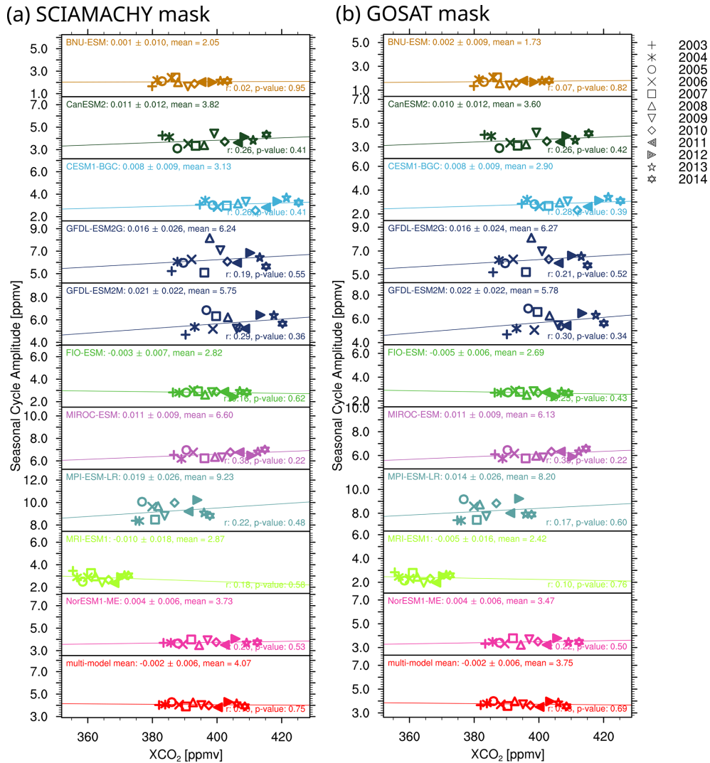
Figure B2. Same as Fig. B1 but with CMIP5 models masked using (a) the SCIAMACHY mask and (b) the GOSAT mask, with the masks derived from Fig. 8, masking out points with less than 50 % coverage in those time periods.
