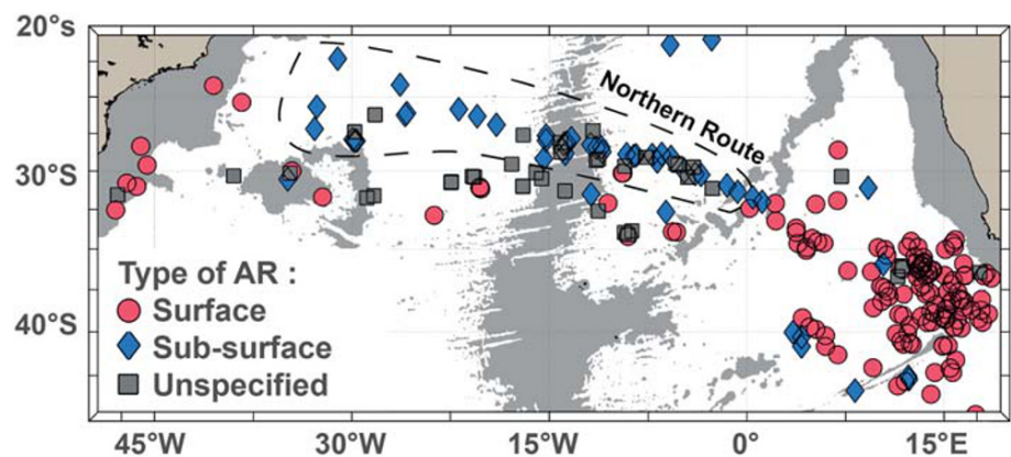
Figure 5. Type of anticyclonic eddies (surface-, subsurface-intensified, and unspecified) for Agulhas rings identified in the region. Only Argo profiles sampling inside an anticyclone at a distance of less than half of its instantaneous R_{Vmax} are considered. The northern route is indicated by a dashed contours, and the southern route considered in the text corresponds to the profiles in the South Atlantic Ocean south of the northern one. The gray shading in each panel represents water depths of less than 3,500 m in the ETOPO1 data set (Amante & Eakins, 2009).
