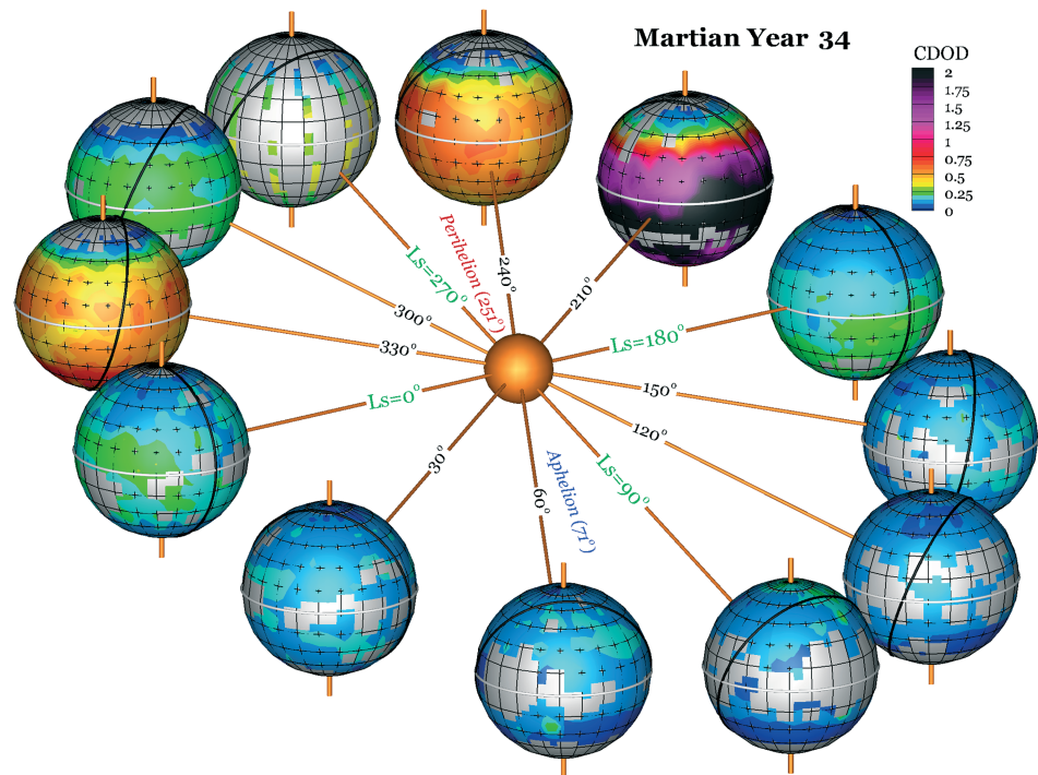
Figure 2. Global distributions of column dust optical depth at the wavelength of 9.3\ \mu\text{m} during Martian Year 34. The dust opacity has been scaled to the atmospheric pressure of 610 Pa. Gray areas indicate missing data. The planetary rotational axis is shown in yellow, and the equatorial and terminator circles are superposed as thick white and black curves, respectively. While the sizes of the solar and Martian bodies are not scaled in comparison with the distances between them, the planetary orientations and orbital positions are based on calculations using NAIF-SPICE. Note that the color scale is different from Figure 1.
