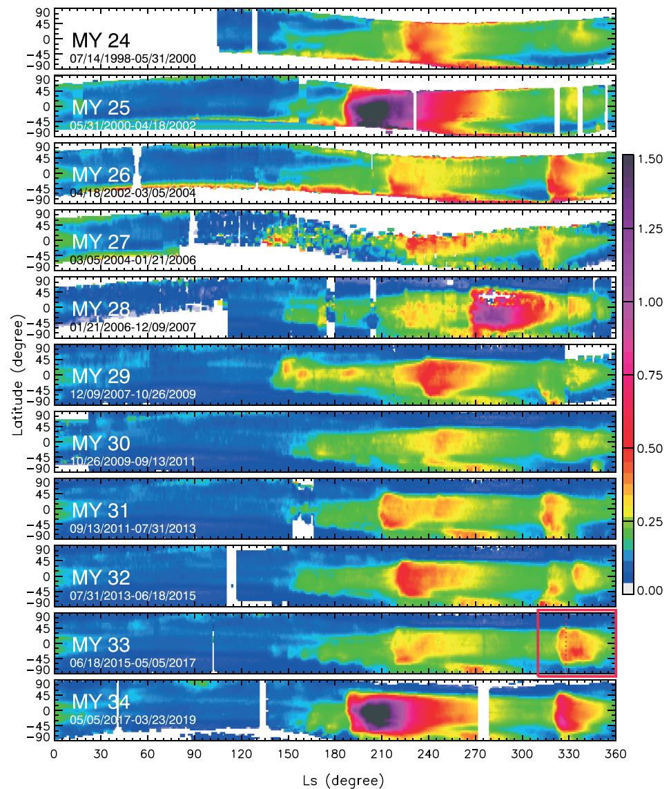
Figure 1. Mars zonally averaged column dust optical depth at the infrared wavelength of about 9.3\ \mu\text{m} during 11 Martian years. The dust opacity, scaled to the atmospheric pressure level of 610 Pa, is shown as a function of solar longitude ( L_s ) and geographic latitude. The start and end dates on Earth are given for each Martian year, and white areas indicate missing data. The red box in the second to the last panel denotes the currently investigated 2017 regional dust storm period, and the vertical dashed line indicates the time when a dusty condition is taken for this study. Note that while MY 24–33 zonal means are created using the Mars Climate Database gridded dust climatology versions 2.0 and 2.1, MY 34 zonal mean is created using an updated version (as described in Montabone et al., 2020). Therefore, caution is required when directly comparing MY 34 and the other years (particularly MYs 28–33).
