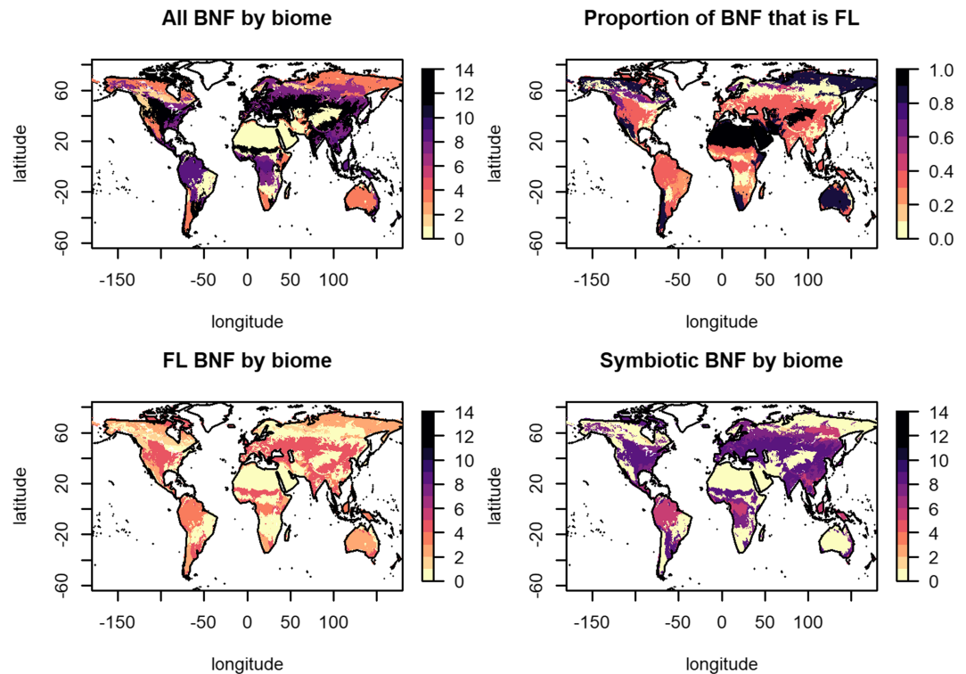
Figure 6. Maps of BNF using median BNF allocated to IGBP land cover types. (top) Symbiotic (S) and free-living (FL-ud) BNF combined (left) and relative proportion of free-living (FL-ud) BNF (right). (bottom) Free-living (FL-ud) BNF (left) and Symbiotic (S) BNF (right). BNF in \text{kg ha}^{-1} \text{year}^{-1} . The proportion of free-living BNF is 0 (all symbiotic) to 1 (all free living).
