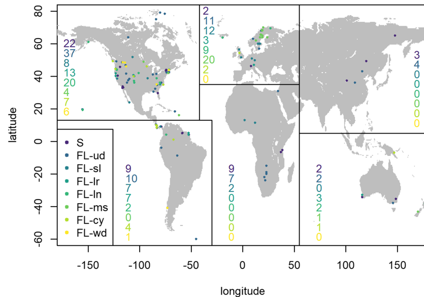
Figure 1. All the data locations mapped, with the color indicating the type of BNF. Since some regions have multiple measurements associated, less values are shown than are used in other parts of the analysis, as they are overplotted. The numbers shown in the map relate to the number of values within each category found within the delineated region.
