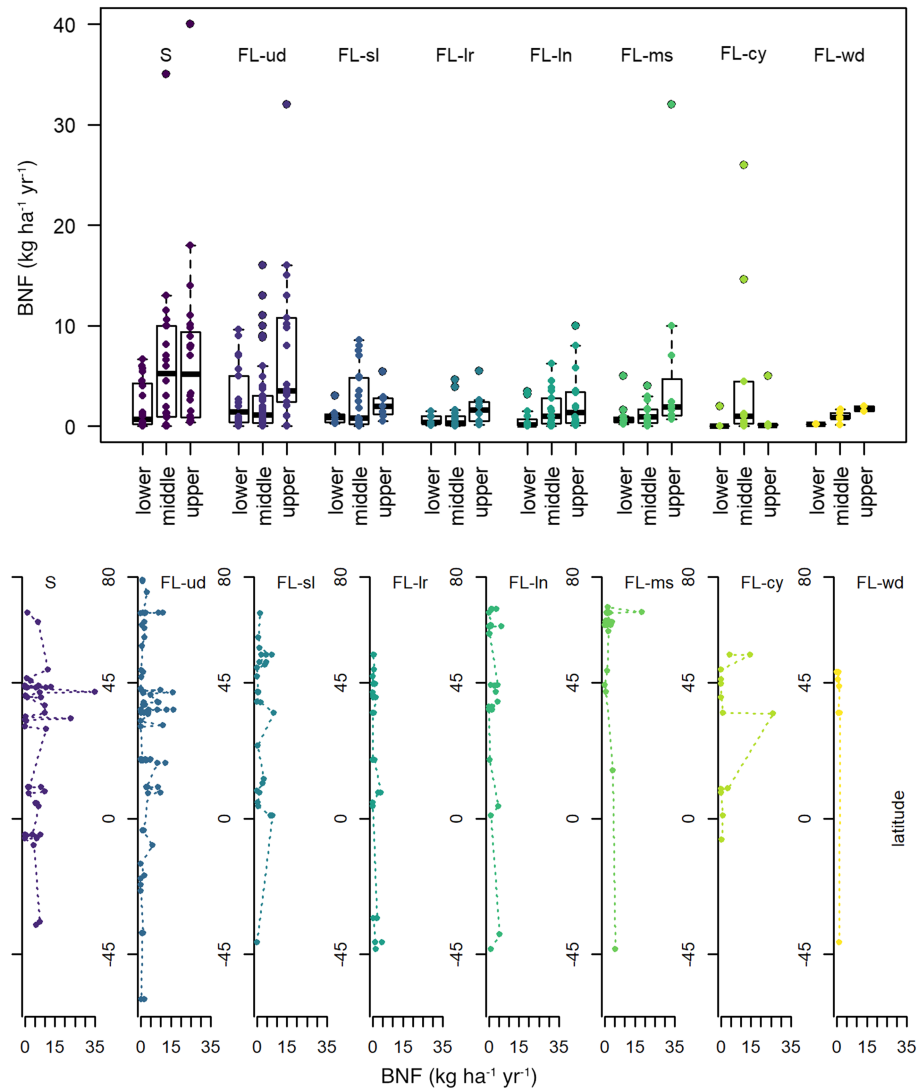
Figure 2. (a) Fixation values for each of the BNF types, grouped by lower and upper bounded ranges or a single central value (note a measurement is either represented as a range or as a single value but not both). For each boxplot, the midline is the median, the upper line third quartile, lower line the first quartile, and the whiskers extend up to 1.5 times the interquartile range from the top of the box to the furthest datum within that distance. Datum beyond 1.5 times the interquartile range are represented as individual points. Overlaid on the boxplots are all the individual points as a “beeswarm” scatter. (b) BNF values by latitude and separated by type. These are the central values as described in the methods, that is, the mean of a range or the single most representative value. BNF units for all cases are kg ha -1 year -1 .
