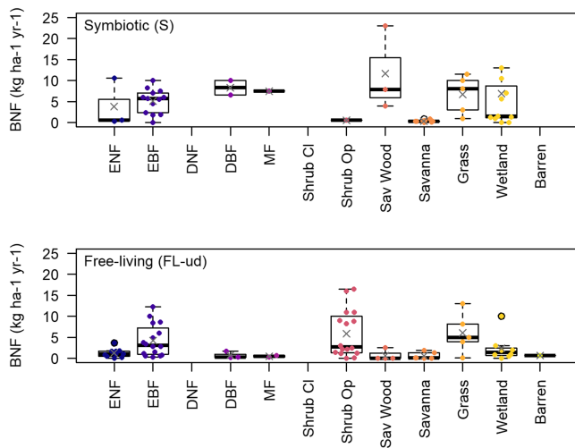
Figure 7. The symbiotic (S) and free-living (FL-ud) values categorized by biome type. For each boxplot, the midline is the median, the upper line third quartile, lower line the first quartile, and the whiskers extend up to 1.5 times the interquartile range from the top of the box to the furthest datum within that distance. Datum beyond 1.5 times the interquartile range are represented as individual points. Overlaid on the boxplots are all the individual points as a “beeswarm” scatter. The grey x on each set of data represents the arithmetic mean.
