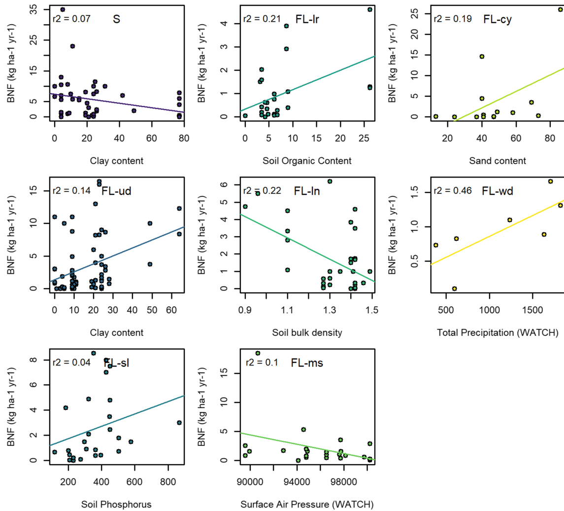
Figure 4. The strongest relationship (highest r^2 ) between each of the BNF types and the climate or soil variables listed in methods. The linear fit is shown as a line in each of the plots and the corresponding r^2 value is in the top left-hand corner. SOC ( \text{kg m}^{-2} ), ET ( \text{mm day}^{-1} ), precipitation ( \text{mm year}^{-1} ), clay or sand content (percent), and surface pressure (Pa).
