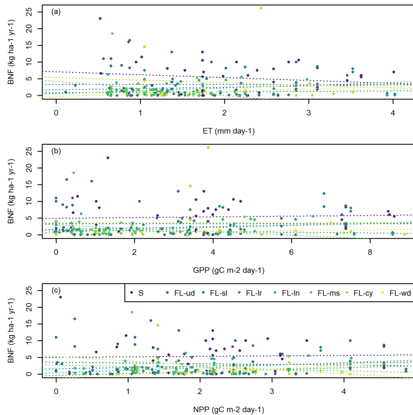
Figure 3. BNF plotted against (a) ET ( \text{mm day}^{-1} ), (b) GPP ( \text{gC m}^{-2} \text{day}^{-1} ), and (c) NPP ( \text{gC m}^{-2} \text{day}^{-1} ), color coded by BNF type (Table 2). Dotted lines represent the linear fit of the BNF type of the same color.
