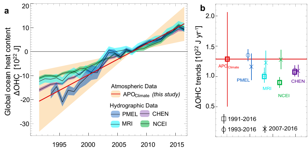
Figure 1. Change in global ocean heat content ( \Delta\text{OHC} ). (a) \Delta\text{OHC} derived from hydrographic and atmospheric observations (normalized to zero in 2007, \pm 1-\sigma uncertainty). (b) Linear least-squares trends for 1991–2016, 1993–2016 and 2007–2016 ( \pm 1-\sigma uncertainty). Hydrography-based \Delta\text{OHC} estimates combine warming rates at ocean depths of 0 to 2,000 m warming rates (Cheng and co-authors (CHEN) 8 , Pacific Marine Environmental Laboratory (PMEL) 6 , Meteorological Research Institute (MRI) 5 and National Center for Environmental Information (NCEI) 47 with revised deep ocean (depth of more than 2000 m) of ref. 7 (Tables S1, S2). The atmospheric-based estimate which uses observed atmospheric potential oxygen trends ( \Delta\text{APO}_{\text{Climate}} ) and model-based \Delta\text{APO}_{\text{Climate}} -to- \Delta\text{OHC} ratio, does not resolve interannual variations.
