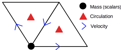
Figure 3. Lozenge: basic computational element containing one node (for mass and other scalars), three edges (for velocities) and two triangles (for circulation). Separate wavelet transforms are provided for the nodes (scalar valued) and edges (vector valued). The adaptive grid consists of the significant nodes and edges, together with nearest neighbours in position and scale necessary for dynamics.
