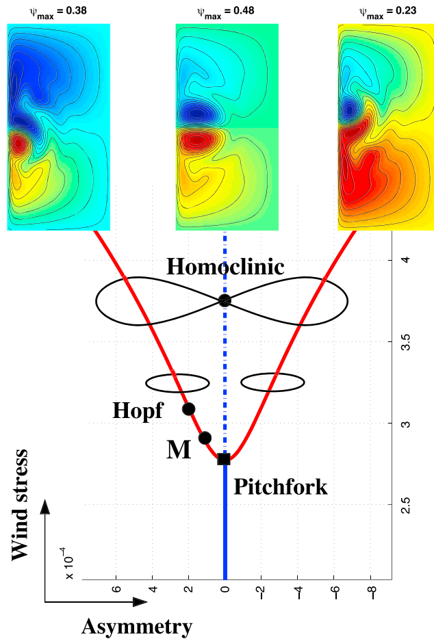
Figure 2. Generic bifurcation diagram for the barotropic quasi-geostrophic model of the double-gyre problem: the asymmetry of the solution is plotted versus the intensity of the wind stress \tau . The stream function field \psi = \psi(x, y) is plotted for a steady-state solution associated with each of the three branches; positive values in red and negative ones in blue. After Simonnet et al. (2005).
