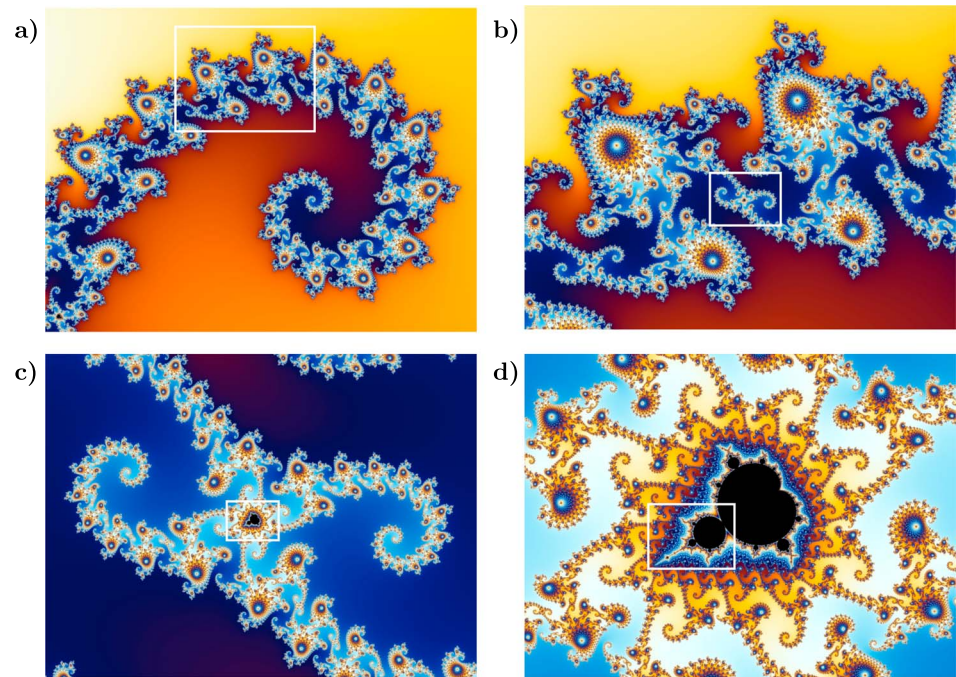
Figure 4. Mandelbrot set, with c_r on the abscissa and c_i on the ordinate. The white rectangles indicate the domain of the zoom in the next panel. Created by Wolfgang Beyer with the program Ultra Fractal 3 ( https://commons.wikimedia.org/wiki/File:Mandel_zoom_00_to_01.png ); Steps 4–8 of the iteration are reproduced here as panels (a)–(d) of the figure, under the Creative Commons Attribution-Share Alike licence ( https://creativecommons.org/licenses/by-sa/2.5/deed.en ).
