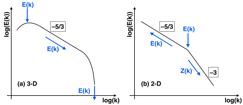
Figure 5. Energy and enstrophy cascades in (a) three-dimensional (3-D) and (b) two-dimensional (2-D) turbulence. The latter panel also characterizes the dual cascades in quasi-geostrophic turbulence. Courtesy of Niklas Boers.
