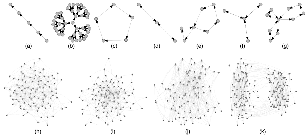
Figure 7. Schematic diagram of the network classes studied by Colon and Ghil (2017). Simple network motifs: (a) linear networks; (b) trees; (c) isolated loops; (d and e) two interacting loops, connected through a pivotal node; (f and g) three interacting loops. More complex classes of directed graphs, with n = 100 nodes and connectivity c = 4 : (h) directed Erdős-Rényi (ER) networks; (i) scale-free networks with the specific, production-network distribution of in- and out-degree based on the Fujiwara and Aoyama (2010) data set; (j) random acyclic networks in which production moves upward; and (k) a network of two interdependent RA networks—in the network at left, production moves upward, while it moves downward in the one at right. Reproduced from Colon and Ghil (2017). Economic networks: heterogeneity-induced vulnerability and loss of synchronization, Chaos , 27, 126703, doi: 10.1063/1.5017851, with the permission of AIP Publishing.
