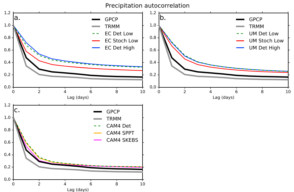
Figure 4. The mean autocorrelation between 10°S–10°N of daily mean precipitation averaged over 2.5° × 2.5° grid boxes in the satellite and model data sets. (a–c) Data for each family of model configurations along with TRMM and GPCP data. Most of the stochastic physics schemes reduce the autocorrelation, the exception being SPPT in CAM4, and this is very likely to be an improvement in EC-Earth (EC) and the UM.
