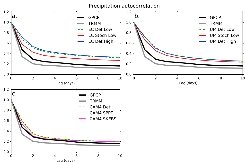
Figure 4. The mean autocorrelation between 10°S–10°N of daily mean precipitation averaged over 2.5^\circ \times 2.5^\circ grid boxes in the satellite and model data sets. (a–c) Data for each family of model configurations along with TRMM and GPCP data. Most of the stochastic physics schemes reduce the autocorrelation, the exception being SPPT in CAM4, and this is very likely to be an improvement in EC-Earth (EC) and the UM.
