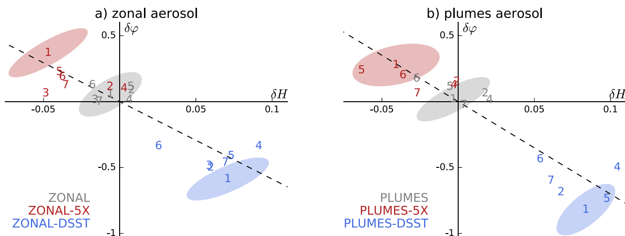
Figure 10. ITCZ shift \delta\varphi (y axis; units of deg lat) as a function of the change in cross-equatorial energy transport \delta H (x axis; units of PW) in simulations with (a) the zonal aerosol and (b) the plumes aerosol. The dashed lines are linear regressions through all models and simulations; the slope is -(5.9 \pm 0.6) deg lat/PW for the zonal aerosol and -(7.0 \pm 0.7) deg lat/PW for the plumes aerosol. This indicates that the ratio between ITCZ shift and energy transport is insensitive to the spatial distribution of the aerosol. The numbers correspond to the model numbers in Table 3. The shaded ellipses indicate the internal variability estimated by the ECHAM6 model (model 1).
