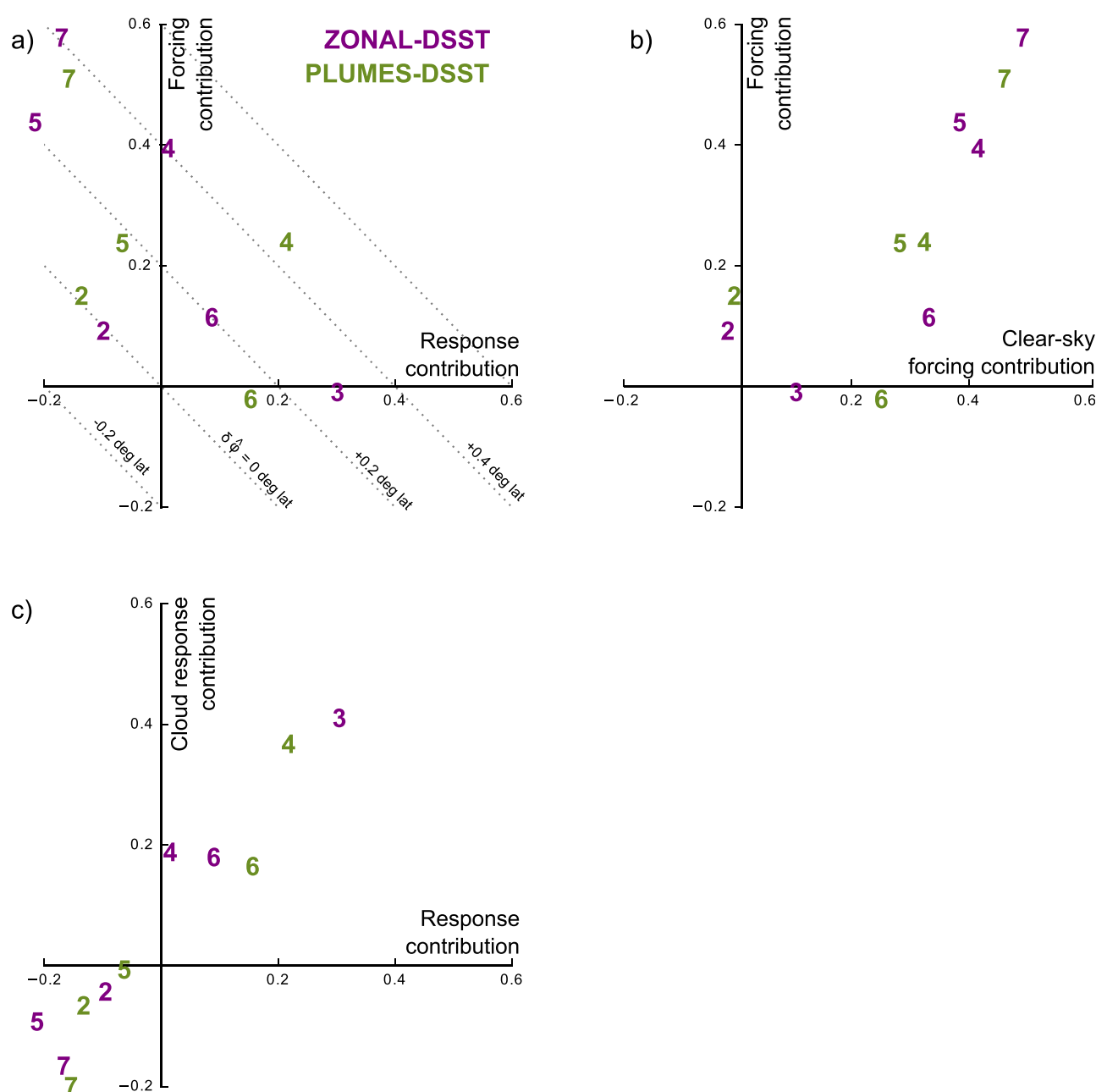
Figure 14. Estimate of the additional ITCZ shift \delta\hat{\phi} that would occur if models were coupled to an interactive-SST surface. The additional ITCZ shift is expressed relative to the ECHAM6 model (model 1), which is thus not included in the plot. (a) The magnitude of \delta\hat{\phi} can be read from the slanted dashed lines. \delta\hat{\phi} is decomposed into a contribution from model differences in top-of-atmosphere aerosol radiative forcing (y axis) and a contribution from model differences in the TOA response (x axis). (b) The contribution from model differences in aerosol forcing versus model differences in clear-sky aerosol forcing. (c) The contribution from model differences in the TOA response versus model differences in the change of cloud-radiative effects. All energetic quantities are converted into ITCZ shift units (deg latitude) using the scaling of 6.5 deg lat/PW from Figure 10.
