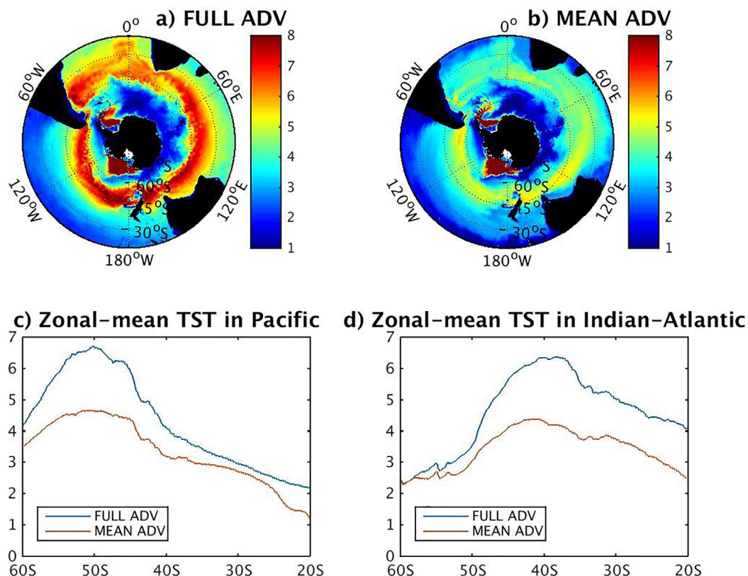
Figure 10. TST inventory (vertically integrated and divided by 5500 m), in years, averaged over the last 6 months of year 30: (a) FULL_ADV; (b) MEAN_ADV. Bottom row: same fields (in years) but zonally averaged within: (c) the Pacific; and (d) the Atlantic-Indian basins.
