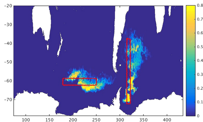
Figure 1. Evolution of the dye tracer; the initial (red lines) and concentrations at Day 196 are shown in the top layer for the online case.
