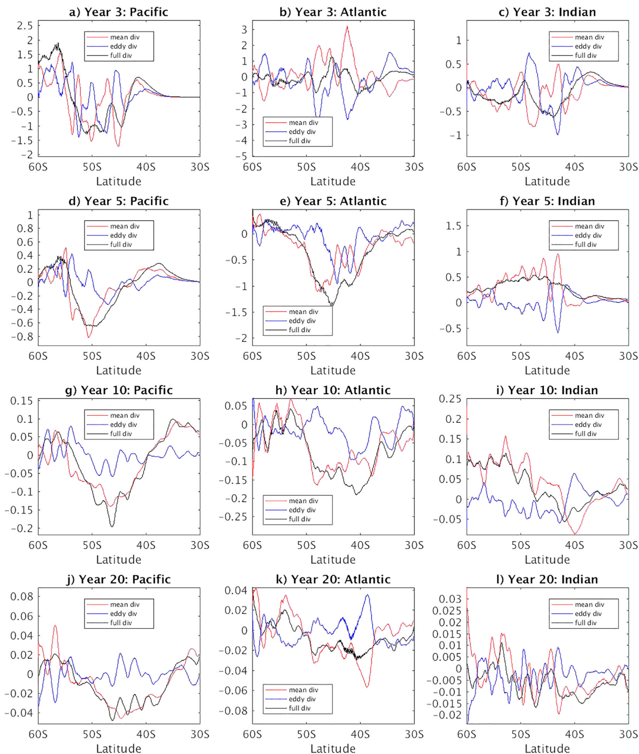
Figure 5. Divergence of BIR fluxes due to the mean currents (“mean advection” in equation (3), red lines) and mesoscale eddy currents (“eddy advection” in equation (3) blue lines), as well as their sum (black lines). Shown are the annual means of these terms for Years 3 (first row), 5 (second row), 10 (third row), and 20 (fourth row). These terms are vertically integrated within the top 25 layers, zonal averaged within the Pacific (left column), Atlantic (middle column), and Indian (right column) sectors and smoothed for presentation purposes. Units are 10^{10} \times \text{m s}^{-1} .
