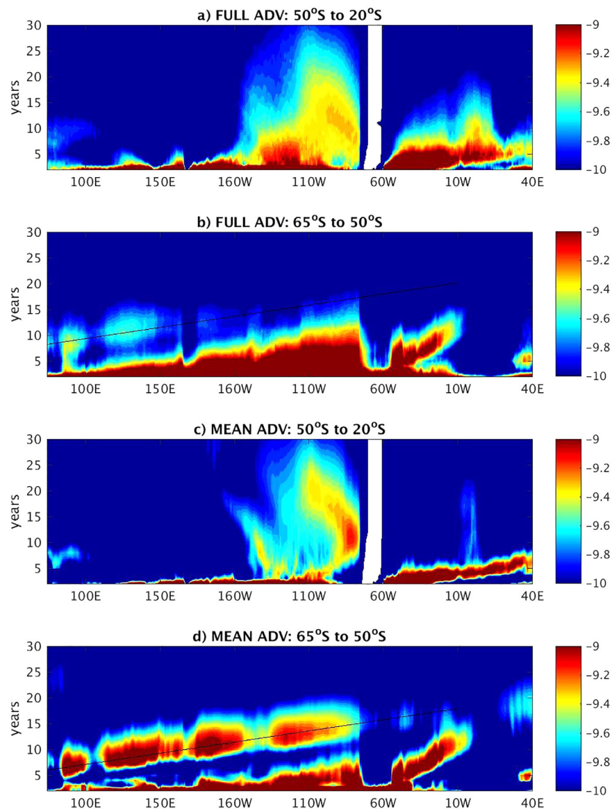
Figure 4. Hovmoller diagram of the zonal evolution of the BIR tracer. Logarithm of the meridionally averaged and vertically integrated tracer values are shown as the function of longitude and time in (a, b) FULL_ADV and (c, d) MEAN_ADV simulations. Figures 4a and 4c show values averaged within the 50°S to 20°S latitude range; Figures 4b and 4d, 65°S to 50°S range; the black line illustrates propagation with a constant speed of 0.05 \text{ m s}^{-1} .
