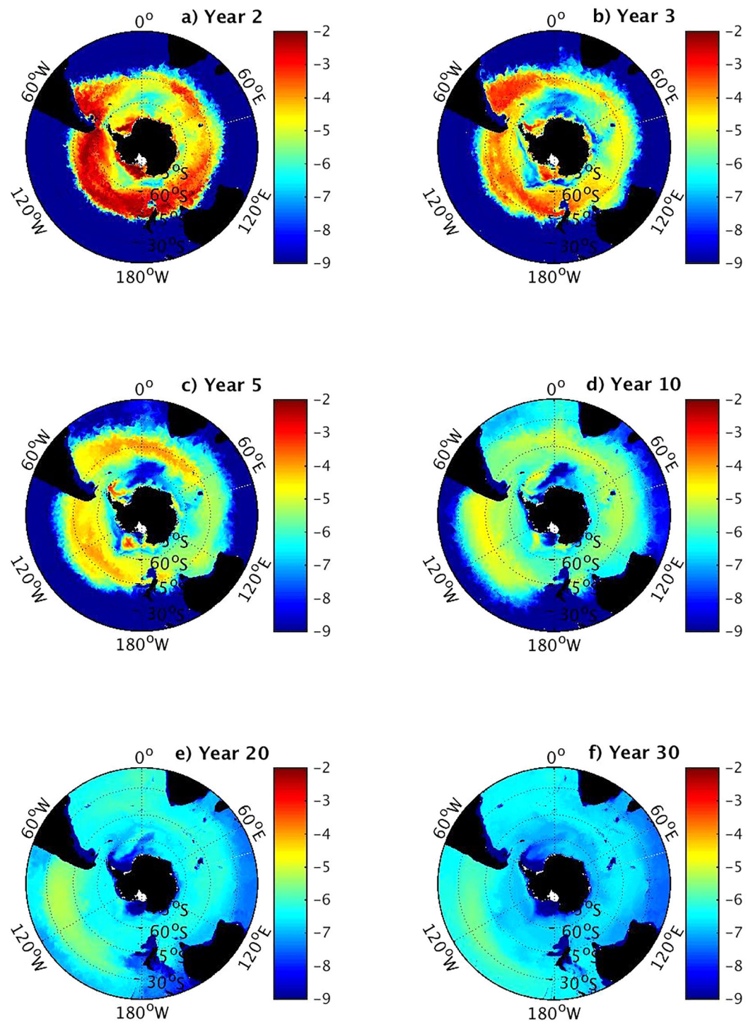
Figure 2. Horizontal spreading of the BIR tracer in the control (FULL_ADV) run. Logarithm of vertically integrated (over top model 25 layers) and divided by 5500 m BIR concentrations are shown for different times (Day 180 for each year). The depth of the 25th layer varies approximately between 1000 and 3500 m.
