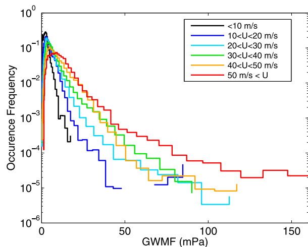
FIG. 7. As in Fig. 5 , but for the long-duration balloons of the Concordiasi campaign (Sep 2010–Jan 2011).
