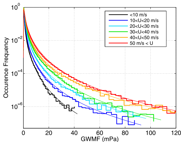
FIG. A2. PDFs of GWMF at a height of 18 km from the WRF simulations. Also shown are the lognormal distributions fitted to approximate their tails (thin lines), as described in the text.
