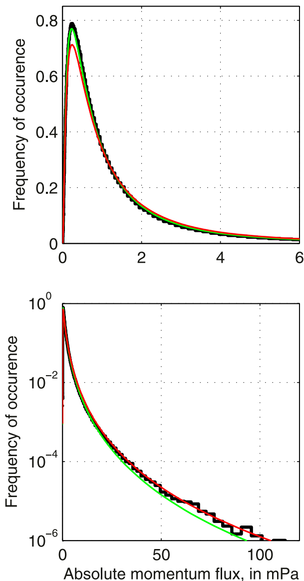
FIG. A1. Example of the fit using a lognormal for the PDF of momentum fluxes found over the ocean at z = 20 km in the WRF simulations for background winds larger than 50 \text{ m s}^{-1} . Three lines are shown: the thick black line is for the PDF estimated using 200 bins equally spaced for the logarithm of momentum fluxes, the thin green line depicts the lognormal PDF with the same median and geometric standard deviation, and the red line is the lognormal PDF optimized for the tail. (top) Standard plot of the PDF, showing the emphasis of values near zero (horizontal axis only extends to 6 mPa). (bottom) Semilog view of the complete distribution.
