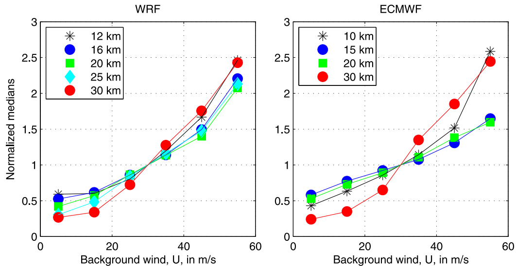
FIG. 10. Variation of the normalized median of GWMF with background wind speed U from (left) the WRF simulations and (right) the ECMWF analyses for different heights (see legends).
