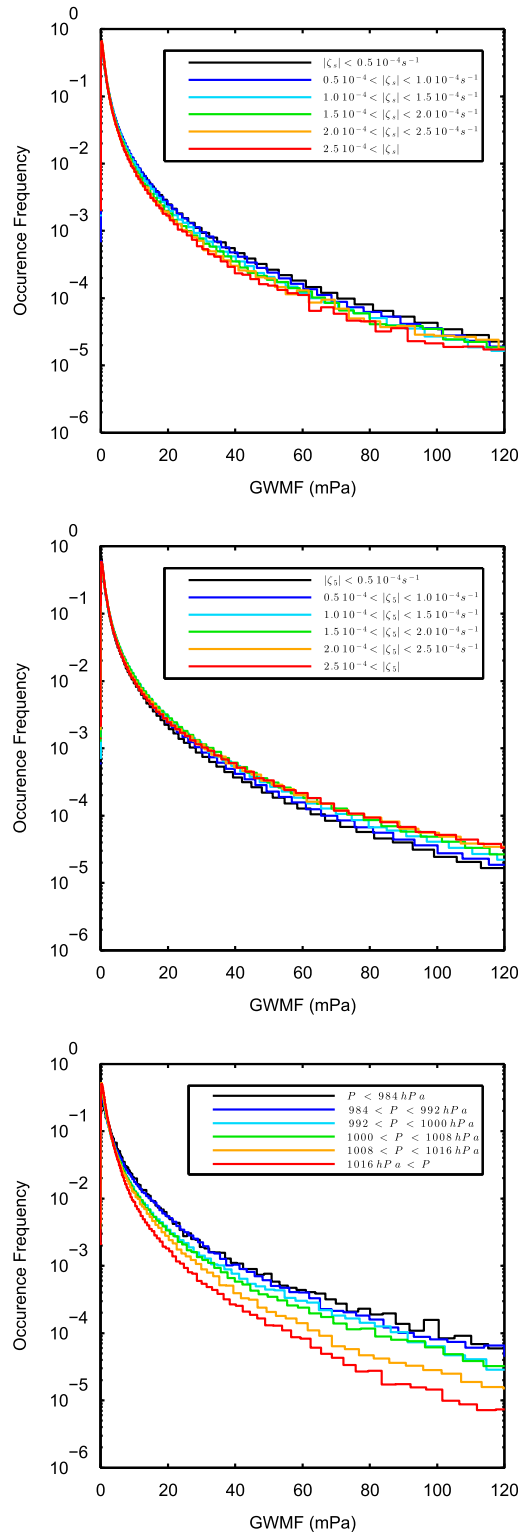
FIG. 13. PDFs of GWMF at z = 10 km, conditional on different indicators of tropospheric jet-front activity: (top) conditional on the absolute value of surface vorticity, by increments of 0.5 \times 10^{-4} \text{ s}^{-1} ; (middle) conditional on the absolute value of relative vorticity at z = 5 km, by increments of 0.5 \times 10^{-4} \text{ s}^{-1} ; and (bottom) conditional on surface pressure anomaly, by increments of 10 hPa.
