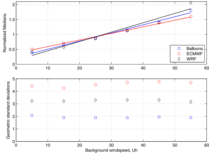
FIG. 8. Normalized medians of the PDFs of (top) GWMF and (bottom) geometric standard deviations as a function of the background wind speed. Black symbols correspond to the mesoscale simulations, red symbols to the ECMWF output, and blue symbols to the Concordiasi balloons. The medians were normalized by the means of the medians found for winds between 20 and 40 \text{ m s}^{-1} . For the medians, the linear regressions (thin lines) are also displayed.
