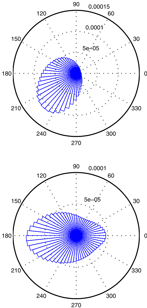
FIG. 12. PDF of the orientation of momentum fluxes relative to the local flow over the ocean from the WRF simulations at z = (bottom) 10 and (top) 20 km.
