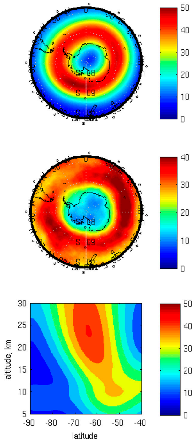
FIG. 3. Winds averaged from Sep to Dec 2010, from the analyses of the ECMWF. See Fig. 2 caption for panel details. Note that the color bars are adapted to each panel.
