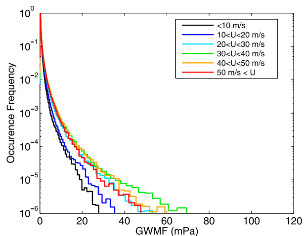
FIG. 11. PDFs of GWMF at 30 km in the WRF simulations, conditional on the wind speed at 10 km.
