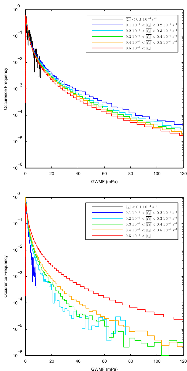
FIG. 14. PDFs of GWMF conditional on the absolute values of relative vorticity at (top) the surface and (bottom) the midtroposphere, averaged in boxes that are 10^\circ longitude by 5^\circ latitude.
