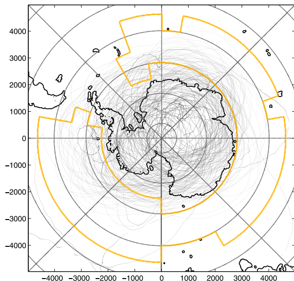
FIG. 4. Trajectories of the 19 Concordiasi balloons above Antarctica and the Southern Ocean (gray points, one every 12 h), along with the outline (thick orange line) of the nonorographic region used for the analysis of the three datasets [region 5 from Plougonven et al. (2013)].
