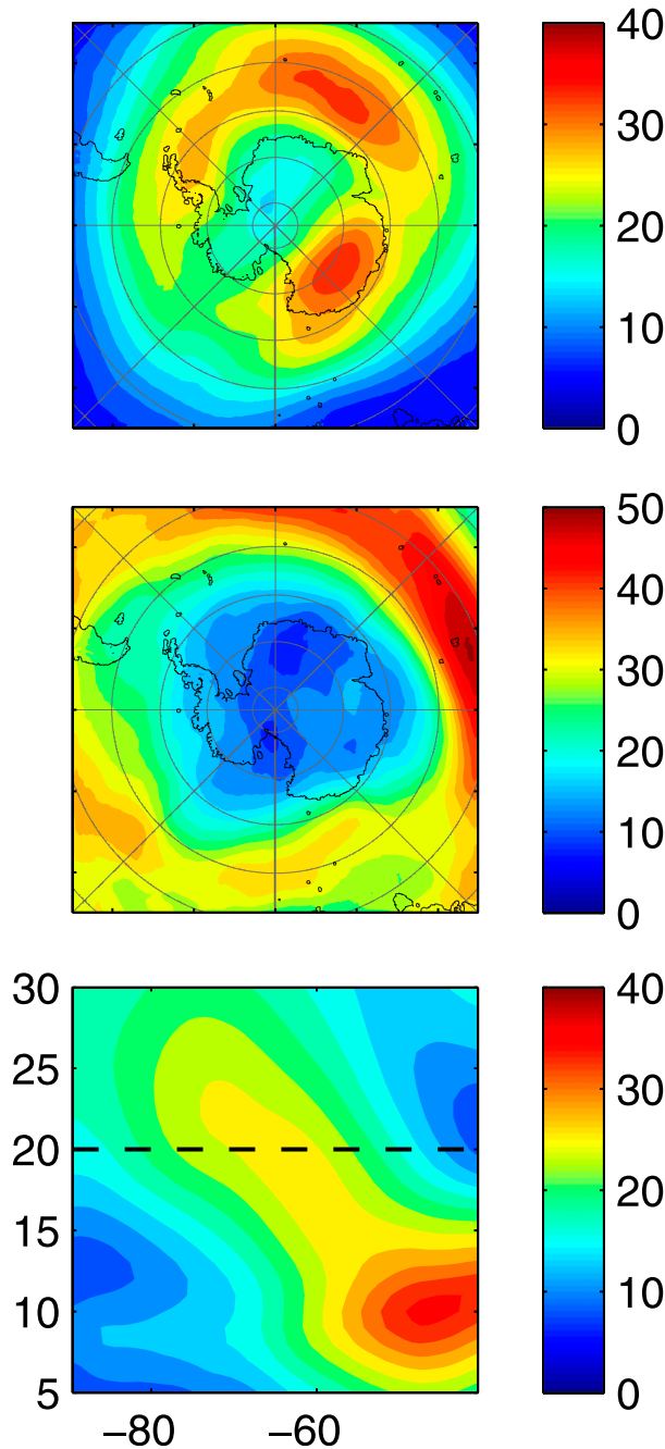
FIG. 2. Winds averaged from 21 Oct to 18 Dec 2005 from the WRF simulations, described by horizontal maps at z = (top) 20 and (middle) 10 km, and (bottom) by a vertical cross section. The dashed line in (bottom) indicates the height at which most of the analyses are carried out. Note that the color bars are adapted to each panel.
