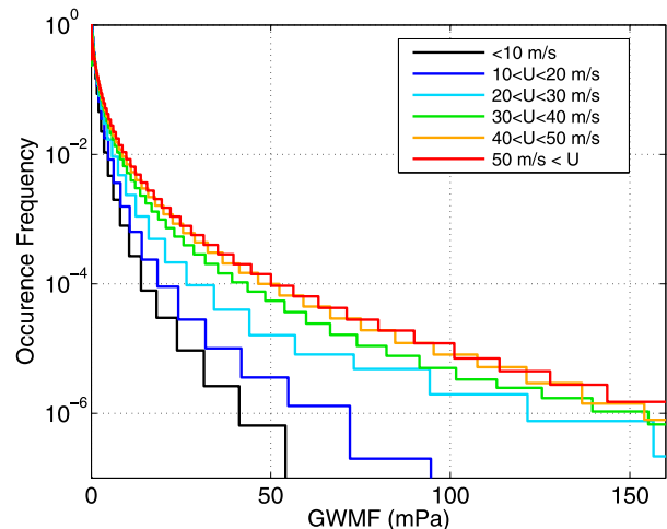
FIG. 6. As in Fig. 5 , but for the momentum fluxes calculated from the ECMWF analyses for the time of the Concordiasi campaign (Sep 2010–Jan 2011).
