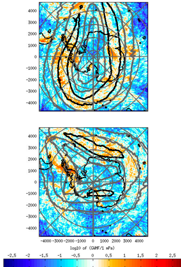
FIG. 1. Two examples of snapshots of absolute momentum fluxes (colors, logarithmic scale) and wind speed (thick gray lines for isotachs of 20 and 40 \text{m s}^{-1} , thick black line for 60 \text{m s}^{-1} ) at an altitude of z = 20 km from the mesoscale simulations of the flow above Antarctica and the Southern Ocean (Plougonven et al. 2013). The dates are (top) 1800 UTC 23 Oct and (bottom) 1200 UTC 7 Nov 2005.
