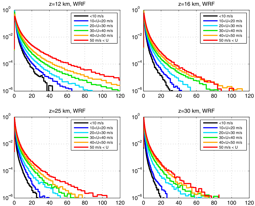
FIG. 9. PDFs of momentum fluxes conditional on the background wind speed at four different heights in the WRF simulations: z = (top left) 12, (top right) 16, (bottom left) 25, and (bottom right) 30 km.
