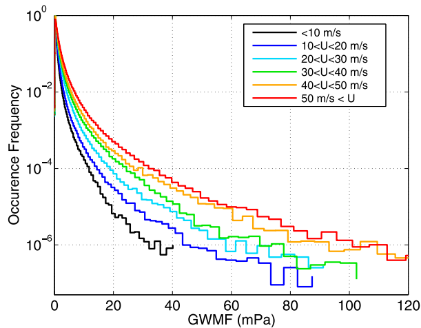
FIG. 5. Probability density functions of the GWMF (mPa) from the WRF simulations, at z = 20 km, conditional on the background wind.
