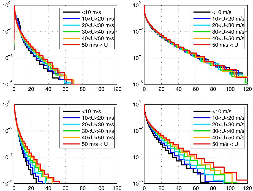
FIG. 15. PDFs of the parameterized GWMF, using the parameterization of the LMDZ atmospheric general circulation model. The scheme is used offline for the period from Sep 2010 to Jan 2011. (left) Results for the parameterization used with the source varying with the tropospheric flow [see de la Cámara and Lott (2015) for details]. (right) Results using a source that retains a lognormal distribution, but with the amplitudes independent of the tropospheric flow. The standard deviations for the phase speeds are (top) 40 and (bottom) 10 \text{ m s}^{-1} .
