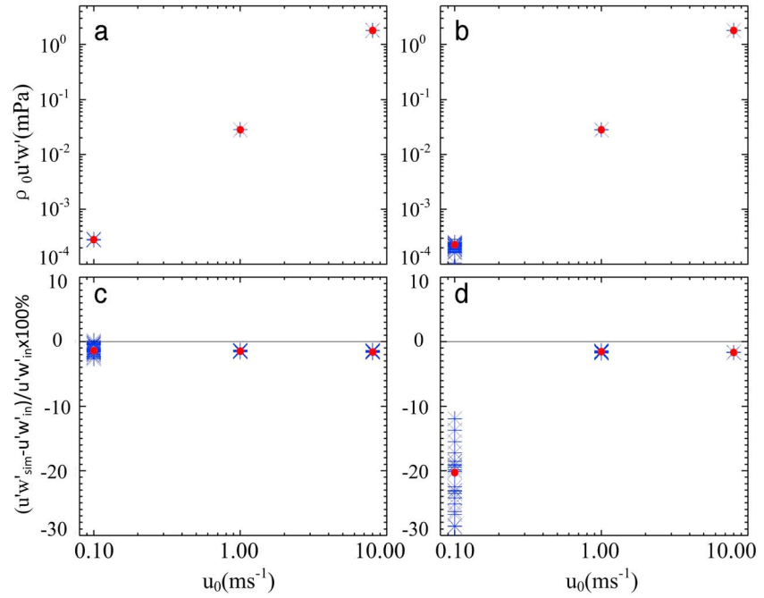
Figure 9. (a) Values of momentum flux in mPa plotted as a function of wave packet amplitude, u_0 . The blue star symbols represent the retrieved momentum flux with PPPAR noise added ( 0.005 \text{ ms}^{-1} in horizontal velocities) and the red symbols show the retrieved values without noise. (b) Similar to Figure 9a but with higher noise ( 0.025 \text{ ms}^{-1} in horizontal velocities) added. (c) The percentage of the difference between the retrieved and input values w.r.t. the input values for the low noise case (Figure 9a). (d) The percentage difference for the high noise case (Figure 9b).
