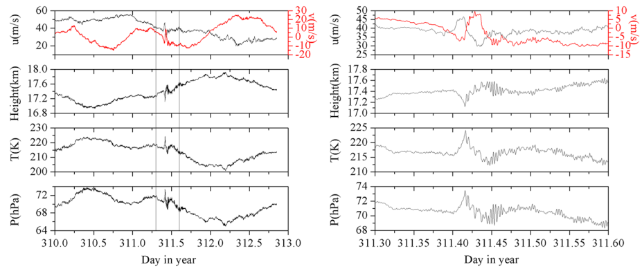
Figure 5. (left column) Time series for PSC19 from 6 November (DOY 310) to 8 November (DOY 312) 2010 and (right column) the zoomed time series during the period indicated by the two vertical black thin lines when the balloon passed over the Antarctic Peninsula. The time series from top to bottom show horizontal velocities, MSL (Mean Sea Level) altitude, air temperature, and air pressure (Lagrangian).
