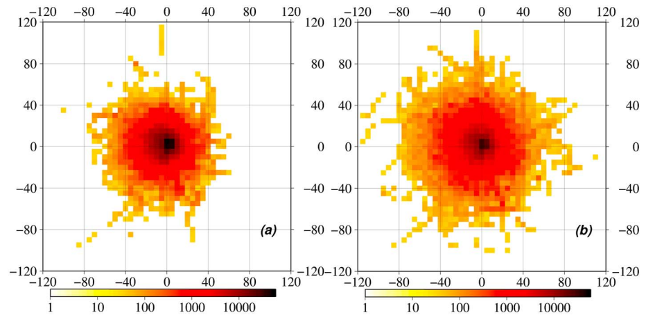
Figure 13. Distributions of gravity wave packet number density as a function of intrinsic phase speed derived from (a) PPPAR and (b) RTP solutions. Horizontal and vertical axes denote \hat{c}_x and \hat{c}_y in \text{ms}^{-1} , respectively. Color scales denote the number of wave packets.
