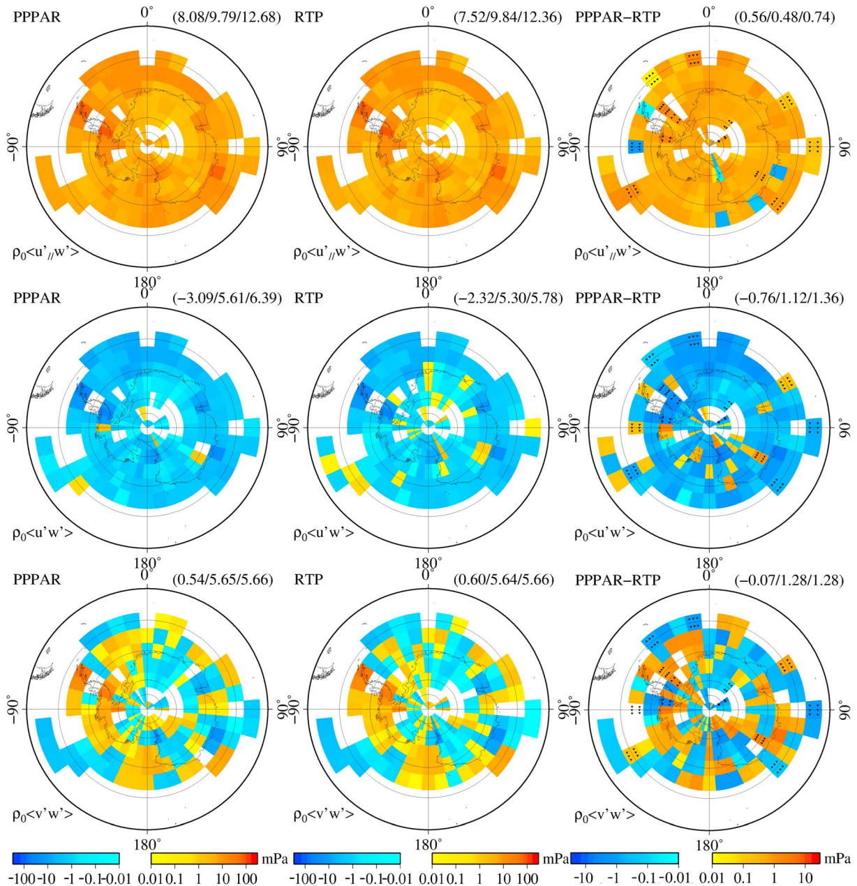
Figure 10. Comparison of the geographic distribution of density-weighted momentum fluxes derived from (left column) PPPAR and (middle column) RTP solutions and (right column) their difference (PPPAR-RTP). Absolute, zonal, and meridional momentum flux results are shown in Figures 9 (top row) to 9 (bottom row). The color scales have been divided by a factor of 10 for the right most column compared with the left two columns. Values given in the brackets at the top right of each panel are the mean value, the standard deviation and the RMS values in all bins, respectively. Bins in the right most columns filled with black dots denote statistical insignificance due to insufficient measurements.
