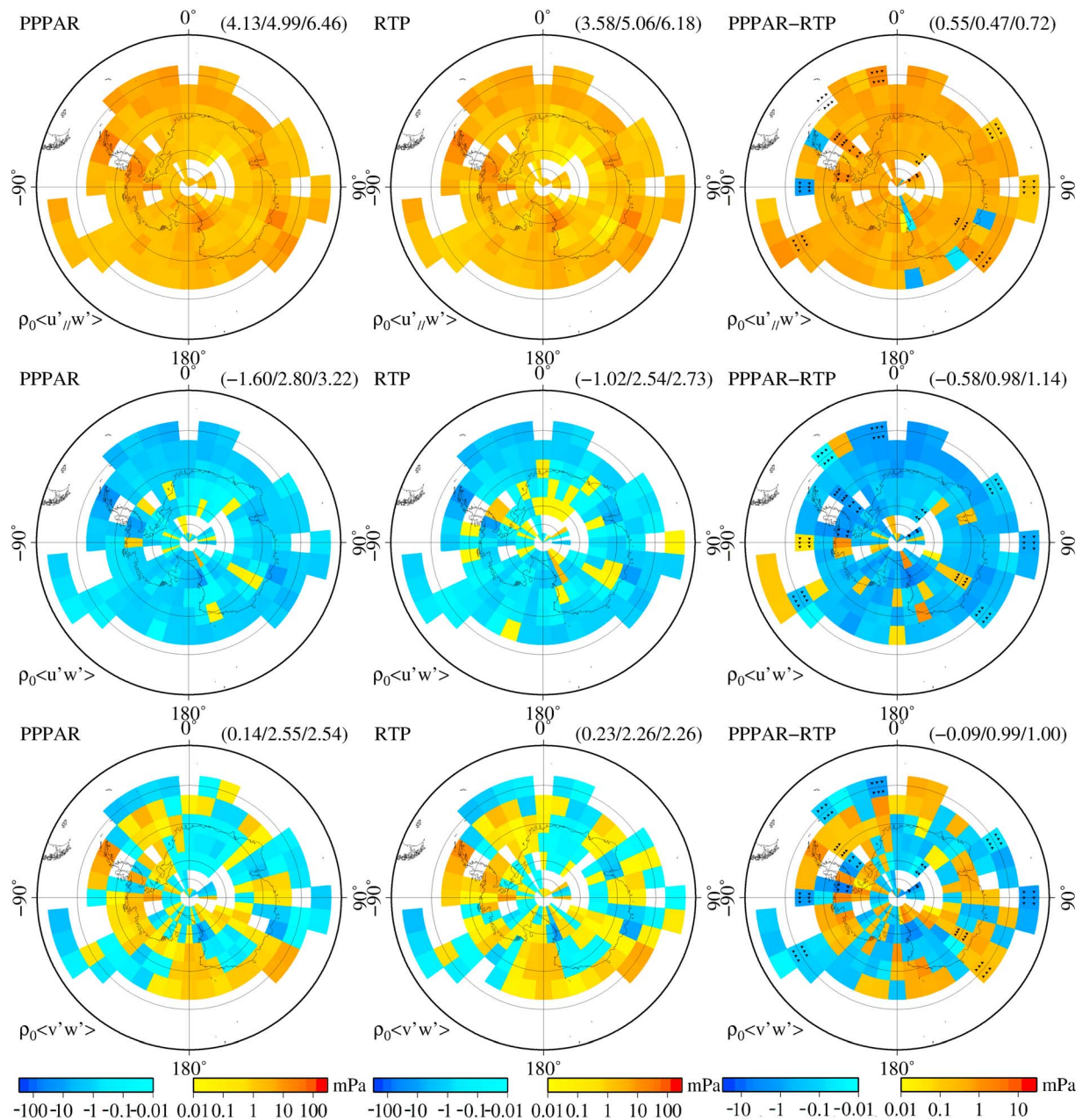
Figure 11. Comparison of the geographic distribution of density-weighted momentum fluxes for the high frequency portion of GWs (intrinsic period shorter than 1 h) derived from (left column) PPPAR and (middle column) RTP solutions and (right column) their difference (PPPAR-RTP). Absolute, zonal, and meridional momentum flux results are shown in Figures 11 (top row) to 11 (bottom row). The color scales have been divided by a factor of 10 for the right most column compared with the left two columns. Values given in the brackets at the top right of each panel are the mean value, the standard deviation and the RMS values in all bins, respectively. Bins in the right most columns filled with black dots denote statistical insignificance due to insufficient measurements.
