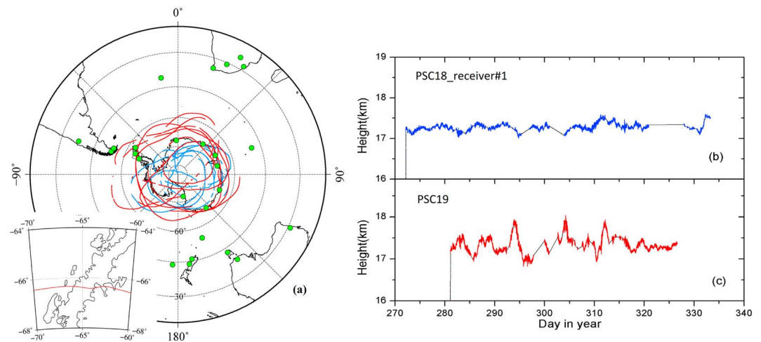
Figure 1. Ground-based GPS station distribution and balloon trajectories: (a) Green dots denote the ground-based GPS stations from the IGS network used for satellite clock and FCB estimation. The blue line and red line are the trajectories of GPS receiver #1 on PSC18 and the receiver on PSC19, respectively. The Antarctic Peninsula region is enlarged in the inset figure when PSC19 passes over the Antarctic Peninsula on 7 November 2010; (b) Altitude time series derived from the ROC GPS receiver #1 on PSC18 and (c) from the ROC GPS receiver on PSC19. Data gaps are indicated by straight lines.
