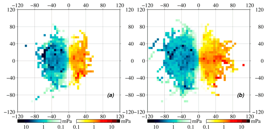
Figure 14. Distributions of zonal momentum fluxes as a function of intrinsic phase speed derived components \hat{c}_x and \hat{c}_y derived from (a) PPPAR and (b) RTP solutions. Negative momentum flux (westward propagation) is shown in blue, while the red scale denotes positive flux (eastward propagation).
