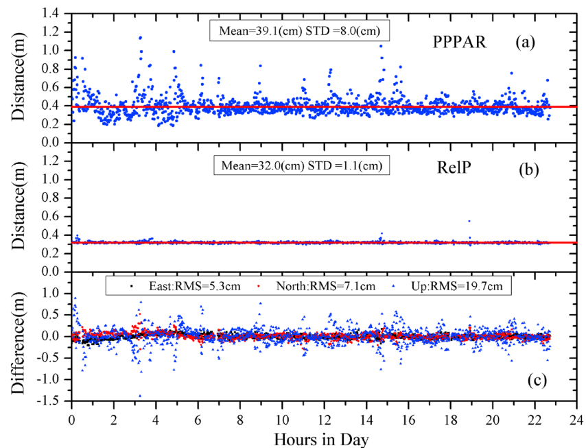
Figure 2. Comparison of PPPAR and RelP solutions: (a) Time series of the baseline distance between the two receivers on PSC18 derived from the PPPAR solutions. The mean value and standard deviation are given at the top of the panel and the mean value is also indicated with the red horizontal line; (b) similar to Figure 2a but derived from RelP solutions; (c) Differences of the baseline from PPPAR and RelP solutions in the east (black), north (red), and vertical (blue) components. The RMS values of the differences are also indicated at the top of the panel.
